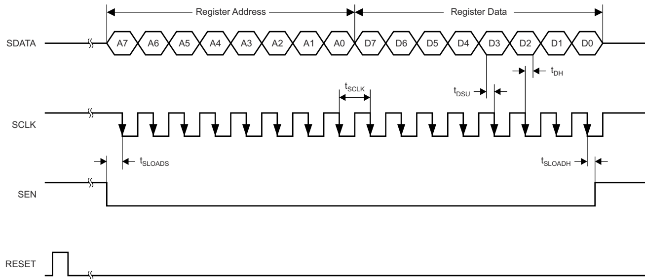
図 6-1. Serial Interface Timing
