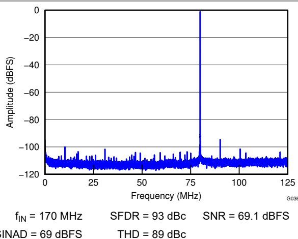
Figure 8-6. FFT (Default) at 170 MHz
