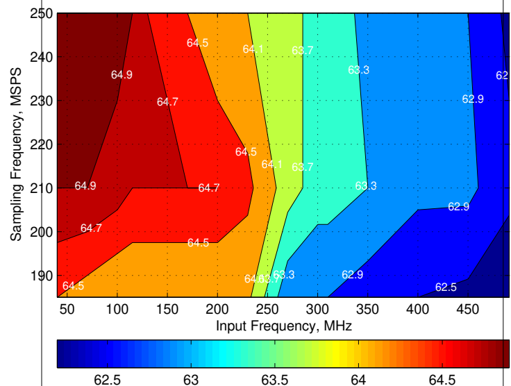
Figure 6-37. Signal-to-Noise Ratio (6-dB Gain)
