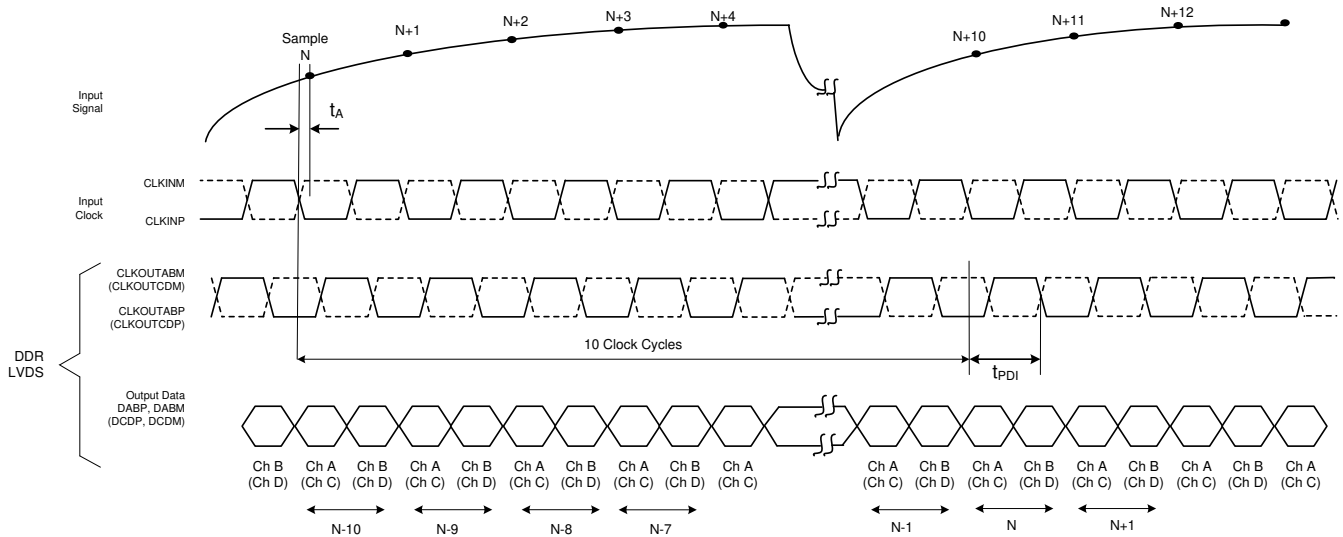
Figure 7-2. Latency Timing
