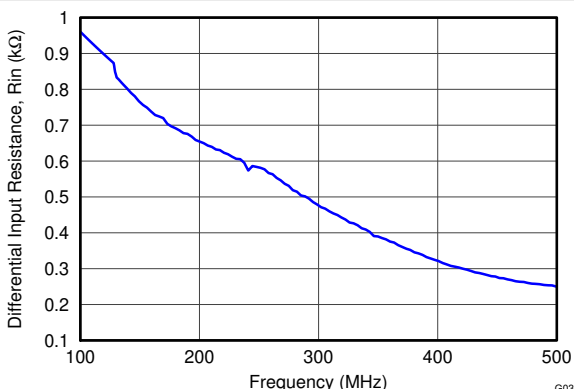
Figure 9-2. ADC Analog Input Resistance ( R_{IN} ) vs Frequency
