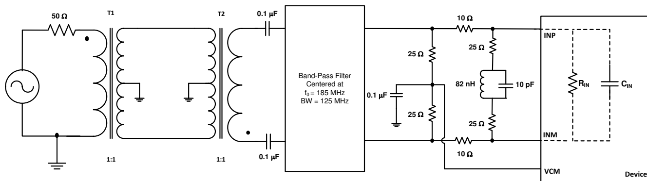
Figure 9-4. Driving Circuit for a 50-Ω Source Impedance and Input Frequencies in the Second Nyquist Zone
