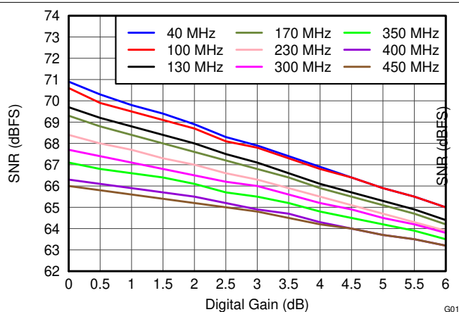
Figure 6-16. Signal-to-Noise Ratio vs Digital Gain
