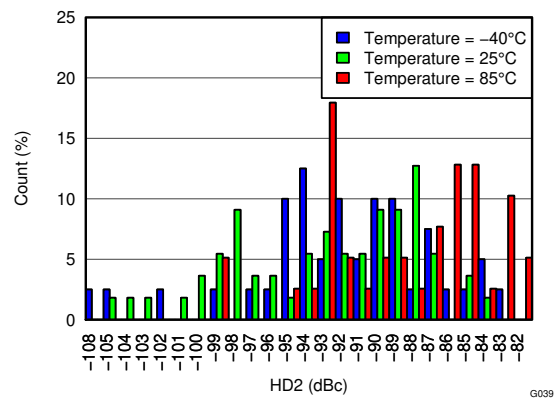
Figure 6-13. HD2 Distribution over Multiple Devices
