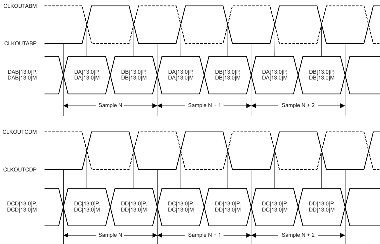
8-4. DDR LVDS Interface Timing Diagram
