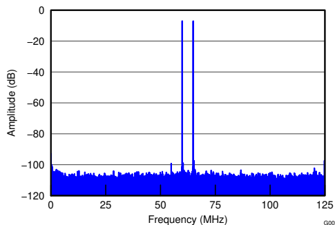
FIG 6-8. FFT for Two-Tone Input Signal
