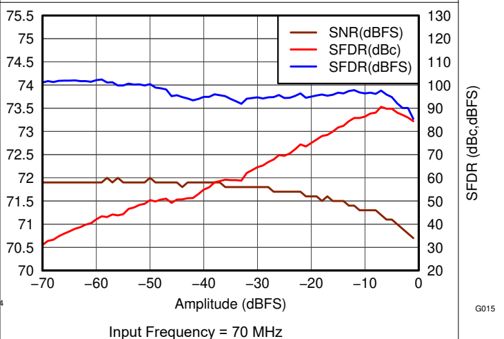
Figure 6-17. Performance vs Input Amplitude
