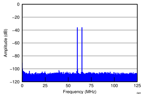
FIG 6-9. FFT for Two-Tone Input Signal
