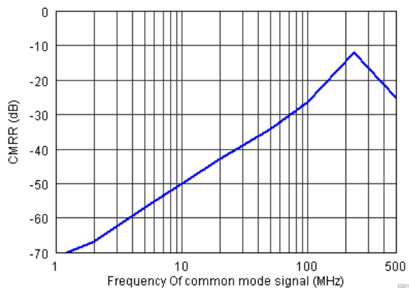
FIG 7-26. CMRR Across Frequency
