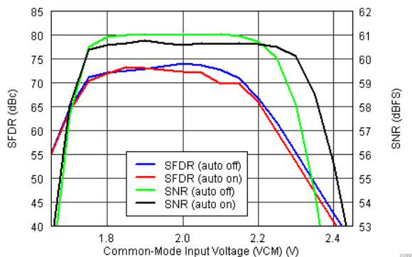
FIG 7-19. Performance Across Input Common-Mode Voltage
