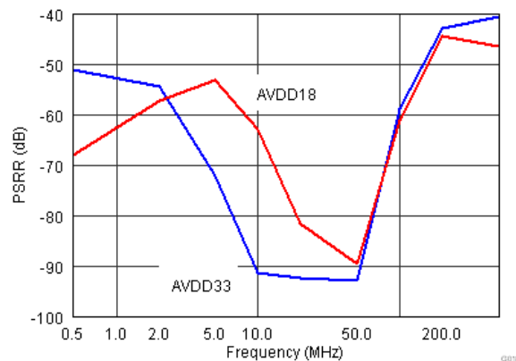
FIG 7-27. PSRR Across Frequency
