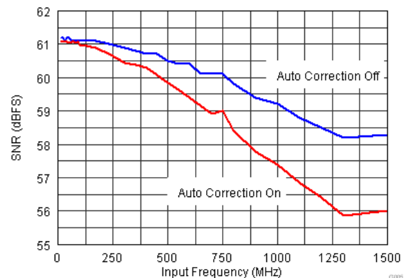
FIG 7-11. SNR vs. Input Frequency
