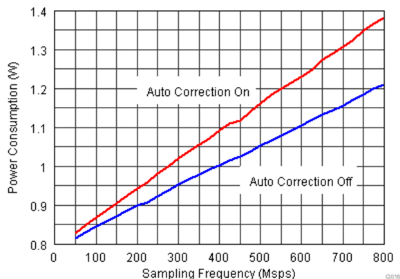
FIG 7-28. Power Across Sampling Frequency
