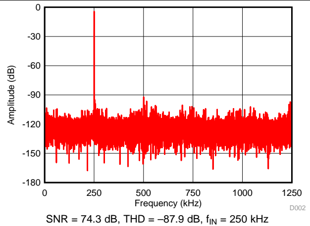
Figure 4. Typical FFT
