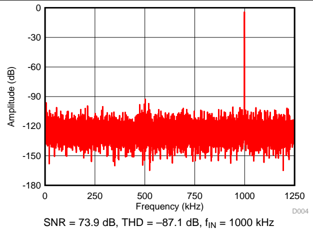
Figure 6. Typical FFT
