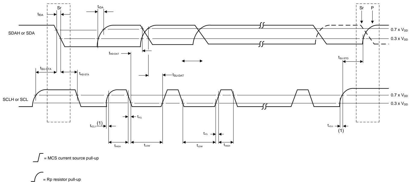
2. Timing Diagram for High Speed Mode
