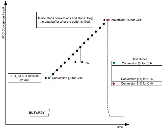
⊗ 62. Start Burst with Single Channel Configurations
