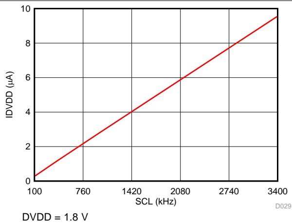
⊗ 27. I_{DVDD} in Manual Mode with SCL
