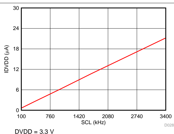
Figure 70. I_{DVDD} in Manual Mode with SCL
