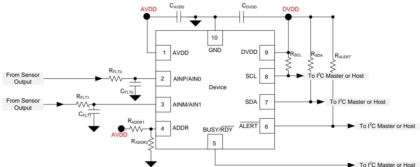
Figure 123. Example Circuit
