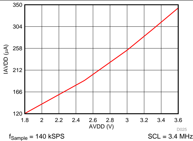
⊗ 25. I_{AVDD} in Manual Mode with AVDD
