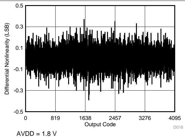
FIG 18. Typical DNL in Manual Mode
