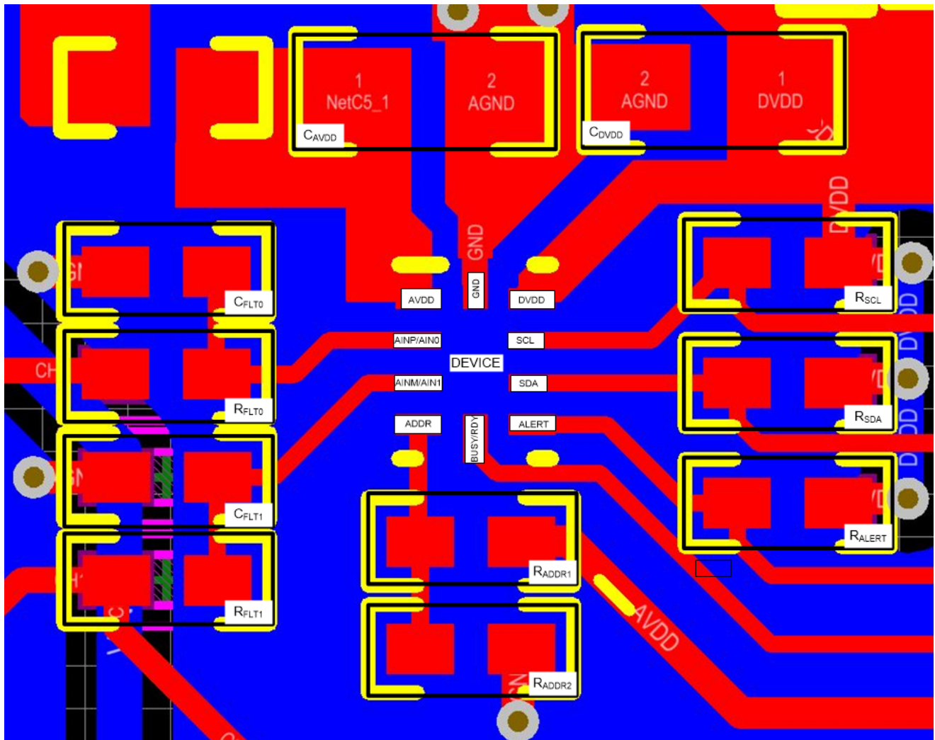
124. Example Layout
