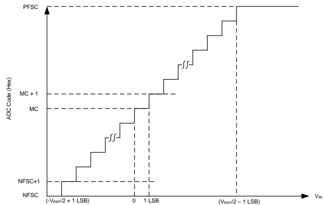
图 44. Ideal Transfer Characteristics for Pseudo-Differential Configuration
