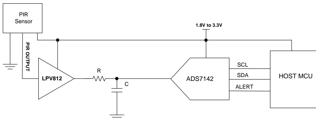
FIG 119. PIR Sensor with ADS7142
