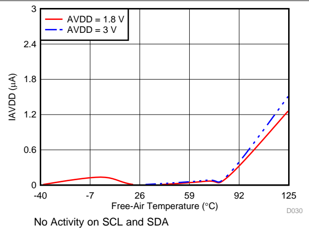
⊗ 28. Static I_{AVDD} in Manual Mode with Temperature
