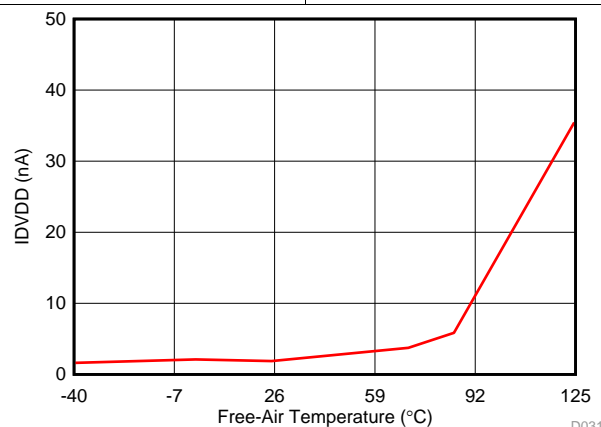
⊗ 27. I_{DVDD} in Manual Mode with SCL
