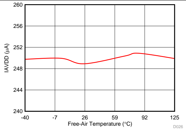
⊗ 26. I_{AVDD} in Manual Mode with Temperature
