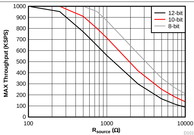
Figure 65. 1 \times V_{REF} Input Range Settling Without an MXO Buffer
