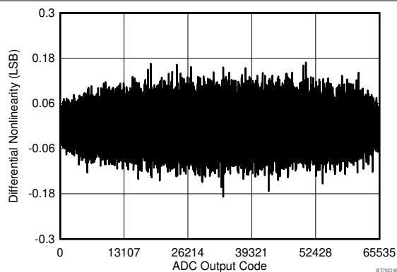
図 5-5. Typical DNL
