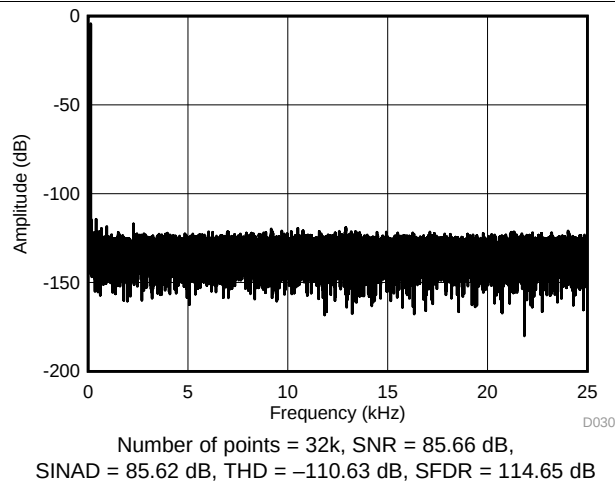
Figure 34. Typical FFT Plot for OSR 4x ( \pm 10\text{ V} )
