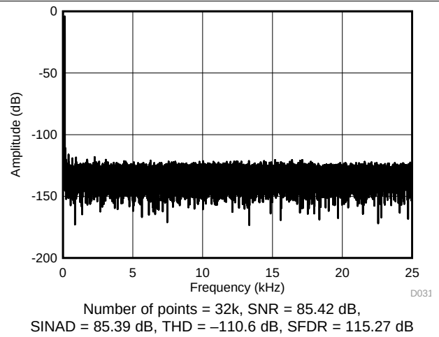
Figure 35. Typical FFT Plot for OSR 4x ( \pm 5\text{ V} )
