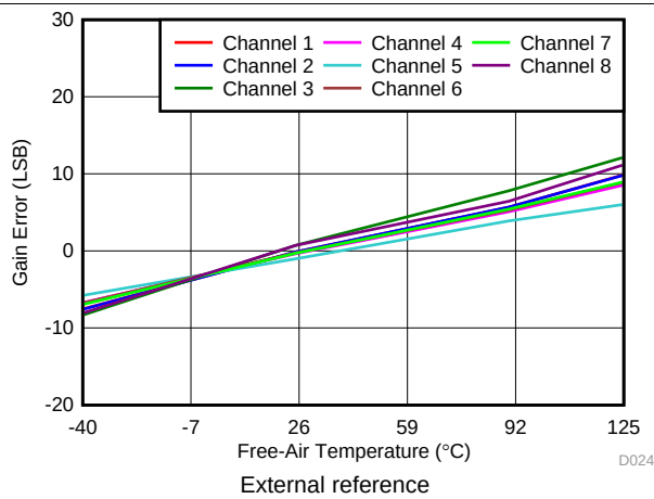
Figure 28. Gain Error Across Channels vs Temperature ( \pm 10\text{ V} )
