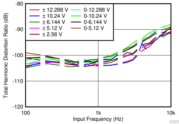
图 6-39. THD vs Input Frequency
