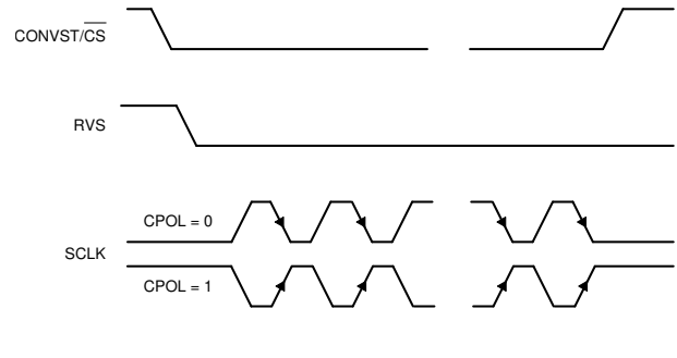
図 7-29. Standard SPI Timing Protocol (CPHA = 1, Single SDO-x)
