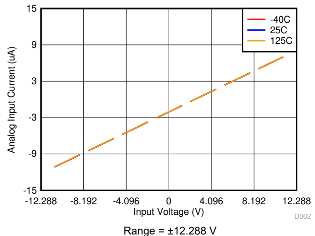
图 6-10. Input I-V Characteristic Across Temperature
