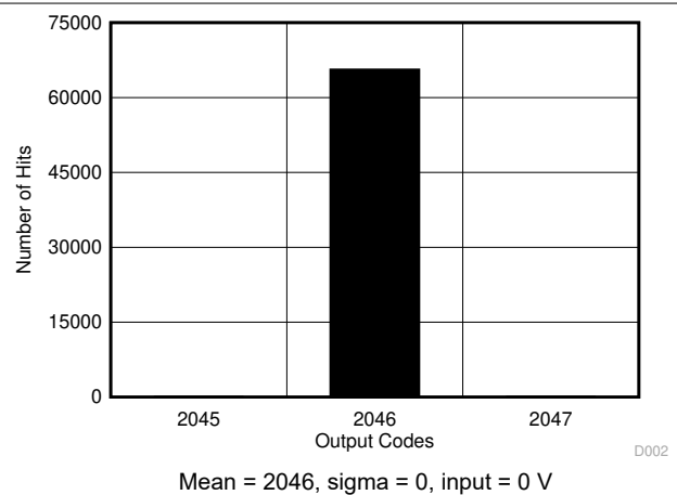
图 6-14. DC Histogram for Mid-Scale Inputs ( \pm 10.24\text{ V} )
