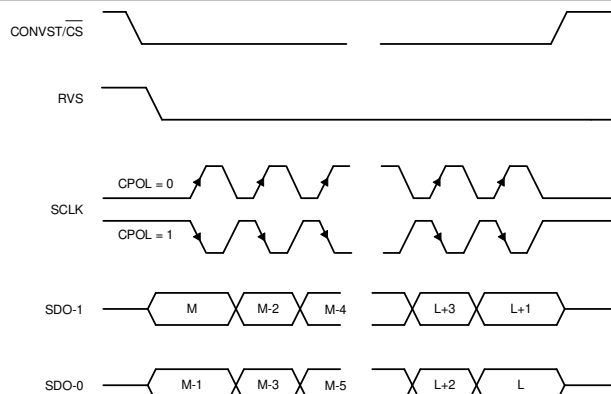
図 7-30. Standard SPI Timing Protocol (CPHA = 0, Dual SDO-x)
