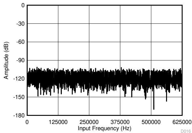
图 6-33. Typical FFT Plot (All Ranges) for the ADS8661
