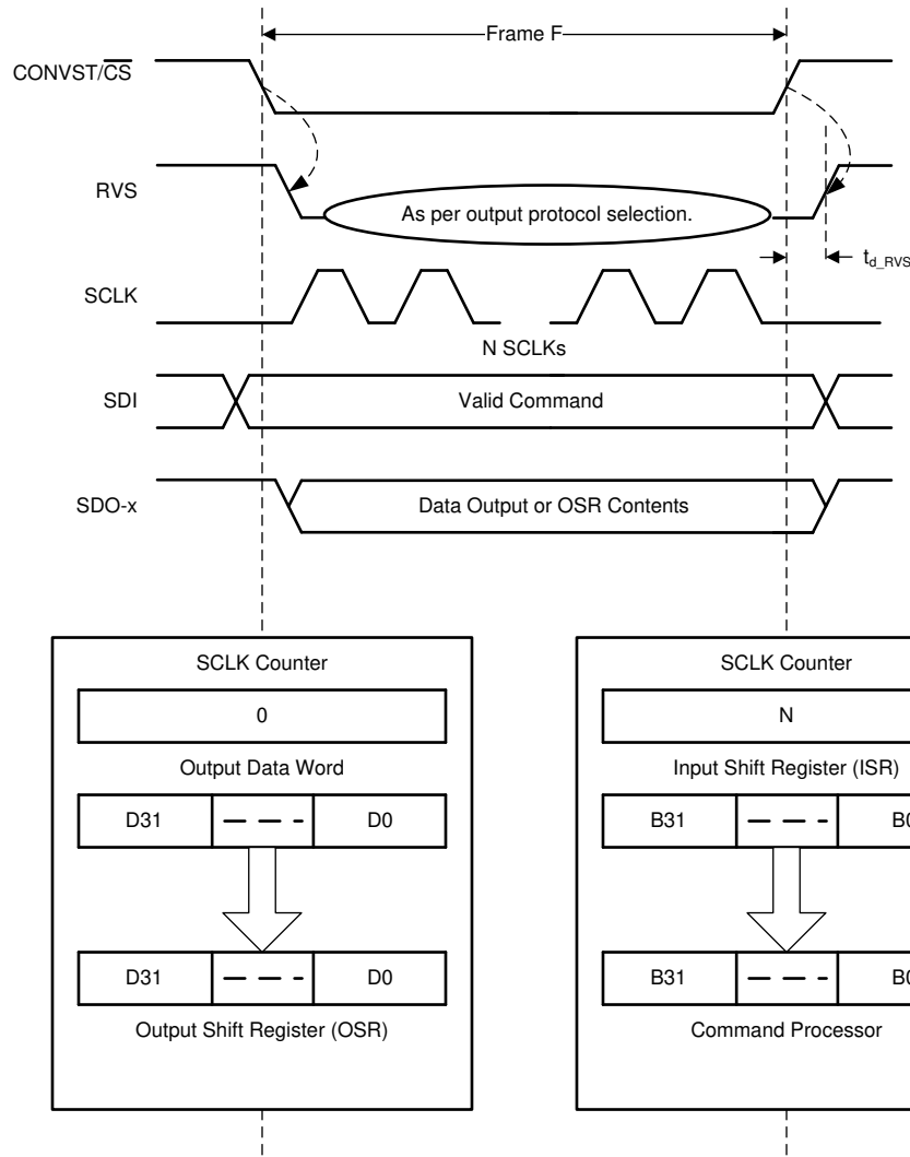
Figure 7-25. Data Transfer Frame
