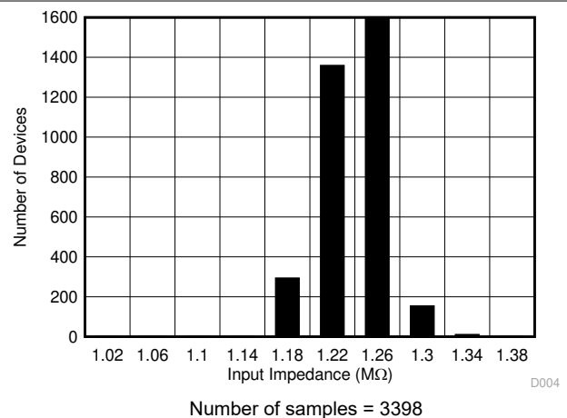
图 6-12. Typical Distribution of Input Impedance
