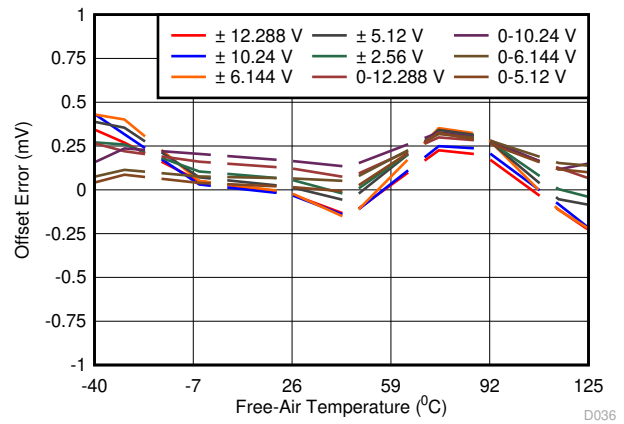
FIG 6-28. Offset Error vs Temperature Across Input Ranges
