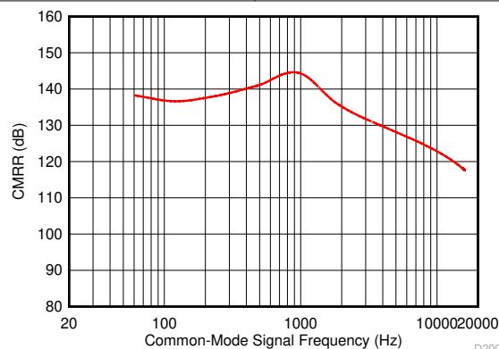
FIG 8-7. Common-Mode Rejection Ratio vs Frequency
