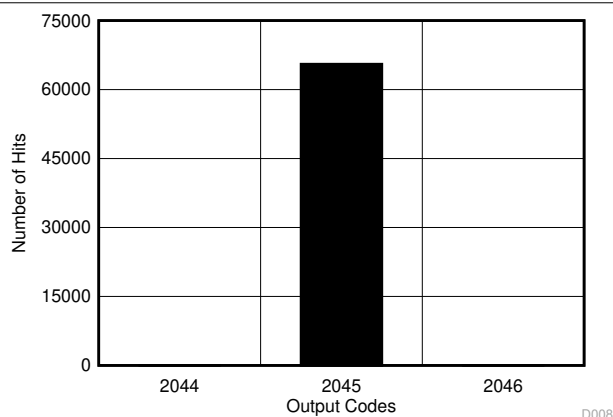
FIG 6-18. DC Histogram for Mid-Scale Inputs ( 0\text{ V} – 12.288\text{ V} )
