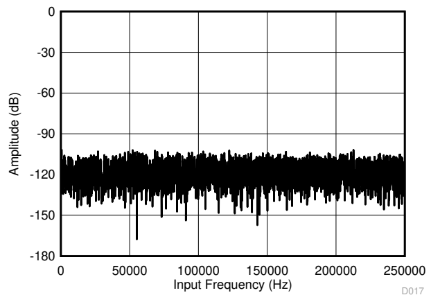
图 6-34. Typical FFT Plot (All Ranges) for the ADS8665
