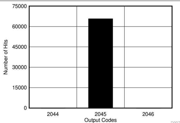
FIG 6-17. DC Histogram for Mid-Scale Inputs ( \pm 2.56\text{ V} )
