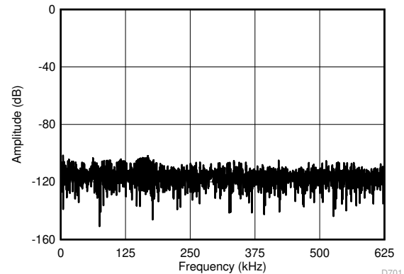
FIG 8-4. FFT Plot With an AC Common-Mode at 1.25 MSPS
