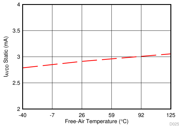
图 6-41. AVDD Current vs Temperature
