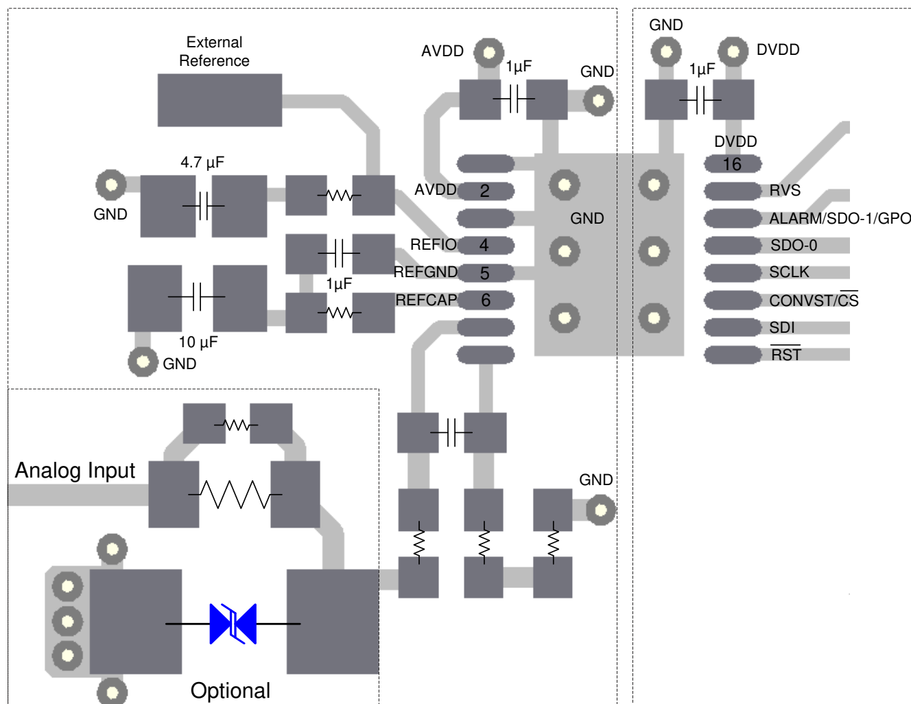
图 10-1. Board Layout for the ADS866x
