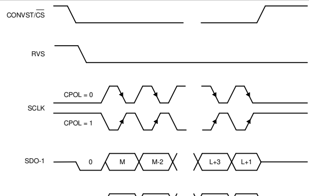
図 7-31. Standard SPI Timing Protocol (CPHA = 1, Dual SDO-x)
