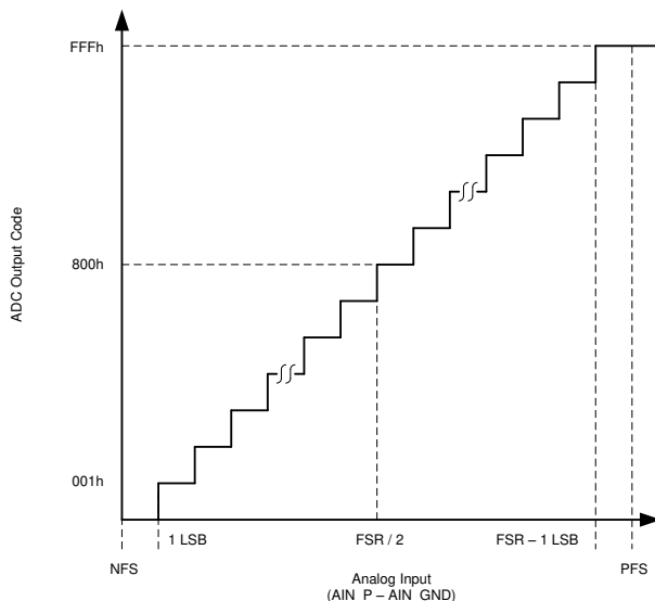
図 7-15. Device Transfer Function (Straight-Binary Format)
