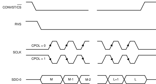
図 7-28. Standard SPI Timing Protocol (CPHA = 0, Single SDO-x)
