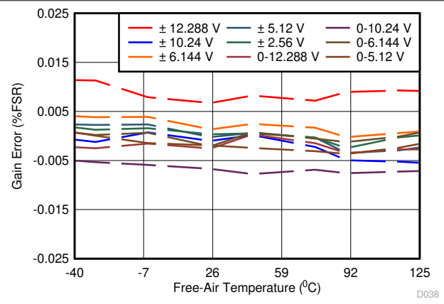
FIG 6-30. Gain Error vs Temperature Across Input Ranges
