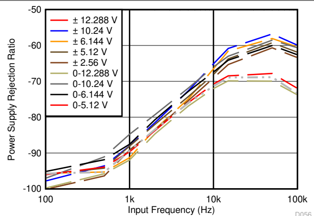
8-11. PSRR With a Decoupling Capacitor
