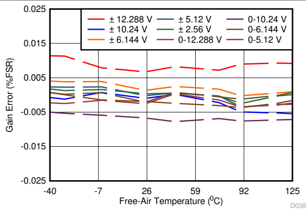
6-30. Gain Error vs Temperature Across Input Ranges
