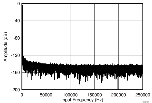
FIG 6-34. Typical FFT Plot (All Ranges) for the ADS8685
