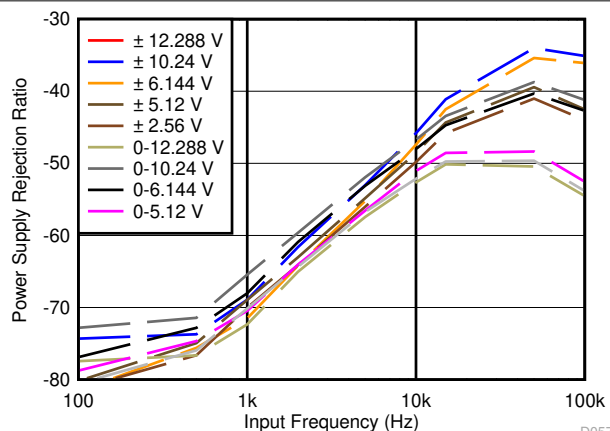
8-10. PSRR Without a Decoupling Capacitor
