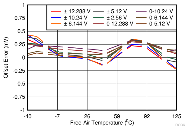
6-28. Offset Error vs Temperature Across Input Ranges
