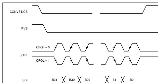
7-30. Standard SPI Timing Protocol (CPHA = 0, 32 SCLK Cycles)
