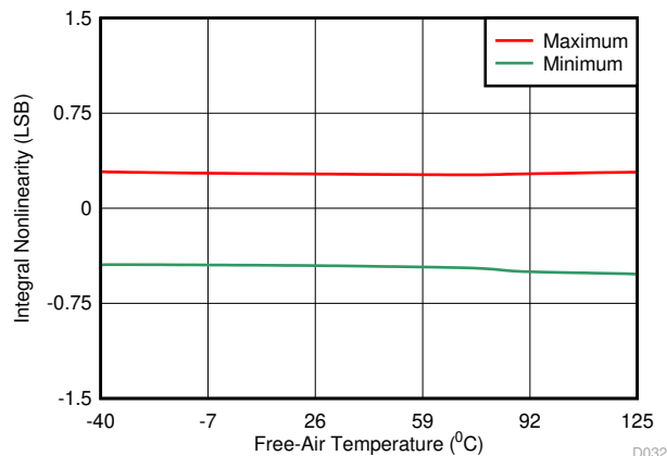
6-27. INL vs Temperature (All Unipolar Ranges)
