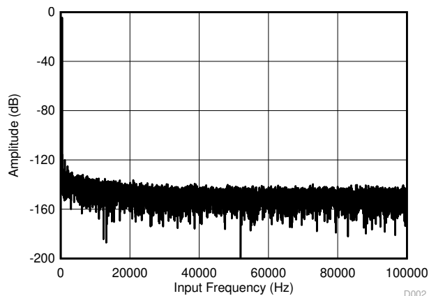
FIG 6-33. Typical FFT Plot (All Ranges) for the ADS8681
