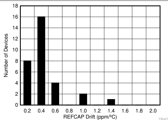
Figure 7-16. Reference Buffer Temperature Drift Histogram (PW Package)
