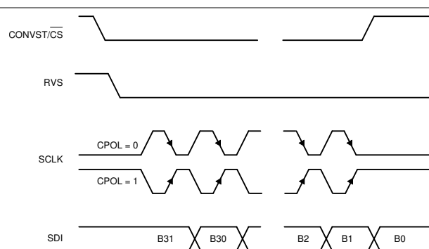
7-31. Standard SPI Timing Protocol (CPHA = 1, 32 SCLK Cycles)
