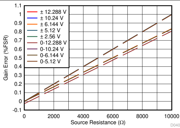
6-32. Gain Error vs External Resistance ( R_{EXT} )
