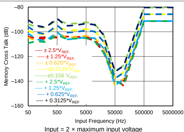
FIG 59. Memory Crosstalk vs Frequency for Overrange Inputs
