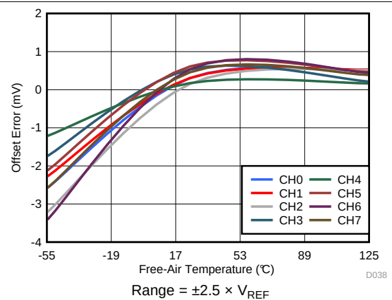
Figure 37. Offset Error vs Temperature Across Channels
