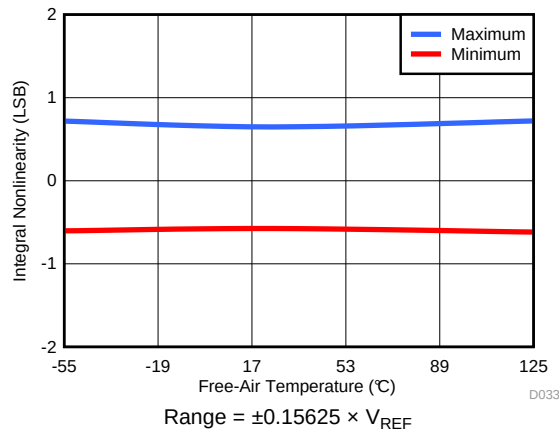
Figure 32. INL vs Temperature ( \pm 0.15625 \times V_{REF} )
