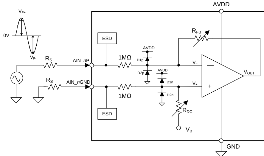
図 66. Input Overvoltage Protection Circuit Schematic
