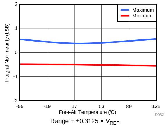
FIG 31. INL vs Temperature ( \pm 0.3125 \times V_{REF} )
