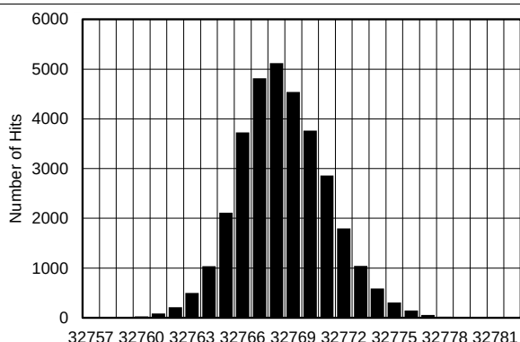
图 10. DC Histogram for Mid-Scale Inputs ( 1.25 \times V_{REF} )
