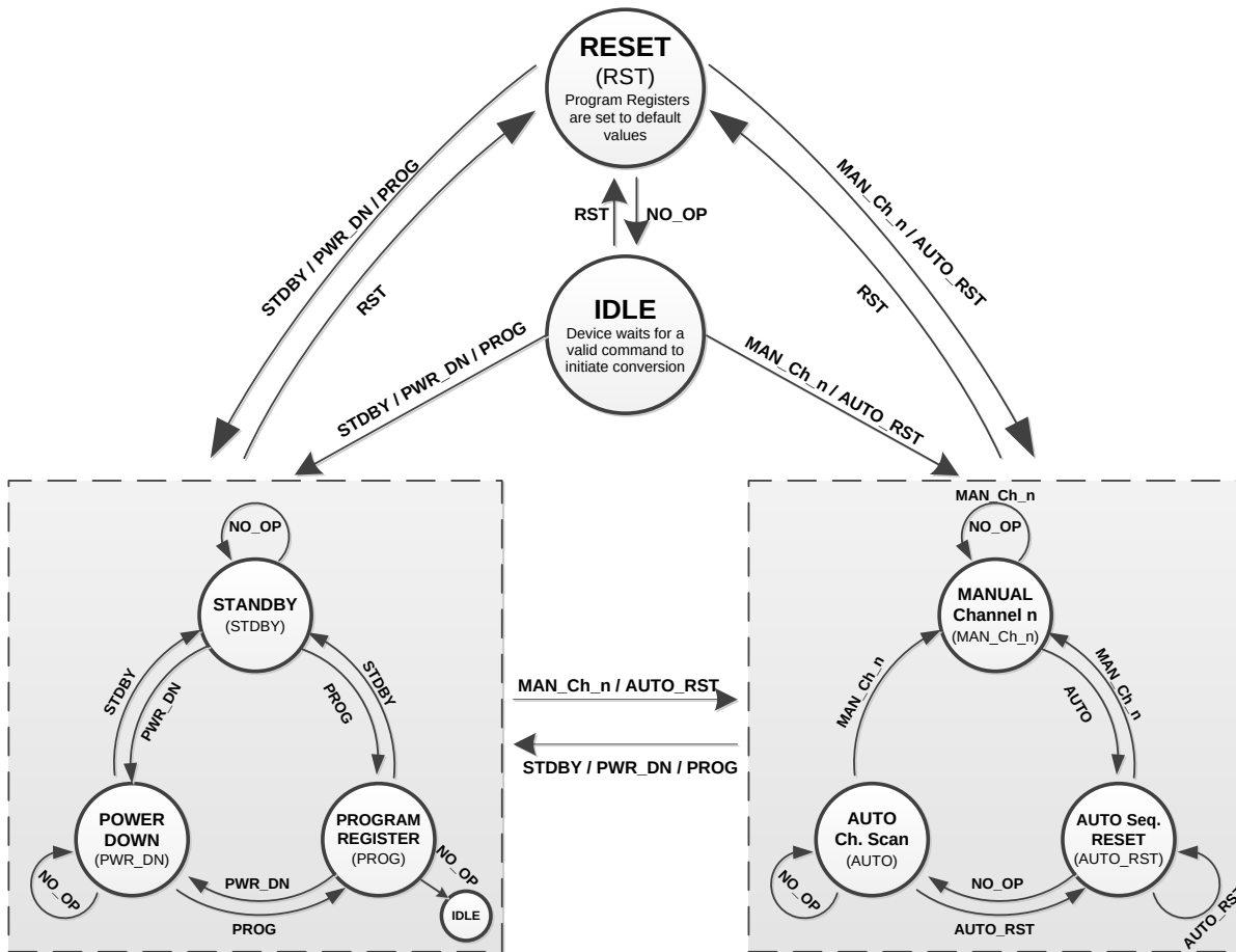
図 91. State Transition Diagram
