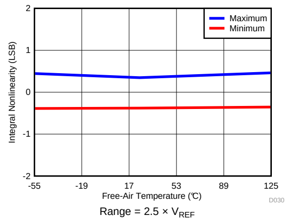
FIG 29. INL vs Temperature ( 2.5 \times V_{REF} )
