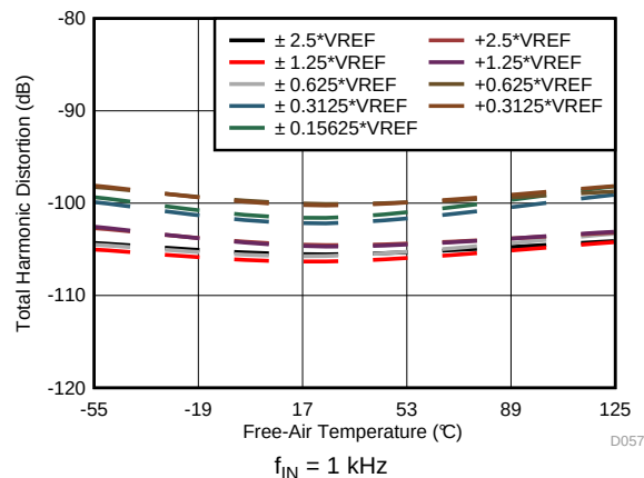
FIG 56. THD vs Temperature
