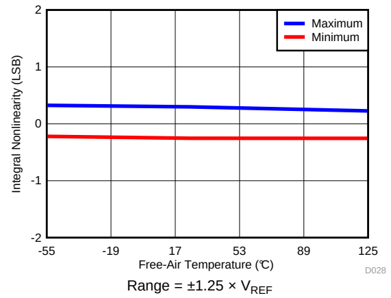
FIG 27. INL vs Temperature ( \pm 1.25 \times V_{REF} )
