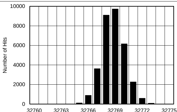
图 11. DC Histogram for Mid-Scale Inputs ( \pm 0.3125 \times V_{REF} )
