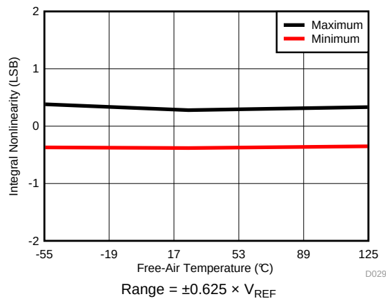
FIG 28. INL vs Temperature ( \pm 0.625 \times V_{REF} )
