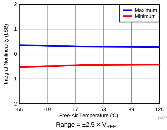
FIG 26. INL vs Temperature ( \pm 2.5 \times V_{REF} )
