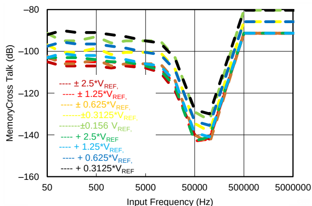
FIG 57. Memory Crosstalk vs Frequency
