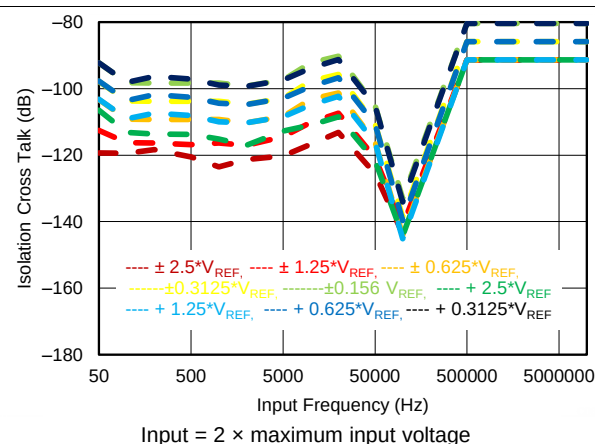
FIG 60. Isolation Crosstalk vs Frequency for Overrange Inputs
