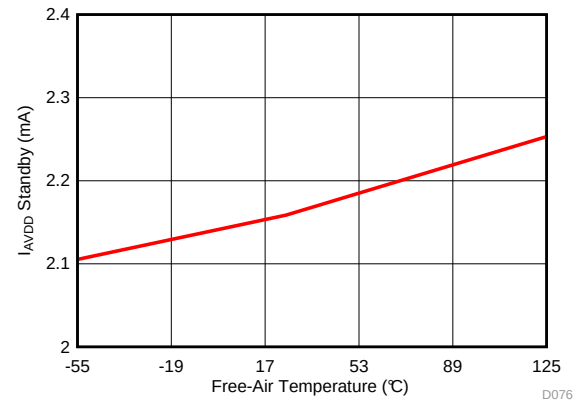
图 63. AVDD Current vs Temperature (STANDBY)
