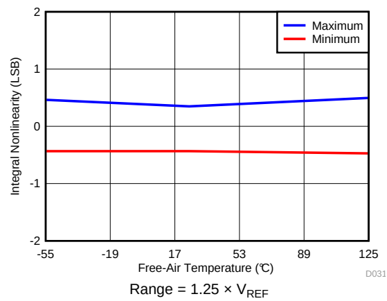
FIG 30. INL vs Temperature ( 1.25 \times V_{REF} )
