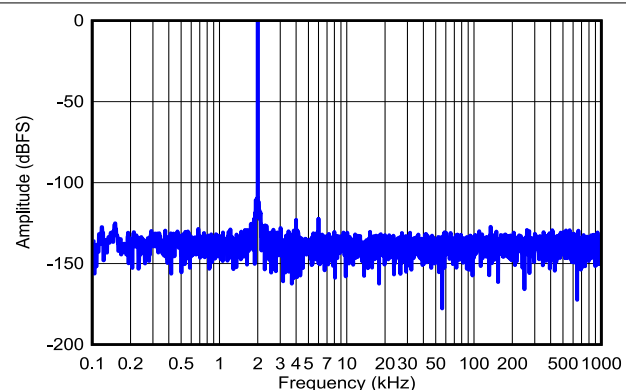
図 5-9. Typical FFT With Wide-Bandwidth LPF, RANGE = ±5V
