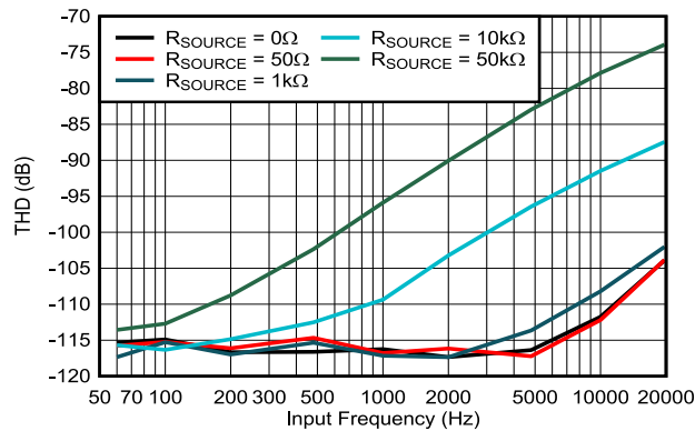
Low-Bandwidth LPF and RANGE = \pm 5V
