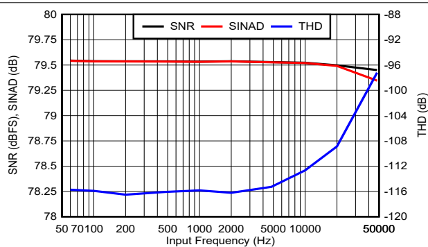
FIG 5-14. SNR, SINAD, and THD vs Input Signal Frequency
