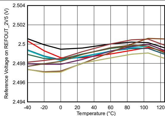
FIG 5-31. REFOUT_2V5 vs Temperature
