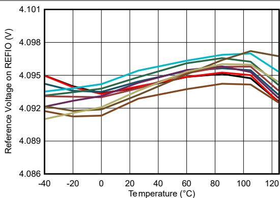
FIG 5-30. REFIO vs Temperature
