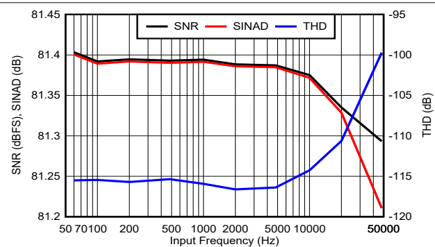
FIG 5-15. SNR, SINAD, and THD vs Input Signal Frequency
