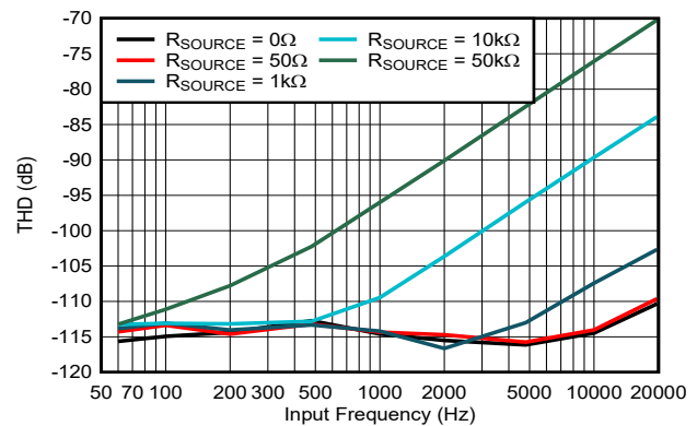
Wide-Bandwidth LPF and RANGE = \pm 10V
