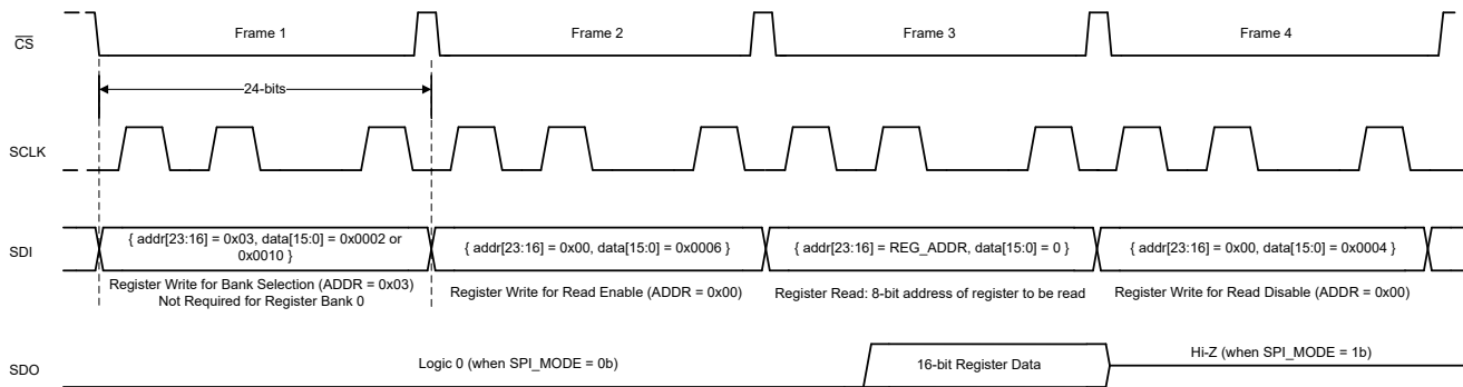
図 6-12. Register Read
