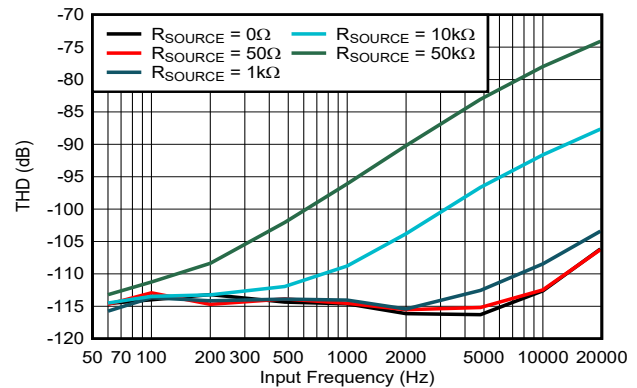
Low-Bandwidth LPF and RANGE = \pm 10V
