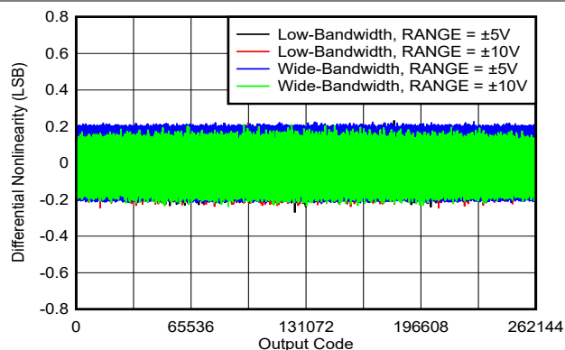
図 5-7. Typical DNL With Low-Noise LPF
