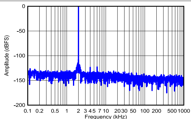
図 5-8. Typical FFT With Low-Bandwidth LPF, RANGE = ±5V
