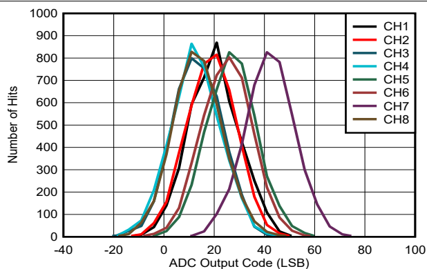
FIG 5-33. DC Histogram of Codes for V_{IN} = 1mV , Low-Bandwidth, RANGE = \pm 5V
