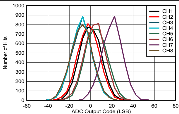
FIG 5-32. DC Histogram of Codes for A_{INxP} = A_{INxM} = GND , Low-Bandwidth, RANGE = \pm 5V
