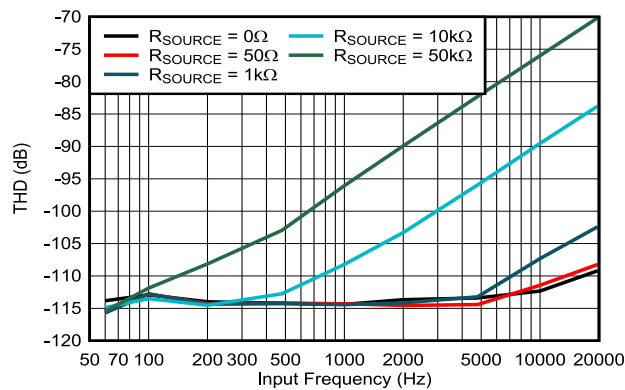
Wide-Bandwidth LPF and RANGE = \pm 5V
