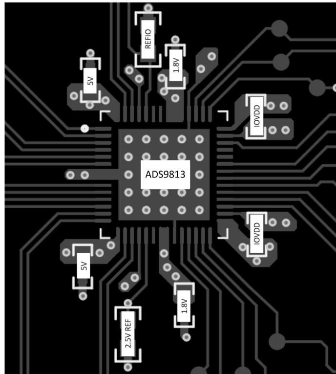
✕ 8-5. Example Layout
