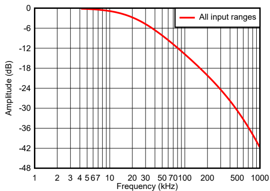
FIG 5-12. Low-Noise LPF Frequency Response Across Input Ranges
