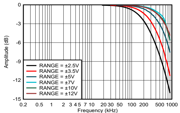
FIG 5-13. Wide-Bandwidth LPF Frequency Response Across Input Ranges
