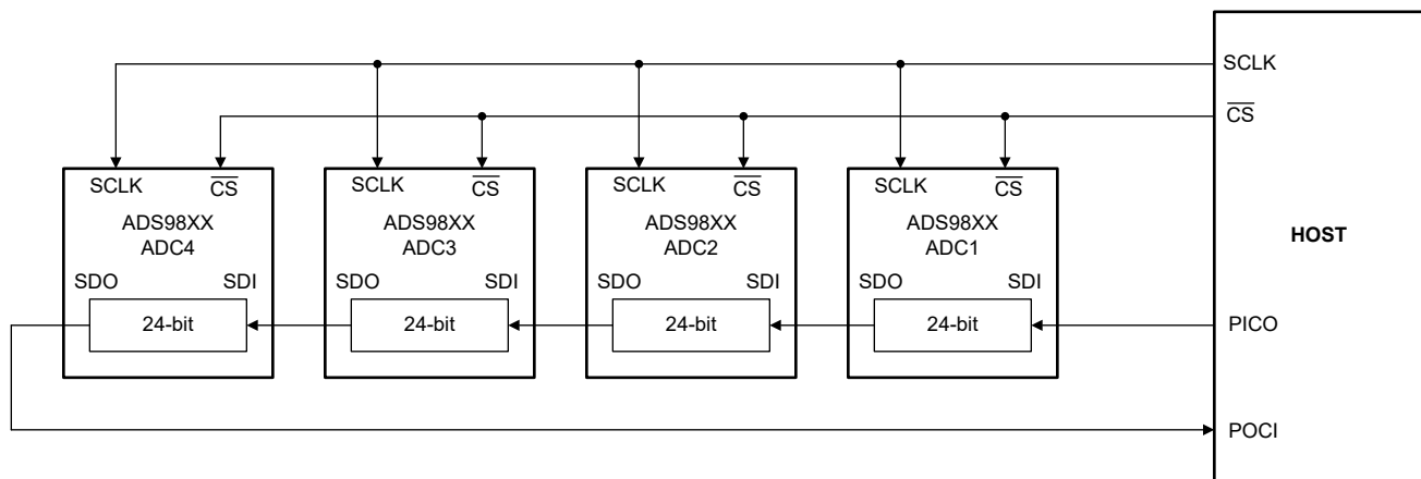
図 6-13. Daisy-Chain Connections for Configuration SPI
