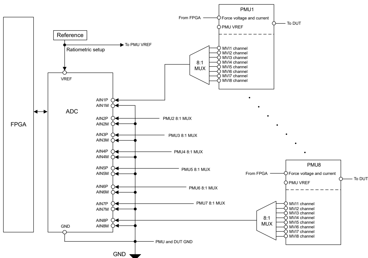
8-2. PMU With a Multiplexer
