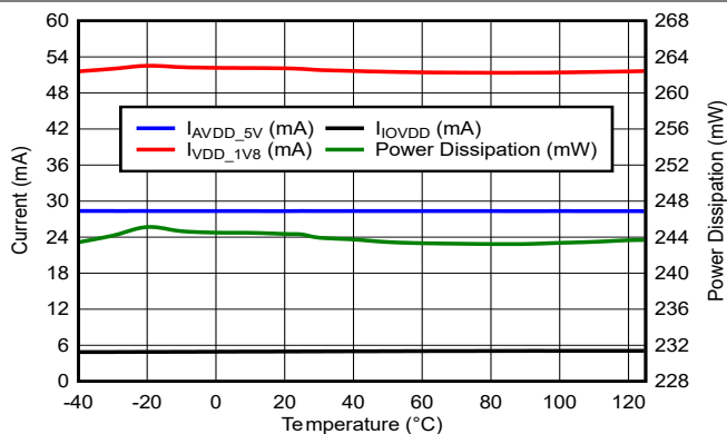
5-36. Supply Currents and Total Power Dissipation vs Temperature
