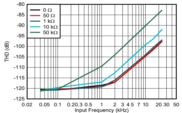
図 5-27. THD vs Input Frequency, High-BW Mode, RANGE = \pm 5V , ADS9815
