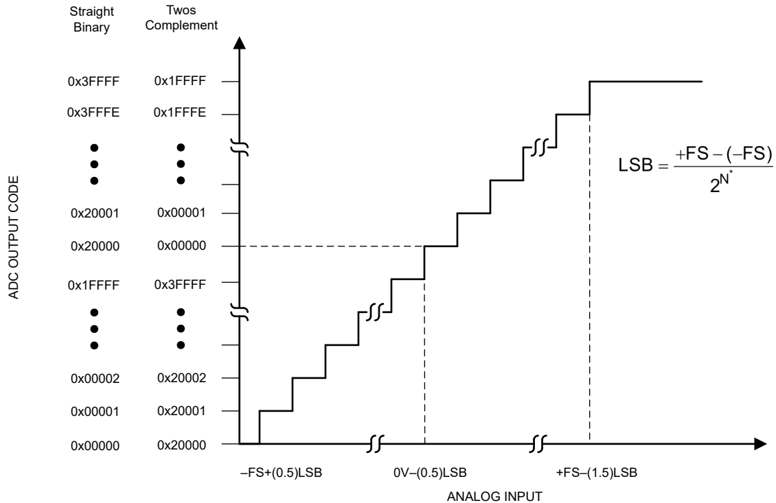
図 6-3. Transfer Characteristics
