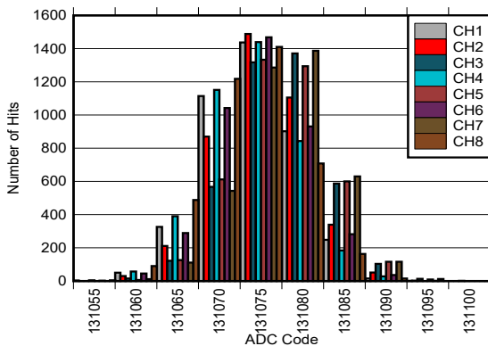
图 5-42. DC Histogram of Codes for AINxP = AINxM = GND , Wide-BW Mode, RANGE = \pm 5V
