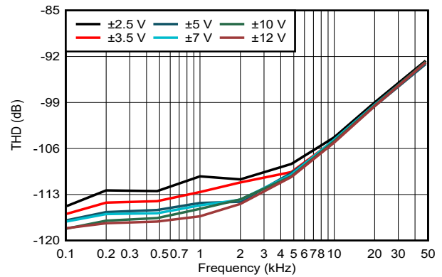
图 5-19. THD vs Input Signal Frequency Across Input Ranges With Wide-Bandwidth LPF
