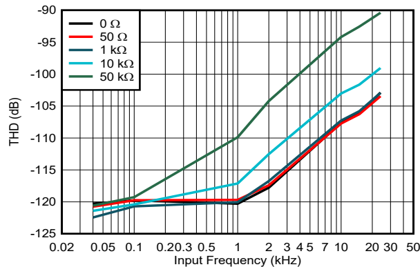
図 5-26. THD vs Input Frequency, Low-BW Mode, RANGE = \pm 5V , ADS9815
