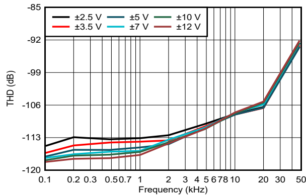
图 5-18. THD vs Input Signal Frequency Across Input Ranges With Low-Bandwidth LPF
