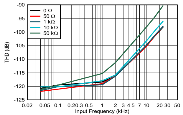
図 5-25. THD vs Input Frequency, High-BW Mode, RANGE = \pm 10V , ADS9817
