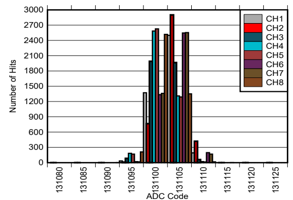
FIG 5-39. Gain Error Drift Histogram
