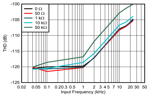
図 5-24. THD vs Input Frequency, Low-BW Mode, RANGE = \pm 10V , ADS9817
