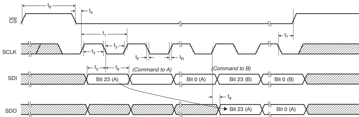
图 6-5. Timing for SPI Daisy-Chain Operation
