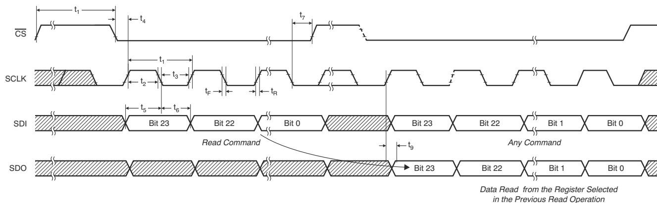
图 6-4. Timing for SPI Single-Chip Read Operation
