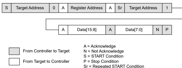
図 7-23. Read A Single Register
