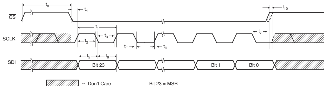
图 6-3. Timing for SPI Single-Chip Write Operation
