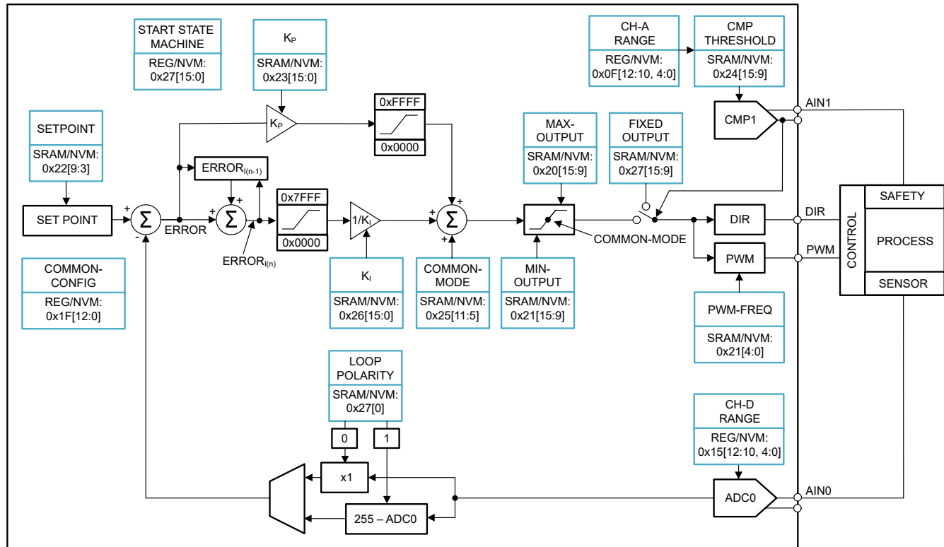
7-7. PI Controller Architecture of AFE439A2
