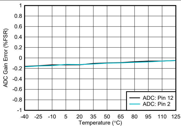
FIG 6-36. ADC Gain Error vs Temperature
