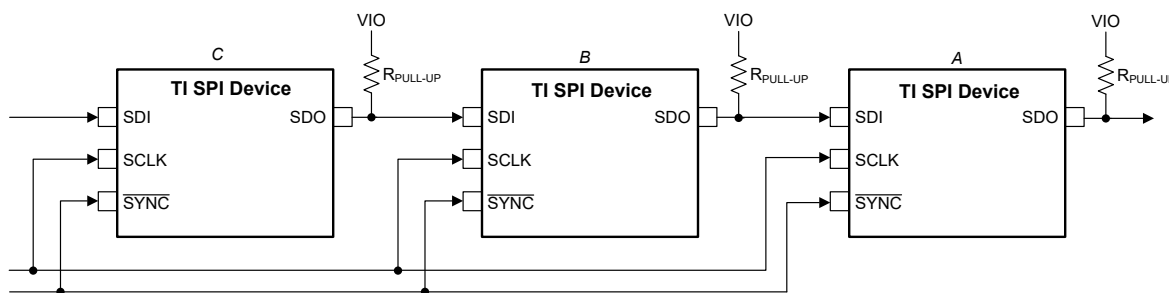
图 7-12. SPI Daisy-Chain Connection
