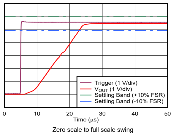
图 6-21. Voltage Output Setting Time - Rising Edge
