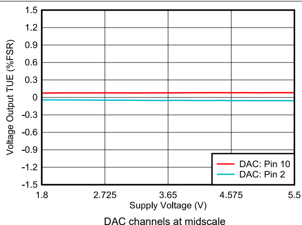
Figure 6-15. Voltage Output TUE vs Supply Voltage
