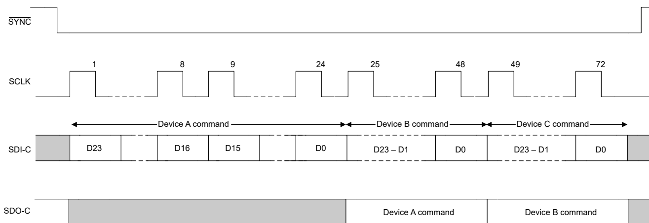
图 7-13. SPI Daisy-Chain Write Cycle
