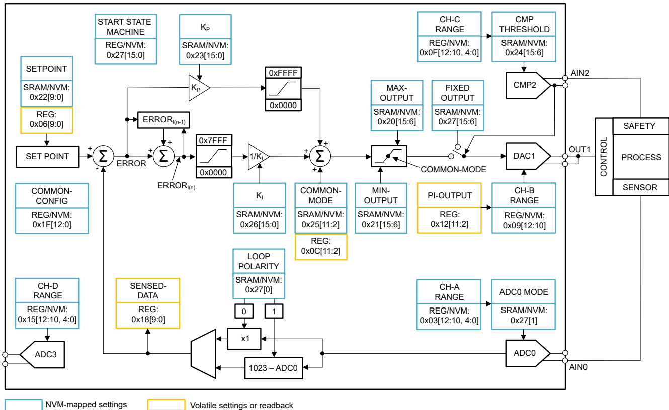
7-8. PI Controller Architecture
