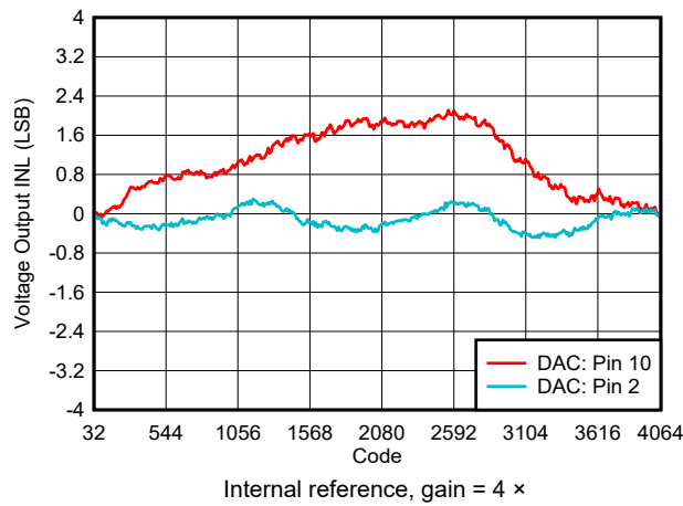
Figure 6-4. Voltage Output INL vs Digital Input Code
