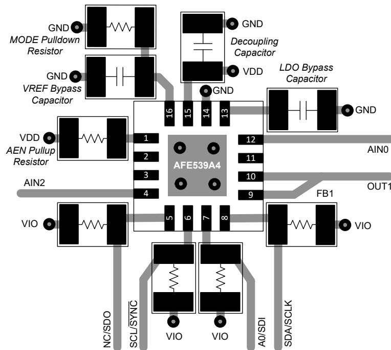
8-4. Layout Example
