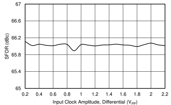
図 5-16. Spurious-Free Dynamic Range vs Input Clock Amplitude (PGA Gain = 0 dB)
