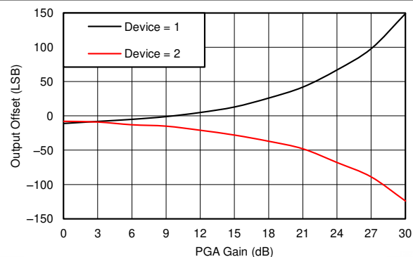
図 5-30. Channel Offset vs PGA Gain for Two Typical Devices
