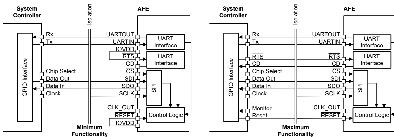
FIG 7-28. SPI Plus UART Mode Connections
