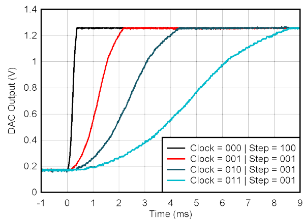
FIG 6-24. DAC Settling Time With Sinusoidal Slew Rate Control
