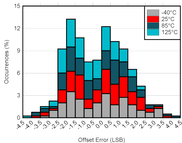
6-39. ADC Offset Error vs Temperature
