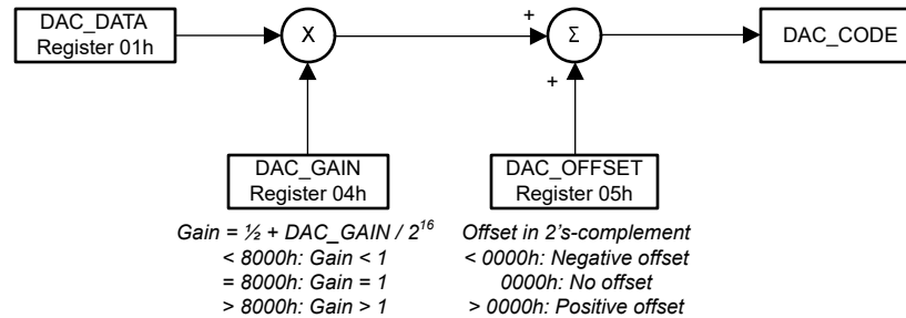
図 7-2. DAC Calibration Path
