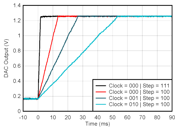
FIG 6-23. DAC Settling Time With Linear Slew Rate Control
