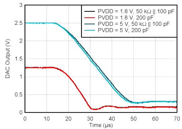
FIG 6-22. DAC Settling Time vs Load (Falling Voltage Step)
