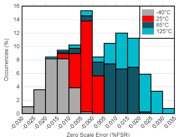
FIG 6-18. DAC Zero Scale Error vs Temperature
