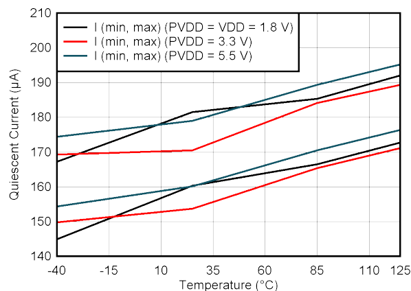
FIG 6-53. PVDD Supply Current vs Temperature
