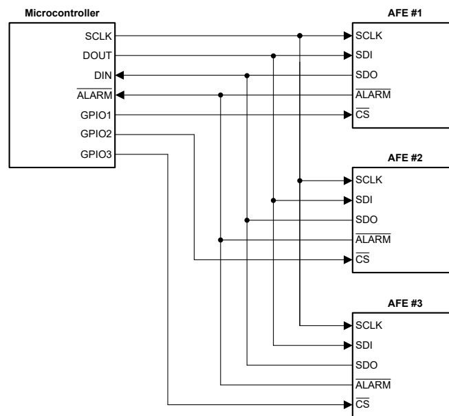
Figure 8-1. Multichannel Configuration
