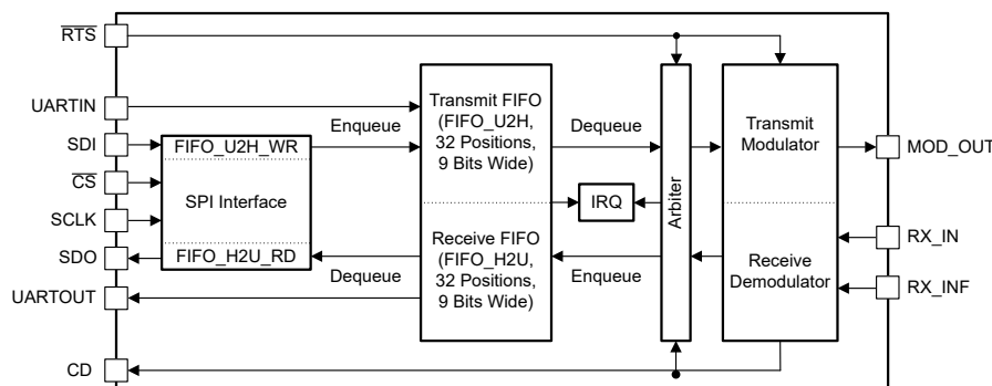
Figure 7-17. HART Architecture
