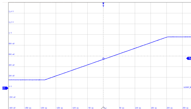
図 7-3. Linear Slew Rate: Rising
