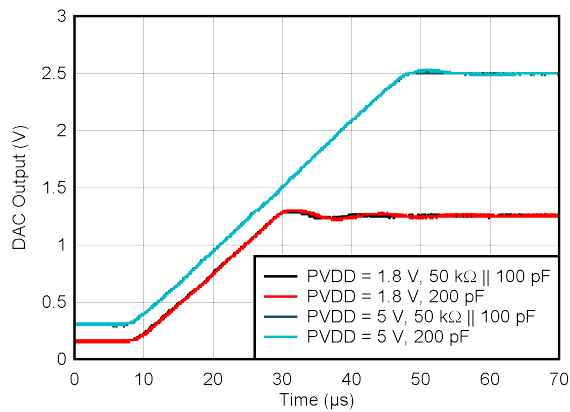
FIG 6-21. DAC Settling Time vs Load (Rising Voltage Step)
