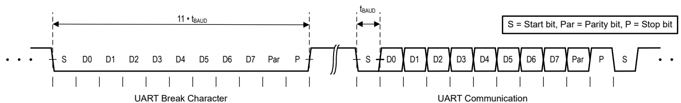
6-2. UBM Timing
