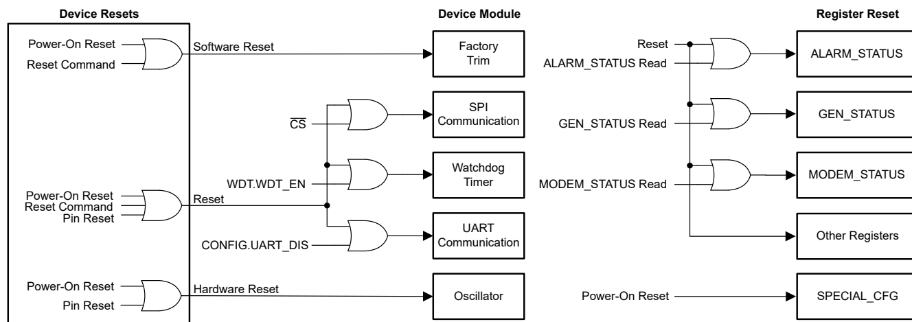
7-25. Reset Conditions
