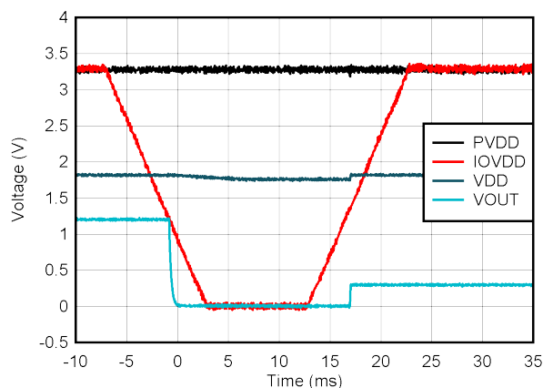
FIG 6-32. DAC IOVDD Supply Collapse Response, RANGE = 1
