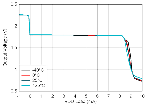
FIG 6-55. VDD Voltage vs Load Current
