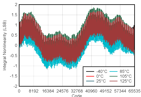
6-6. DAC INL vs Digital Input Code
