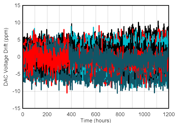
FIG 6-33. DAC Output Voltage Long-Term Stability
