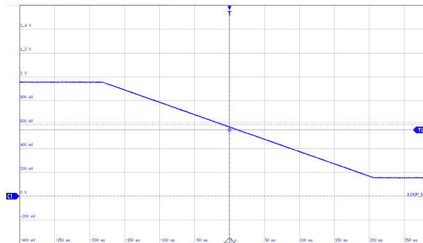
図 7-4. Linear Slew Rate: Falling
