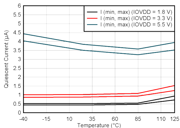
FIG 6-54. IOVDD Supply Current vs Temperature
