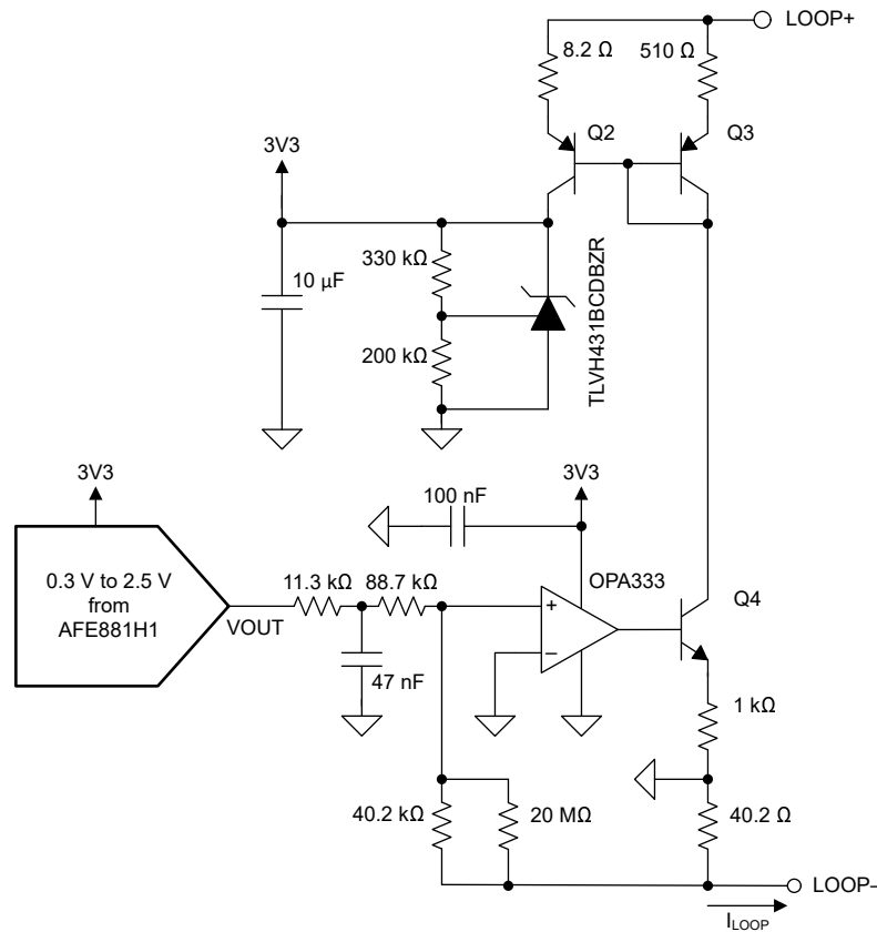
Figure 8-5. Current Loop Control for the AFE881H1 Transmitter
