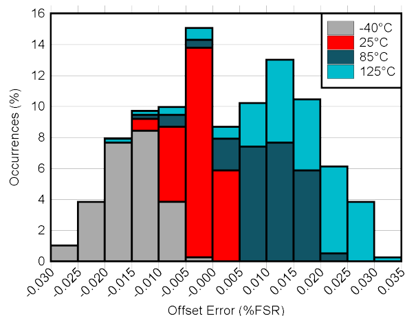
FIG 6-16. DAC Offset Error vs Temperature
