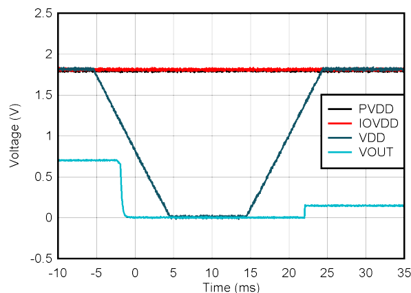
FIG 6-31. DAC VDD Supply Collapse Response, RANGE = 0
