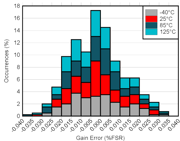
6-40. ADC Gain Error vs Temperature
