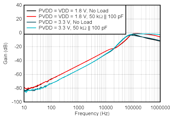
FIG 6-34. DAC AC PSRR vs Frequency
