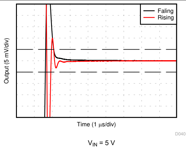
FIG 6-29. Settling Time
