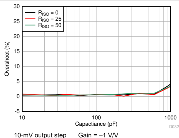
FIG 6-24. Small-Signal Overshoot vs Capacitive Load
