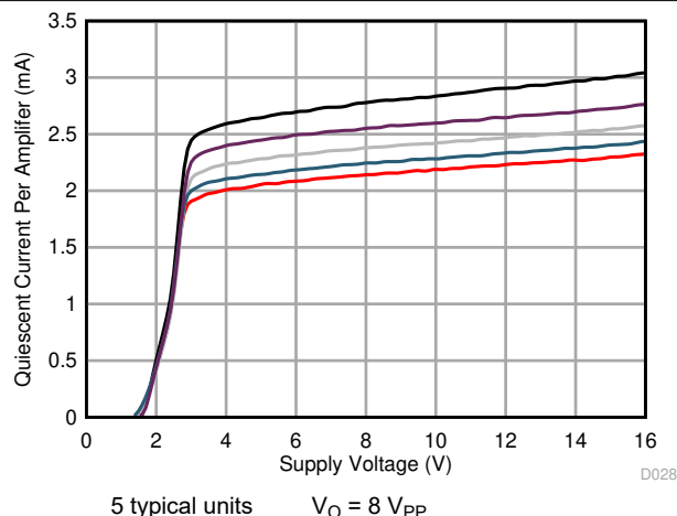
FIG 6-20. Quiescent Current vs Power Supply
