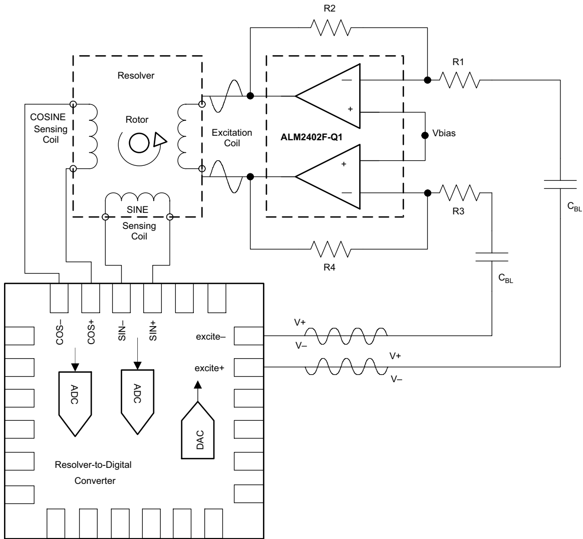
8-2. Resolver-Based Application
