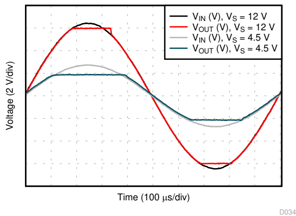
FIG 6-26. No Phase Reversal
