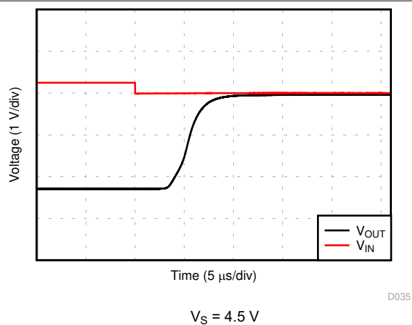
FIG 6-27. Negative Overload Recovery
