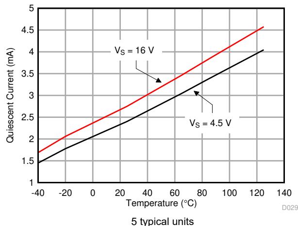
FIG 6-21. Quiescent Current vs Temperature
