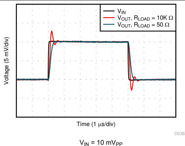
FIG 6-28. Small-Signal Step Response
