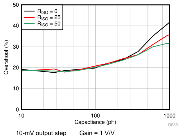
FIG 6-25. Small-Signal Overshoot vs Capacitive Load
