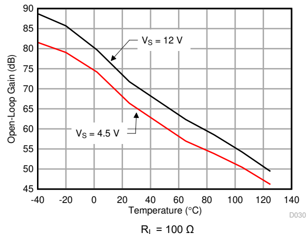
FIG 6-22. Open-Loop Gain vs Temperature
