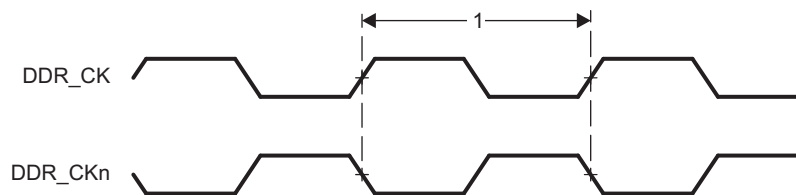
図 7-38. DDR2 Memory Interface Clock Timing
