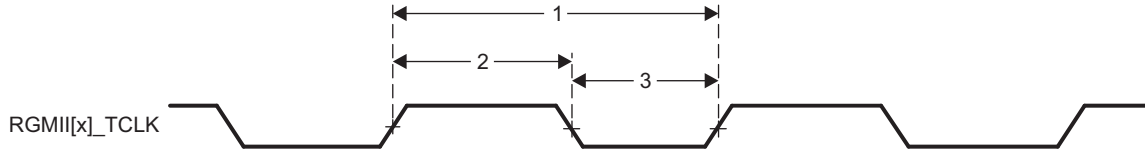
7-15. RGMII[x]_TCLK Timing - RGMII Mode
