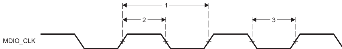
图 7-103. PRU-ICSS MDIO_CLK Timing
