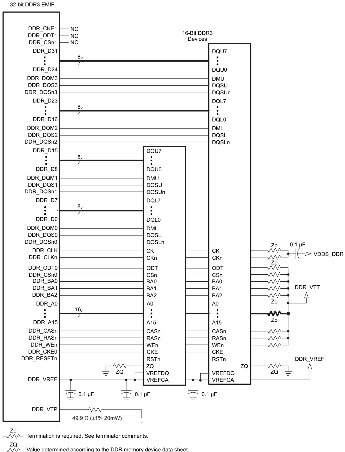
FIG 5-52. 32-Bit DDR3 Interface Using Two 16-Bit DDR3 Devices With V_{TT} Termination
