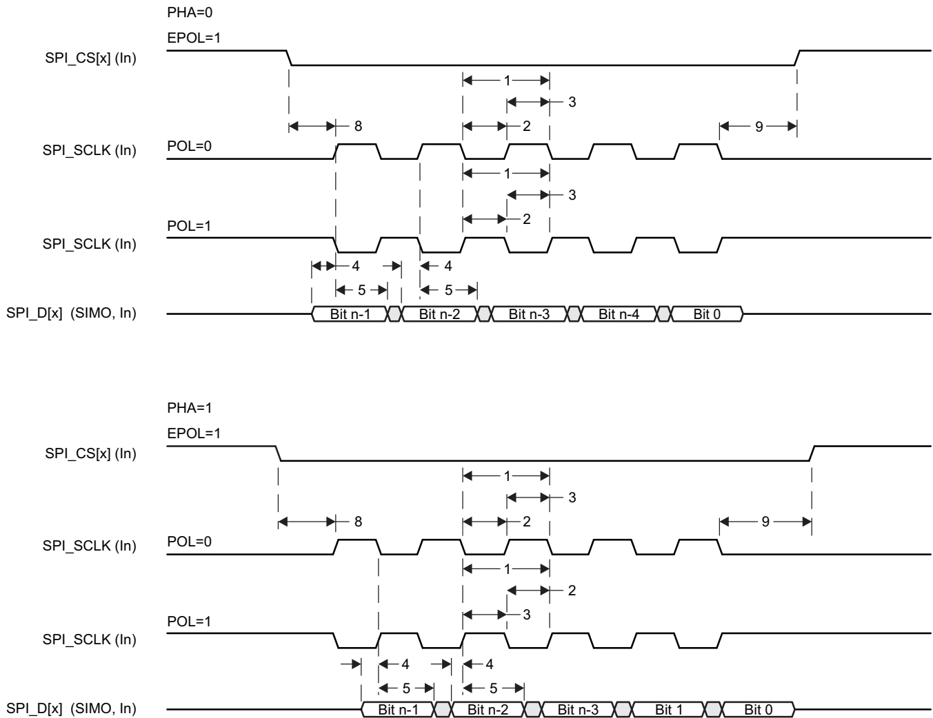
5-106. SPI Slave Mode Receive Timing
