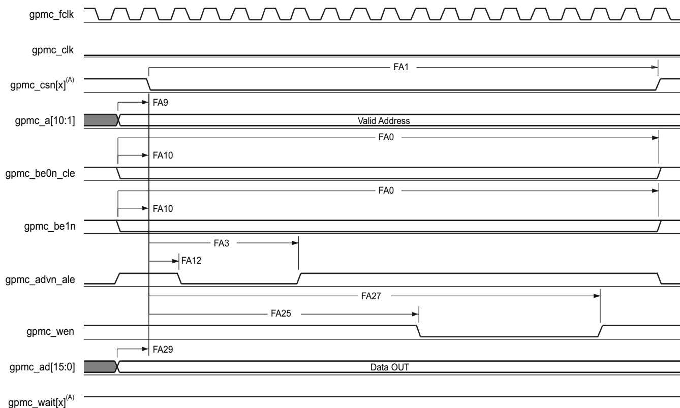
FIG 5-41. GPMC and NOR Flash—Asynchronous Write—Single Word
