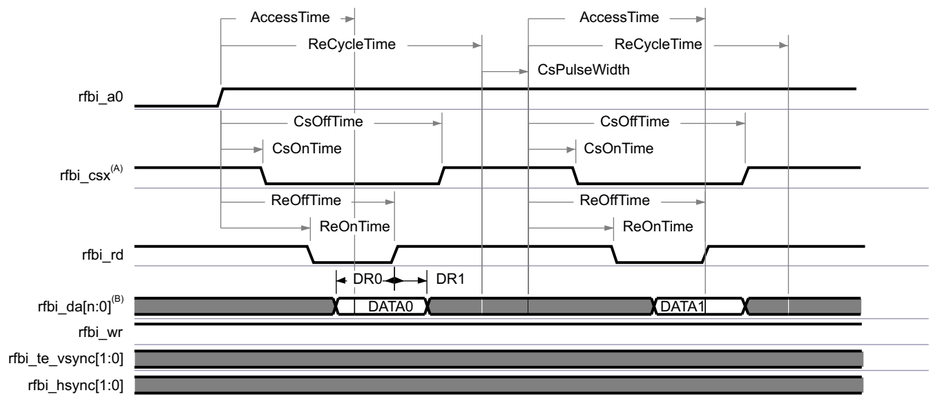
FIG 5-95. DSS—RFBI Mode—MIPI DBI 2.0—LCD Panel—Command / Data Write
