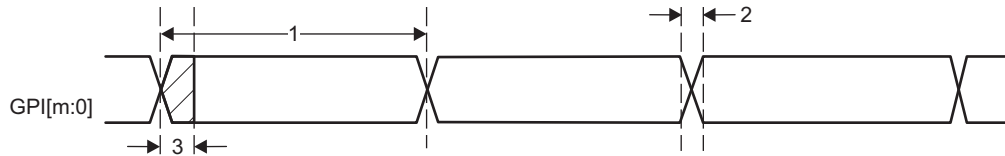
图 5-119. PRU-ICSS PRU Direct Input Timing
