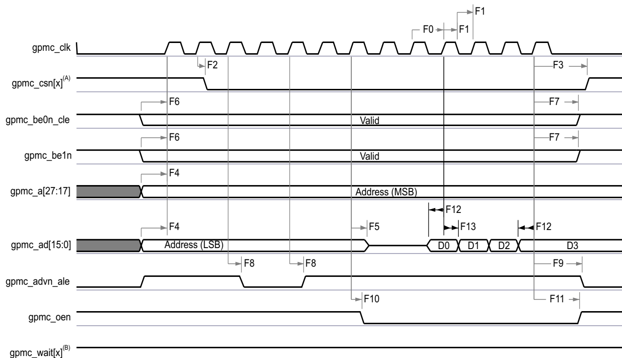
FIG 5-36. GPMC and Multiplexed NOR Flash—Synchronous Burst Read
