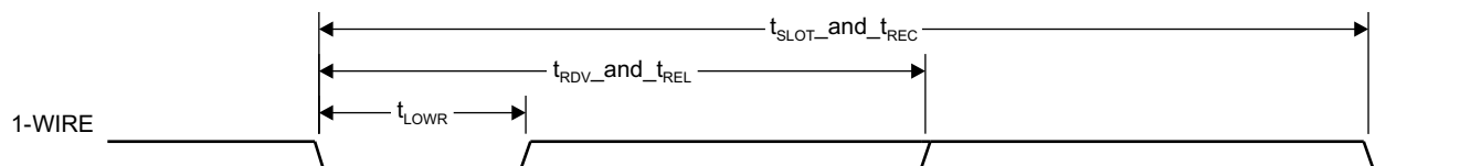
✎ 5-117. 1-Wire Read Bit Timing (Data)
