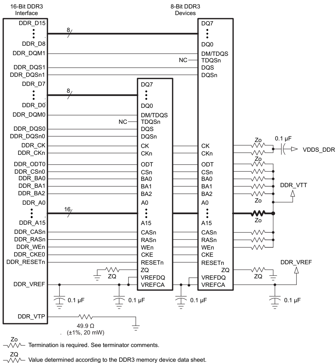
5-51. 16-Bit DDR3 Interface Using Two 8-Bit DDR3 Devices With V_{\Pi} Termination
