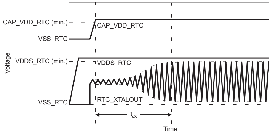
図 5-14. OSC1 Start-up Time
