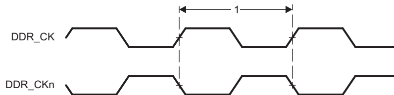
図 5-48. DDR3 Memory Interface Clock Timing
