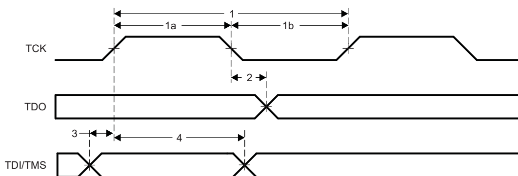
图 5-146. JTAG Timing
