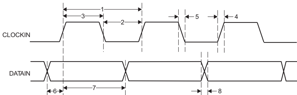
図 5-121. PRU-ICSS PRU Parallel Capture Timing - Rising Edge Mode
