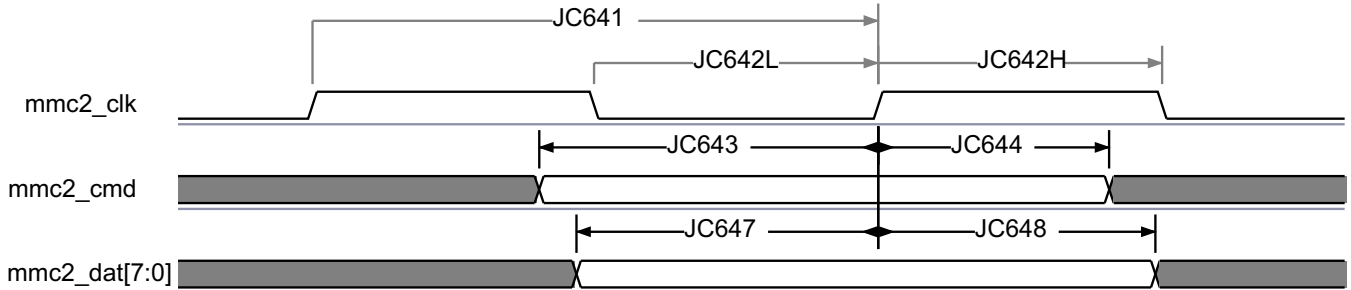
図 5-89. MMC/SD/SDIO in - High Speed JC64 - Receiver Mode
