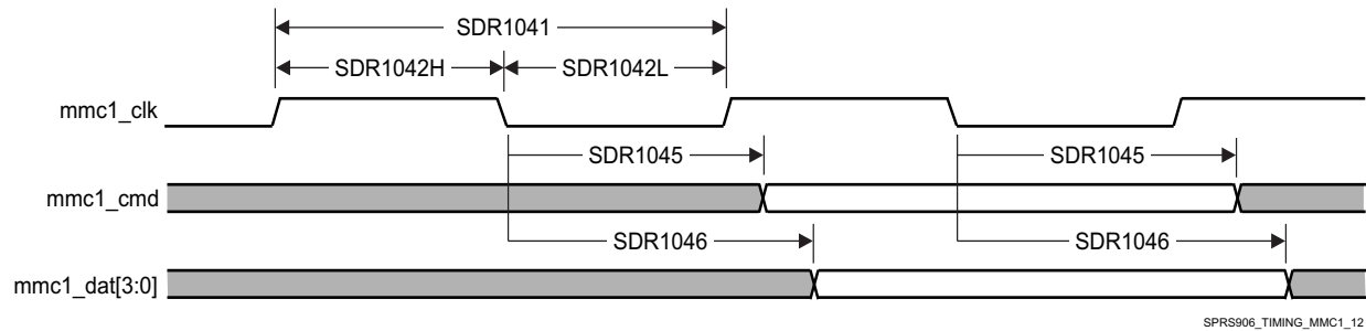
图 5-84. MMC/SD/SDIO in - High Speed SDR104 - Transmitter Mode
