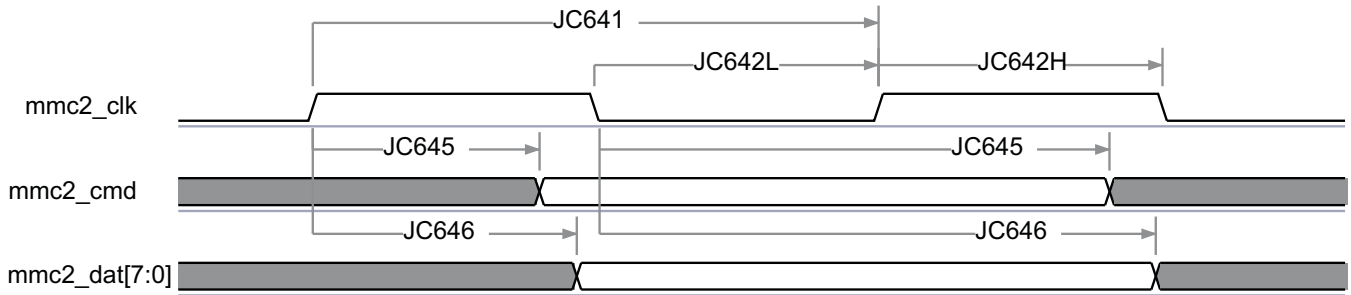
図 5-90. MMC/SD/SDIO in - High Speed JC64 - transmitter Mode
