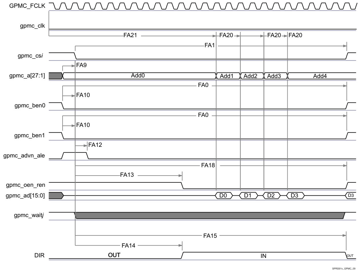
FIG 5-28. GPMC / NOR Flash - Asynchronous Read - Page Mode 4x16-bit Timing (1)(2)(3)(4)
