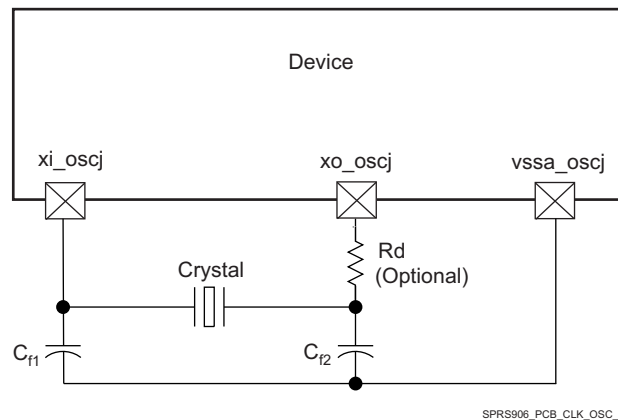
☒ 7-31. Grounding Scheme for High-Frequency Clock
