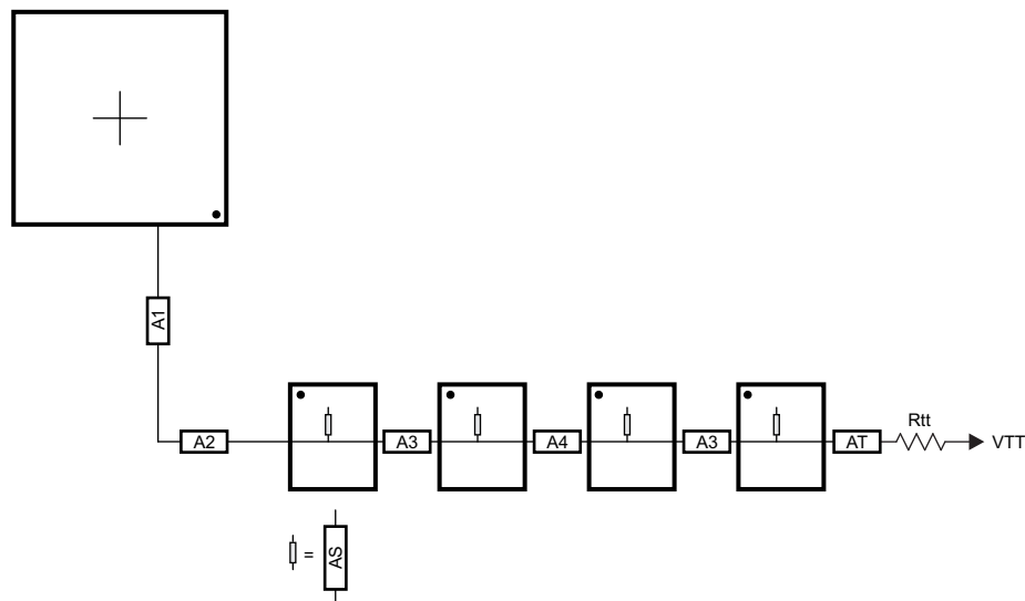
FIG 7-9. ADDR_CTRL Routing for Four Single-Side DDR3 Devices
