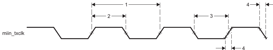
图 5-65. Clock Timing (GMAC Transmit) - MII operation
