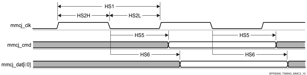
图 5-97. MMC/SD/SDIOj in - High Speed 3.3V Signaling - Transmitter Mode
