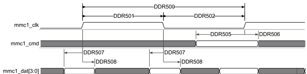
图 5-85. SDMMC - High Speed SD - DDR - Data/Command Receive
