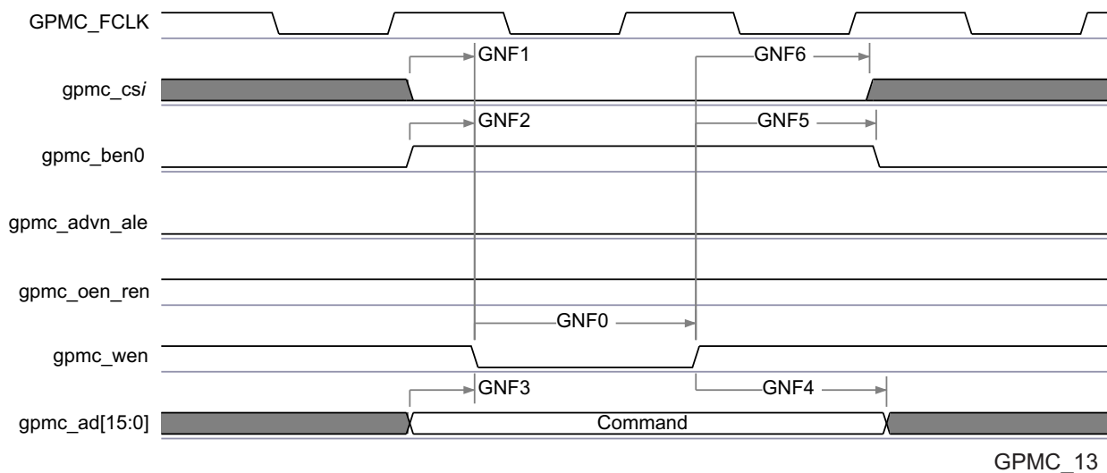
✎ 5-32. GPMC / NAND Flash - Command Latch Cycle Timing (1)
