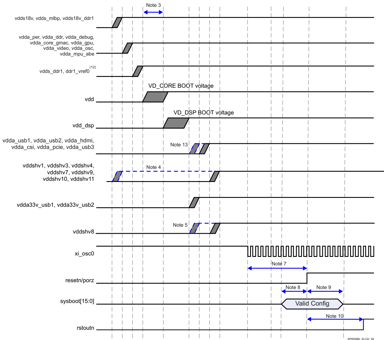
Figure 5-5. Power-Up Sequencing
