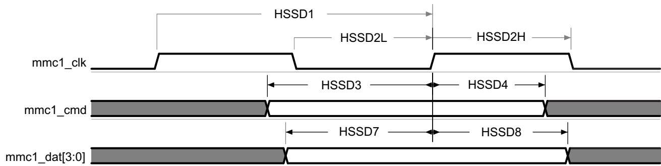
图 5-75. MMC/SD/SDIO in - High Speed - Receiver Mode
