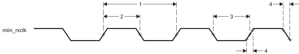
图 5-64. Clock Timing (GMAC Receive) - MII operation
