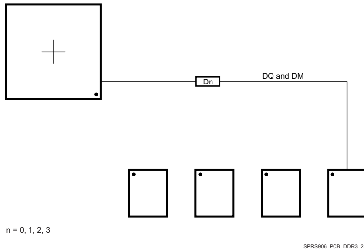
☒ 7-25. DQ/DM Routing With Any Number of Allowed DDR3 Devices
