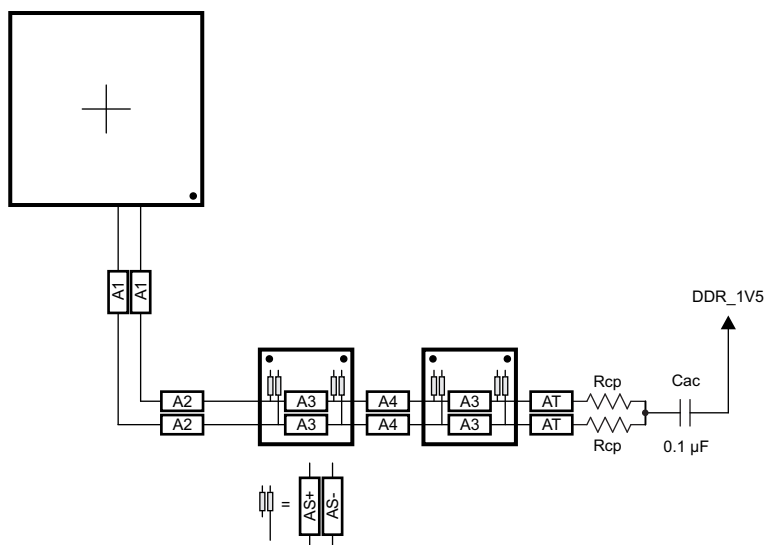
FIG 7-10. CK Routing for Four Mirrored DDR3 Devices
