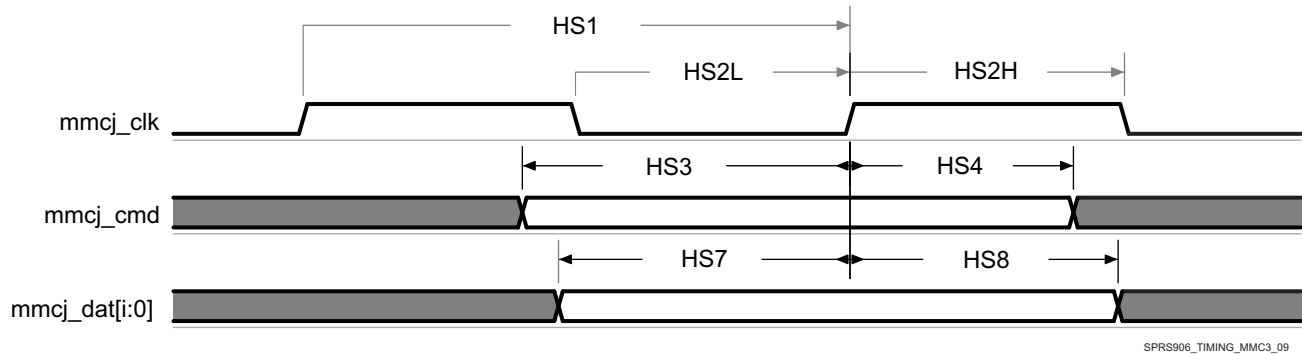
图 5-96. MMC/SD/SDIOj in - High Speed 3.3V Signaling - Receiver Mode
