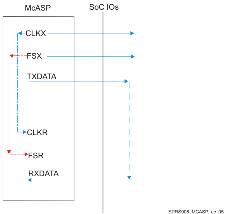
图 5-60. McASP1-8 CO-FO- – SYNC Mode
