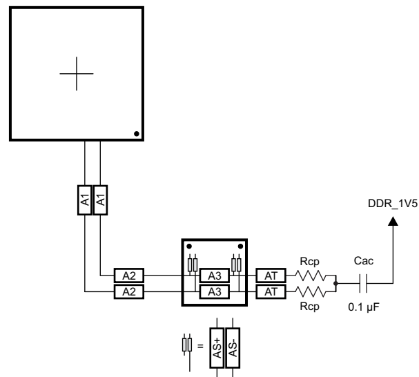
7-16. CK Routing for Two Mirrored DDR3 Devices
