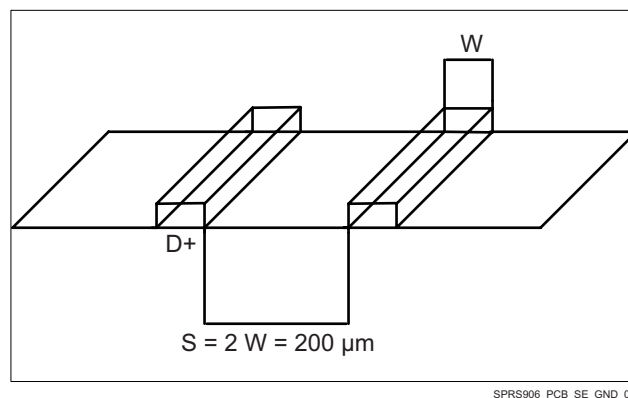
Figure 7-29. Ground Guard Illustration
