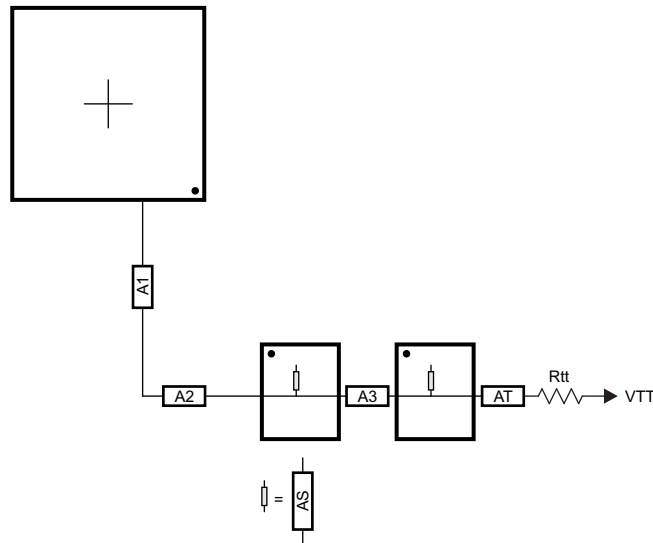
7-15. ADDR_CTRL Routing for Two Single-Side DDR3 Devices
