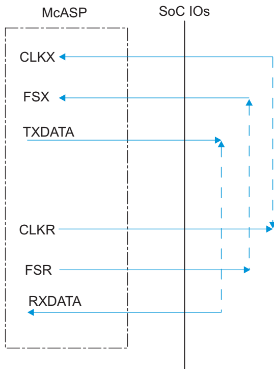
FIG 5-58. McASP1-8 CIOFIO – ASYNC Mode
