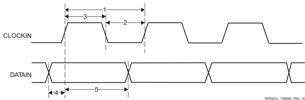
図 5-106. PRU-ICSS PRU Parallel Capture Timing - Rising Edge Mode
