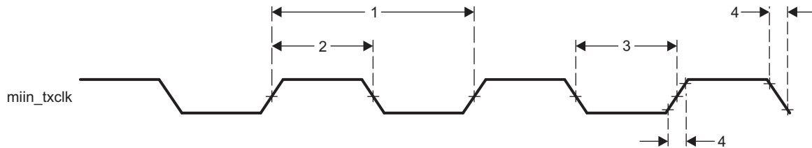
图 5-65. Clock Timing (GMAC Transmit) - MII operation
