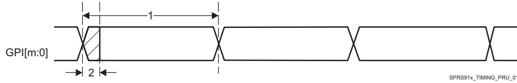
図 5-104. PRU-ICSS PRU Direct Input Timing
