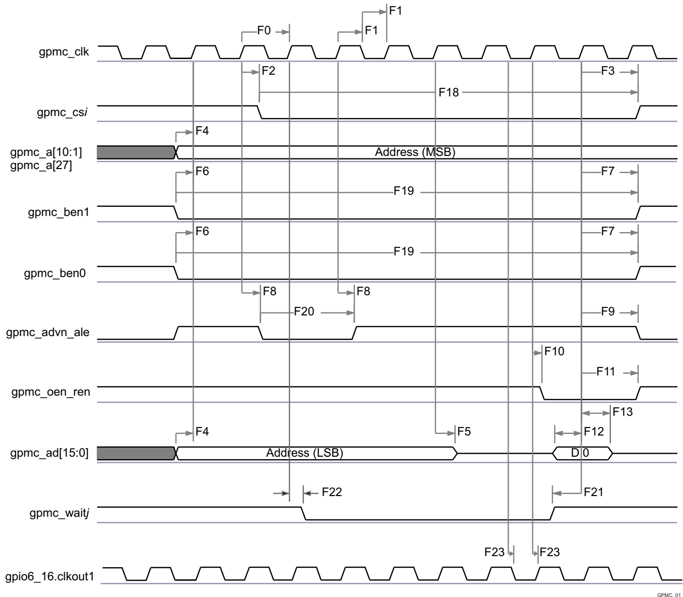
FIG 5-20. GPMC / Multiplexed 16bits NOR Flash - Synchronous Single Read - (GpmcFCLKDivider = 0) (1)(2)
