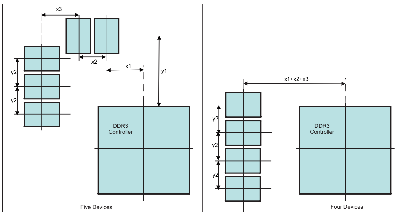
Figure 8-4. Placement Specifications
