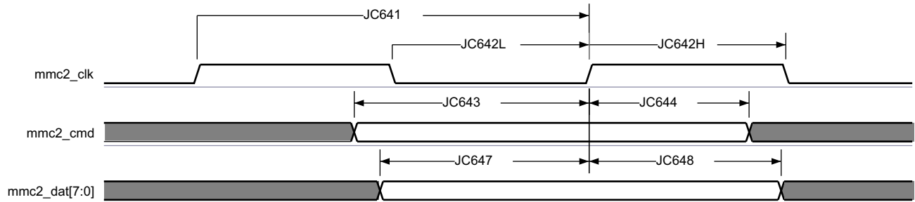
Figure 7-77. MMC/SD/SDIO in - High Speed JC64 - Receiver Mode
