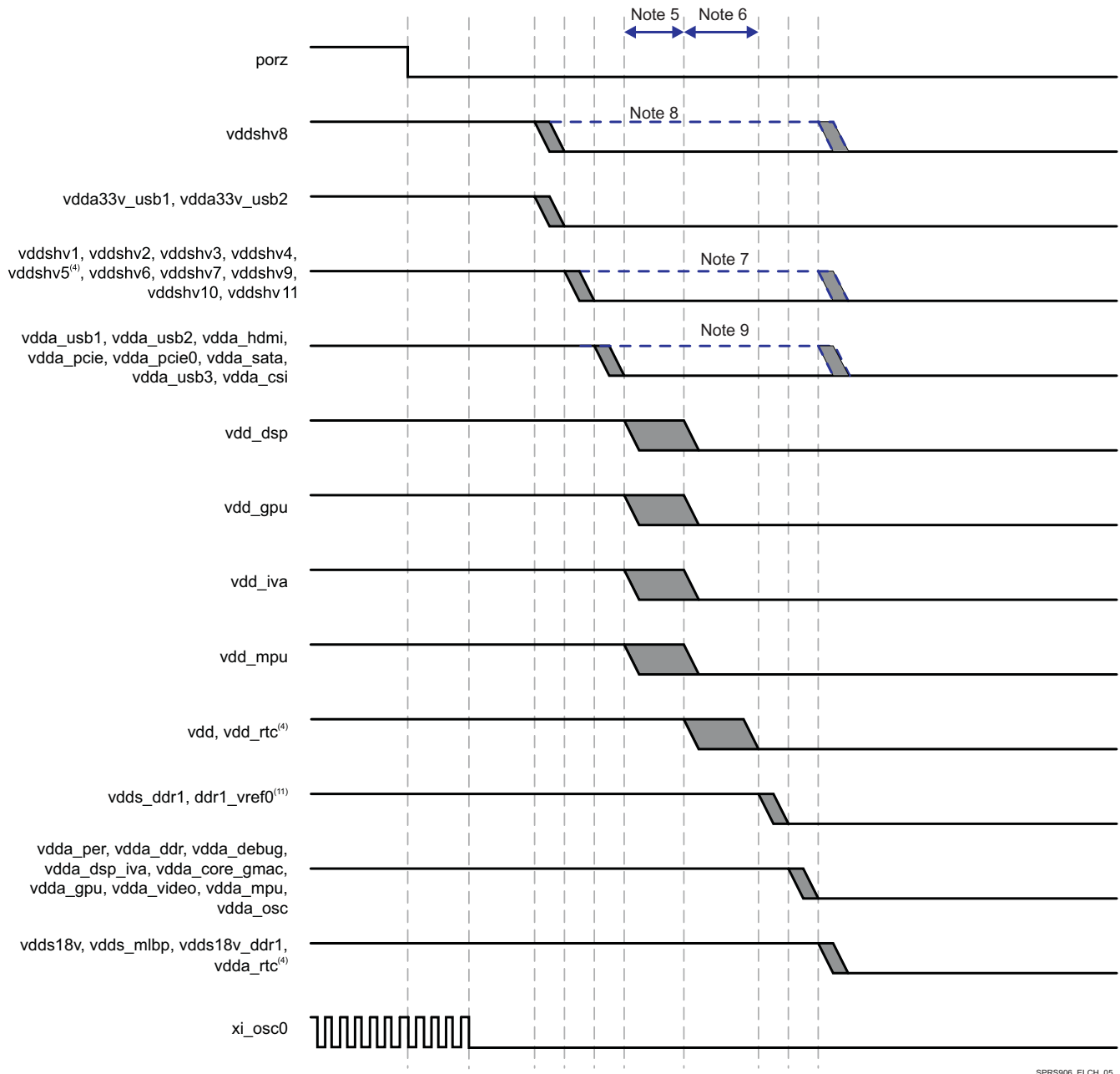
Figure 5-3. Power-Down Sequencing (10)(12)
