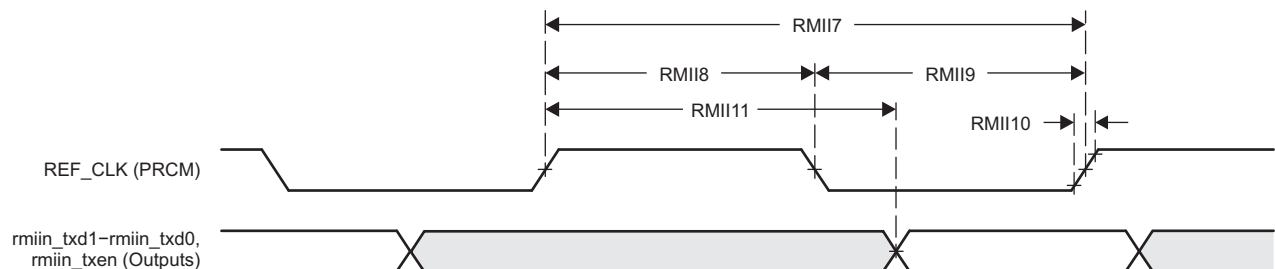
Figure 7-58. GMAC Transmit Interface Timing RMIIIn Operation
