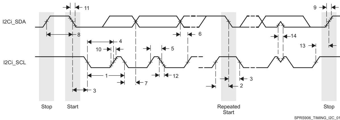
Figure 7-23. I2C Receive Timing
