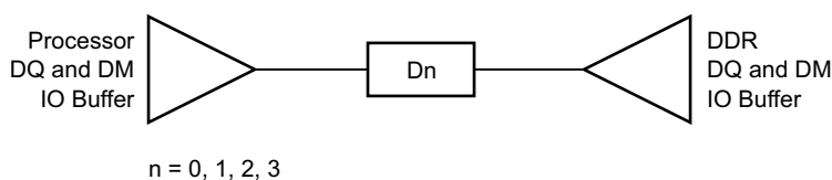
Figure 8-23. DQ/DM Topology
