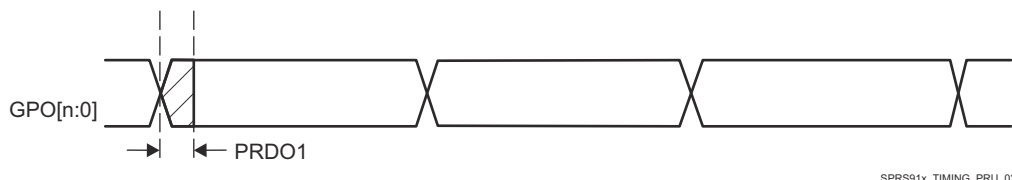
図 6-95. PRU_ICSSG PRU Direct Output Timing
