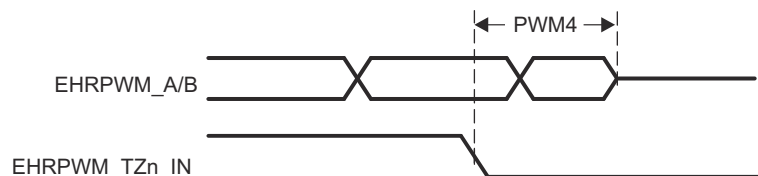
图 6-46. EHRPWM_TZn_IN to EHRPWM_A/B Hi-Z Switching Characteristics
