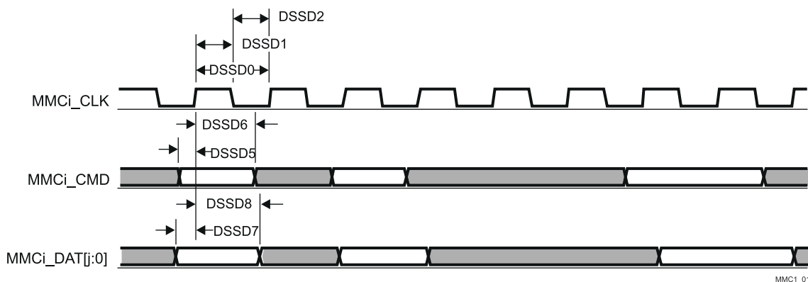
図 6-72. eMMC/SD/SDIO in - Default Speed - Receiver Mode
