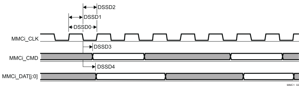
図 6-73. eMMC/SD/SDIO in - Default Speed - Transmitter Mode
