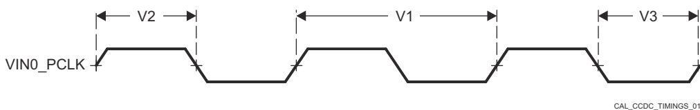
図 6-30. LVDSRX Input Clock Signal
