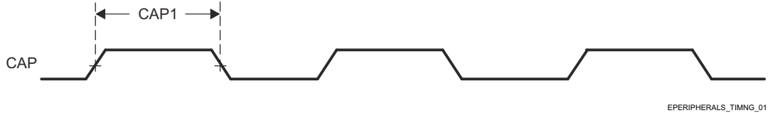
図 6-41. eCAP Timing Requirements
