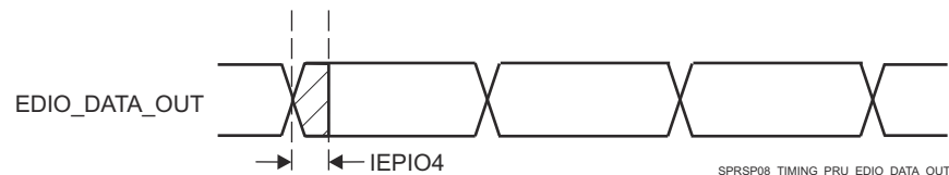
図 6-106. PRU_ICSSG PRU IEP Digital IOs Timing
