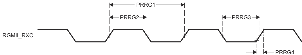
図 6-114. PRU_ICSSG RGMII_RCLK Timing Requirements
