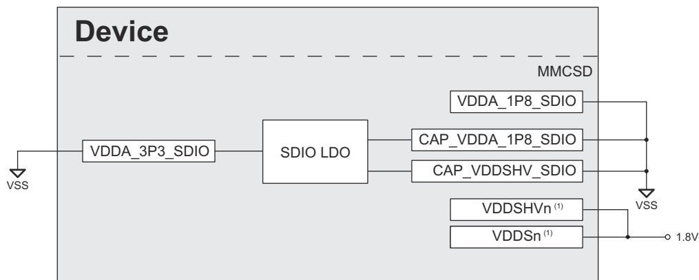
図 8-10. VDDSHV6 or VDDSHV7 Used as the MMCSD Supply for Fixed 1.8V IO
