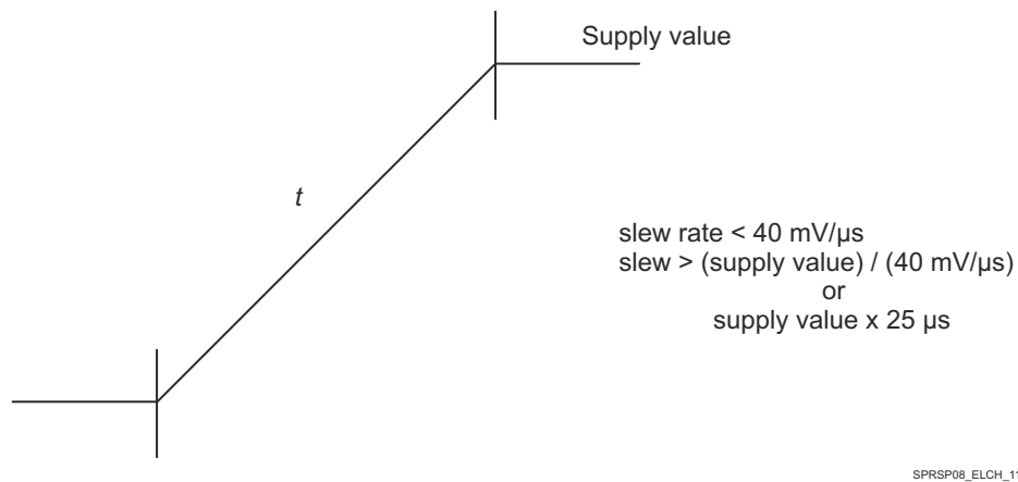
図 6-3. VDDA_1P8_SERDES0 Supply Slew and Slew Rate
