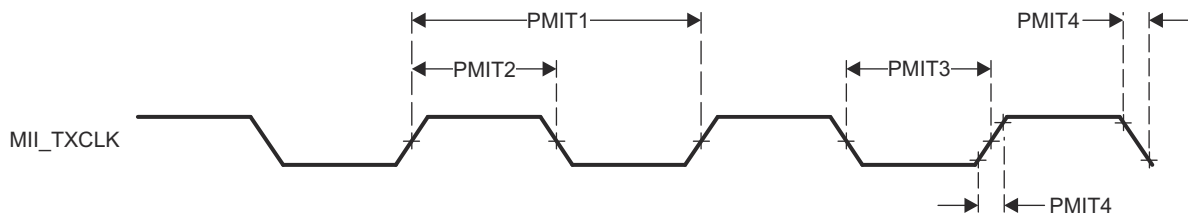
图 6-120. PRU_ICSSG MII_TX_CLK Switching Characteristics
