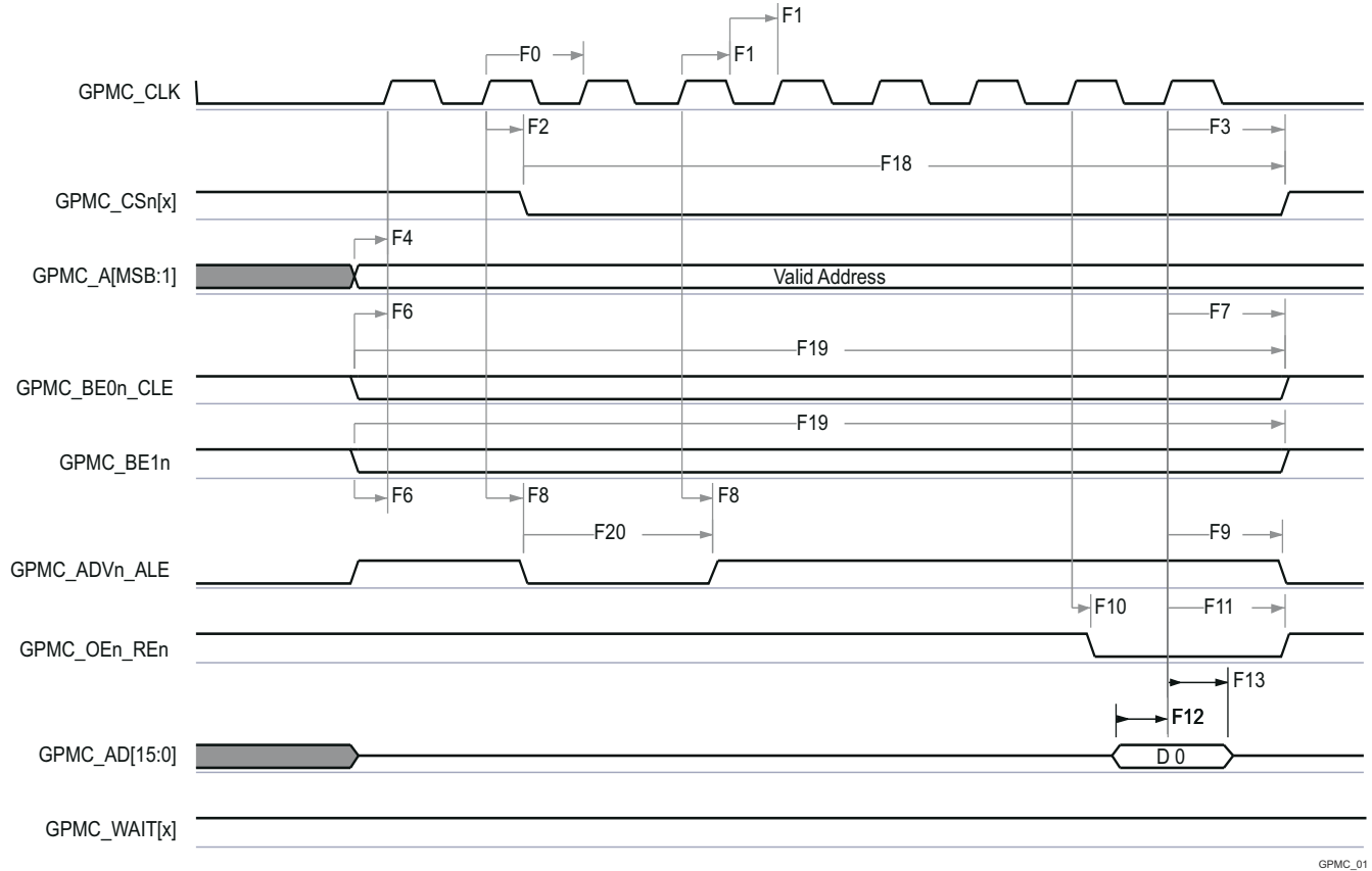
6-48. GPMC and NOR Flash—Synchronous Single Read—(GpmcFCLKDivider = 0)
