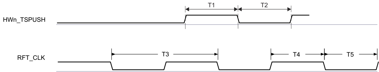
6-84. CPTS Input Timing
