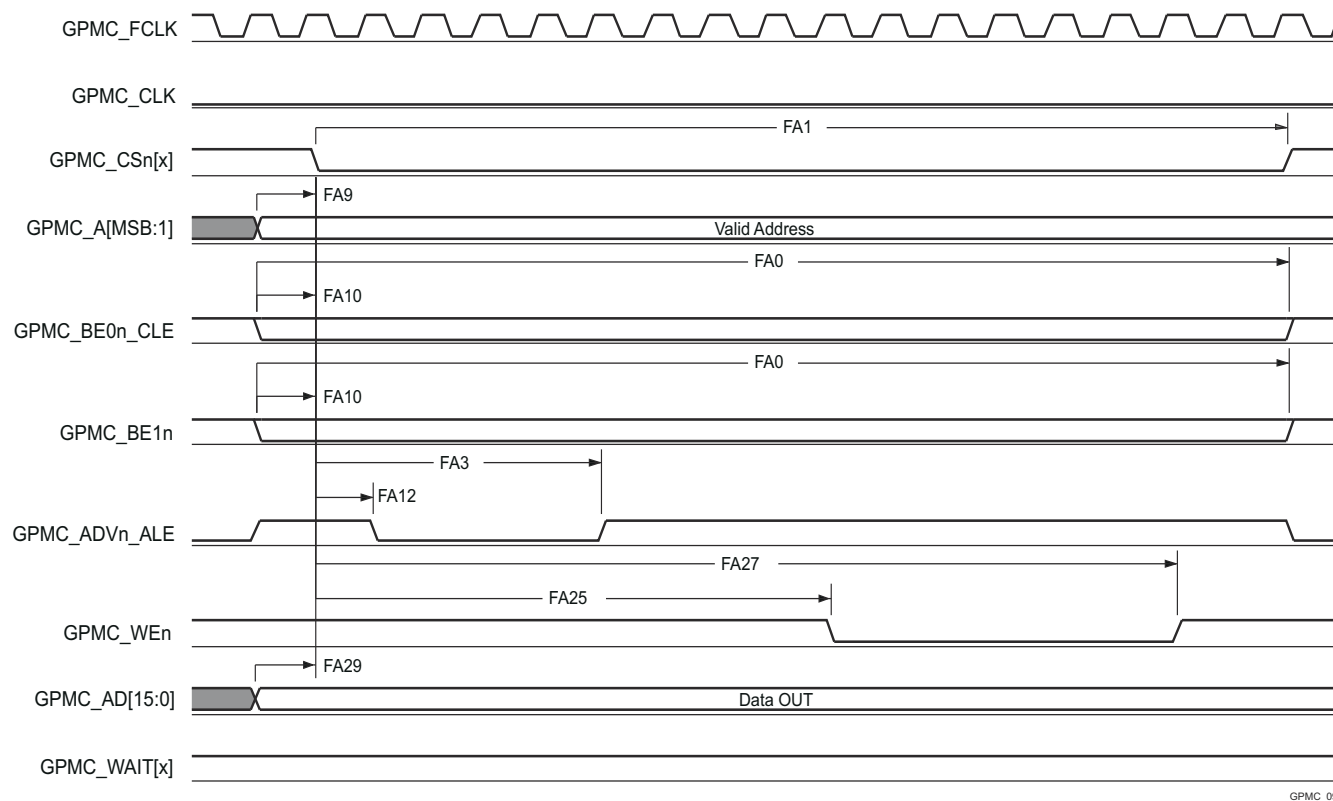
図 6-56. GPMC and NOR Flash—Asynchronous Write—Single Word
