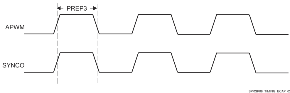
図 6-110. PRU_ICSSG ECAP Switching Characteristics
