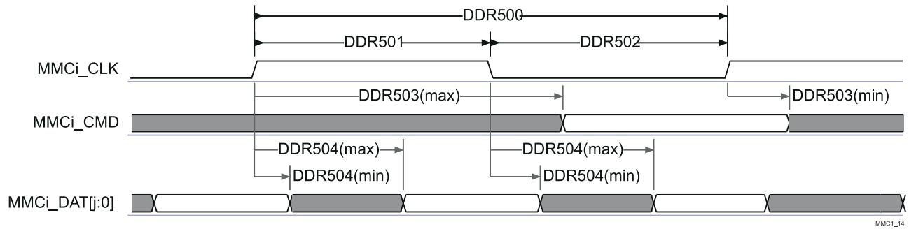
図 6-81. eMMC/SD/SDIO - High-Speed DDR - DDR50 - Transmit Mode
