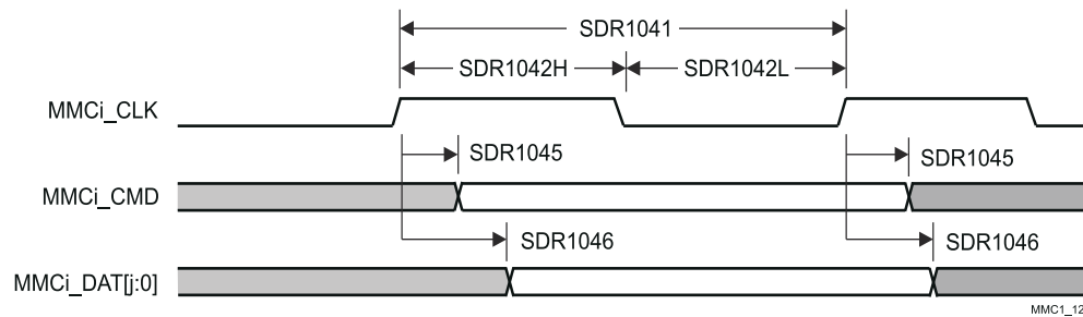
図 6-83. eMMC/SD/SDIO in - High Speed SDR104, HS200 - Transmitter Mode
