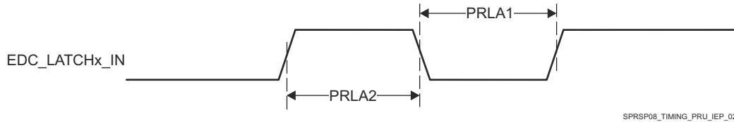
図 6-107. PRU_ICSSG PRU IEP LATCHx_IN Timing
