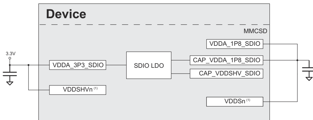
図 8-10. VDDSHV6 or VDDSHV7 Used as the MMCSD Supply for Fixed 1.8V IO
