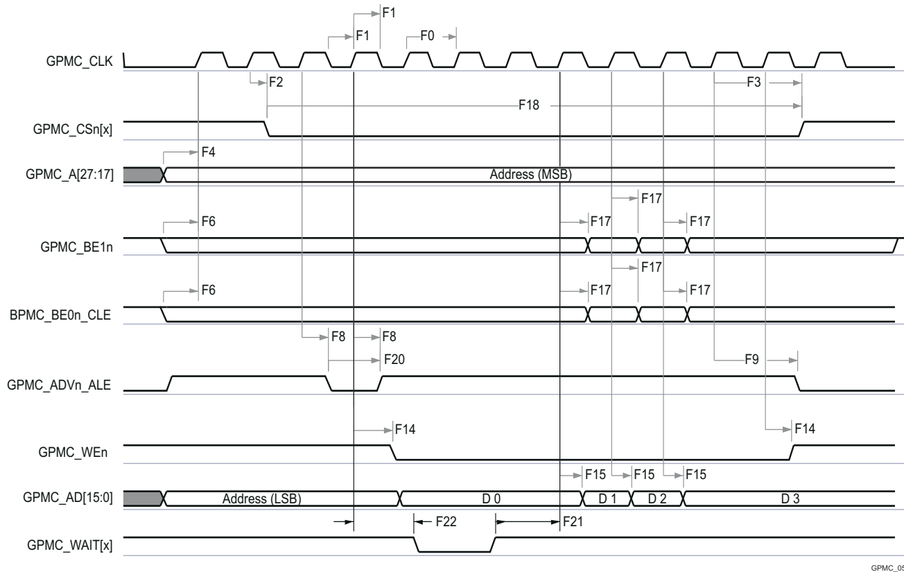
6-51. GPMC and Multiplexed NOR Flash—Synchronous Burst Read
