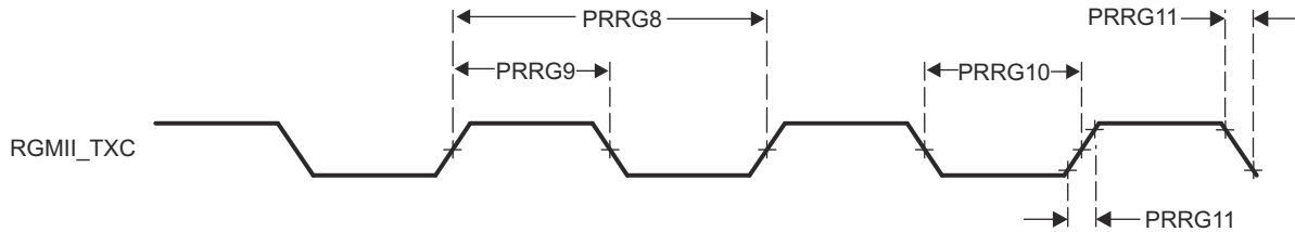
6-116. PRU_ICSSG RGMII_TXC Switching Characteristics
