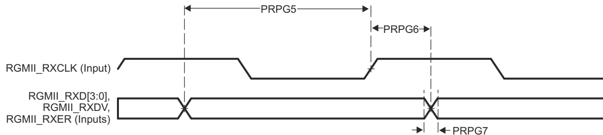
図 6-115. PRU_ICSSG RGMII_RD[3:0] and RGMII_RX_CTL Timing Requirements
