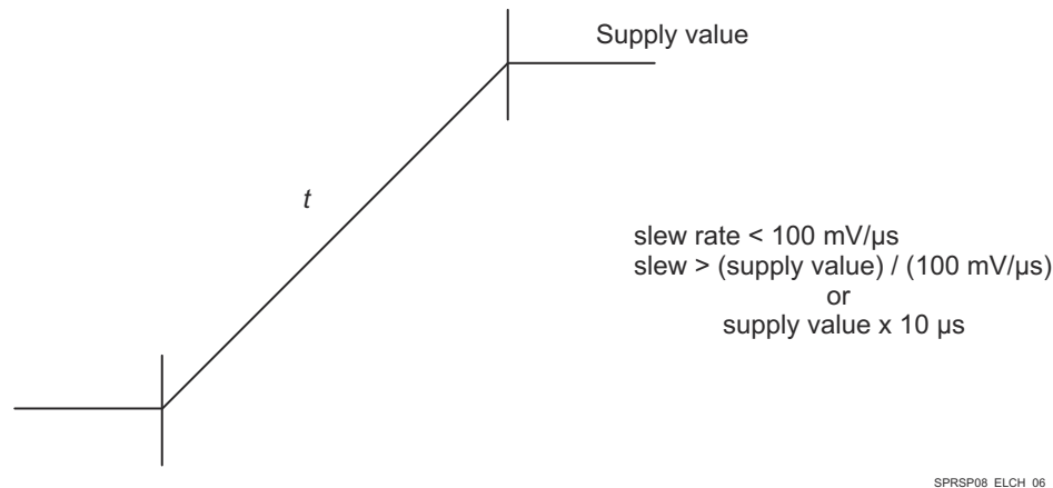
図 6-2. Power Supply Slew and Slew Rate
