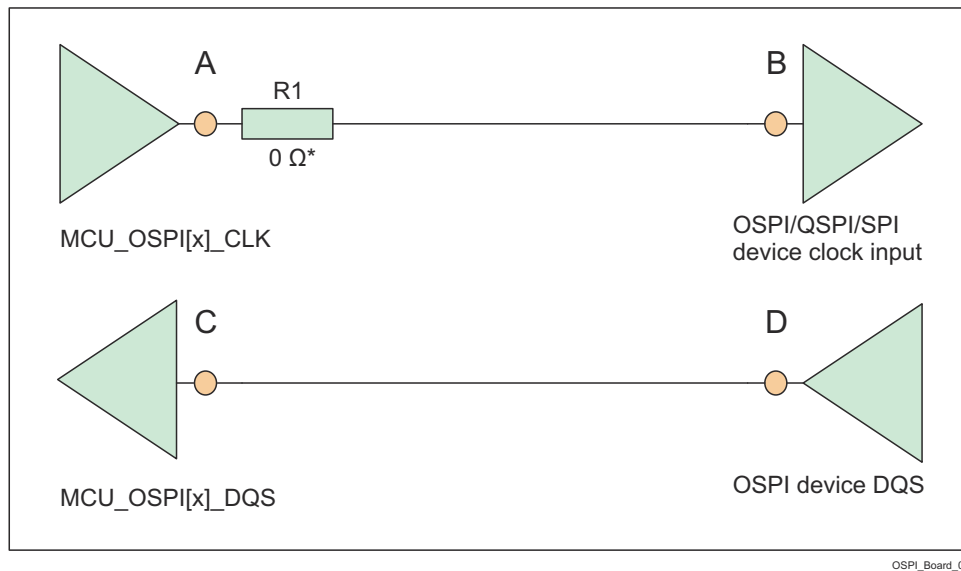
図 8-3. OSPI Interface High Level Schematic
