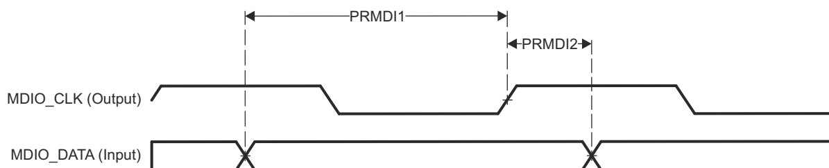
図 6-111. PRU_ICSSG MDIO_DATA Timing – Input Mode
