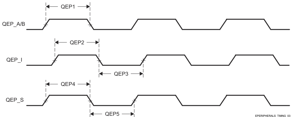
図 6-47. eQEP Timing Requirements
