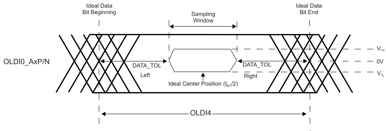
図 6-91. OLDI Output Pulse Positions
