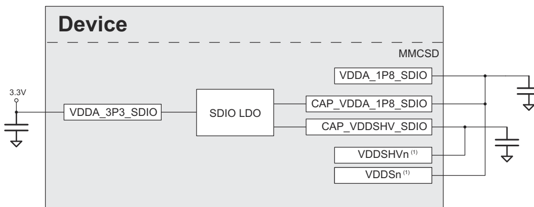
図 8-11. VDDSHV6 or VDDSHV7 Used as the MMCSD Supply for Fixed 3.3V IO
