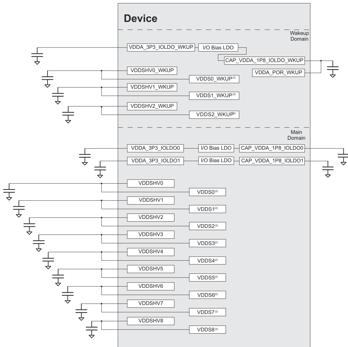
図 8-8. All VDDSHV[8:0] and VDDSHV[2:0]_WKUP Supplies Configured for 1.8V Operation
