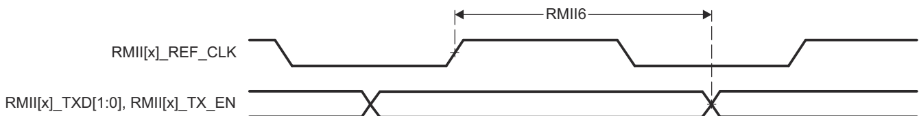
図 6-35. RMII[x]_TXD[1:0], and RMII[x]_TX_EN Switching Characteristics – RMII Mode
