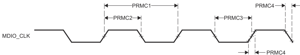
図 6-112. PRU_ICSSG MDIO_CLK Switching Characteristics
