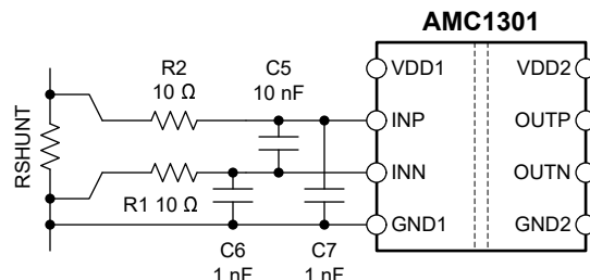
図 8-2. Differential Input Filter
