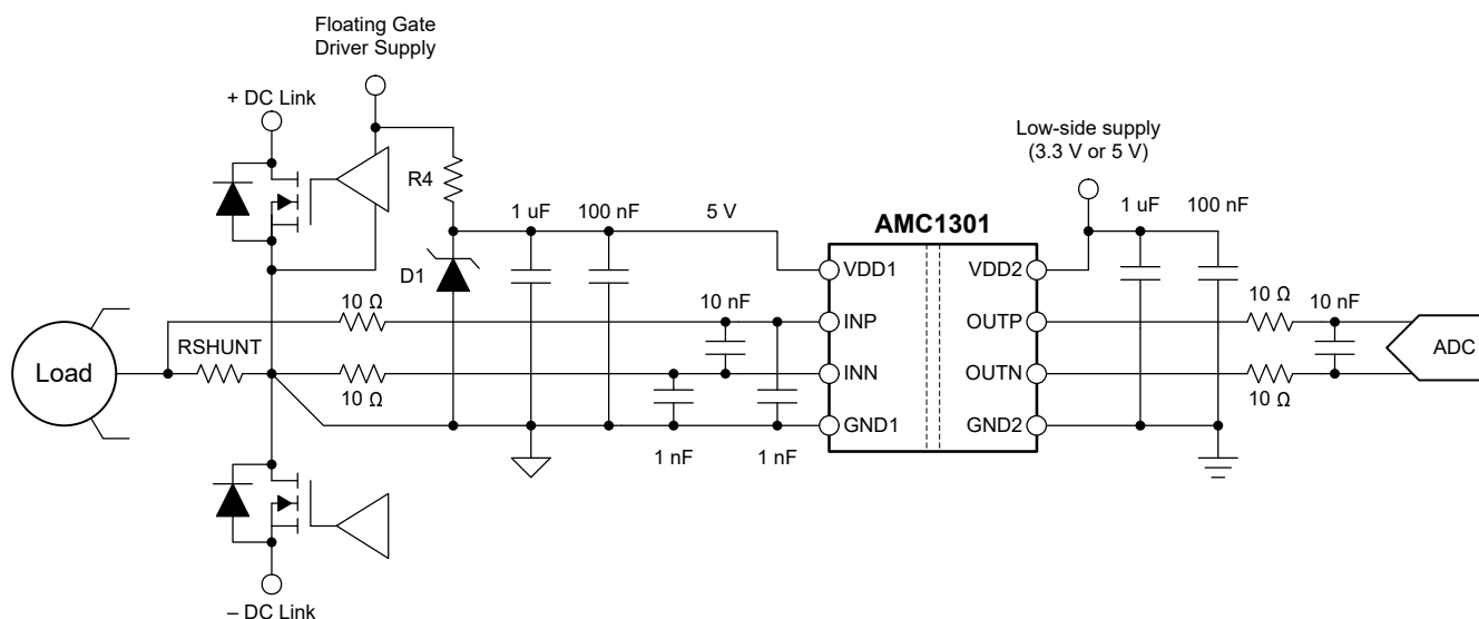
■ 8-1. Using the AMC1301 for Current Sensing in a Typical Application
