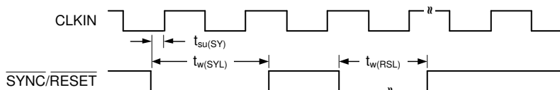
図 6-2. SYNC/RESET Timing Requirements
