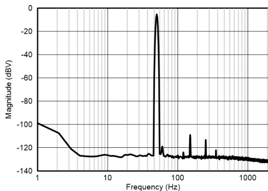
図 6-14. Frequency Spectrum With 50-Hz Input Signal
