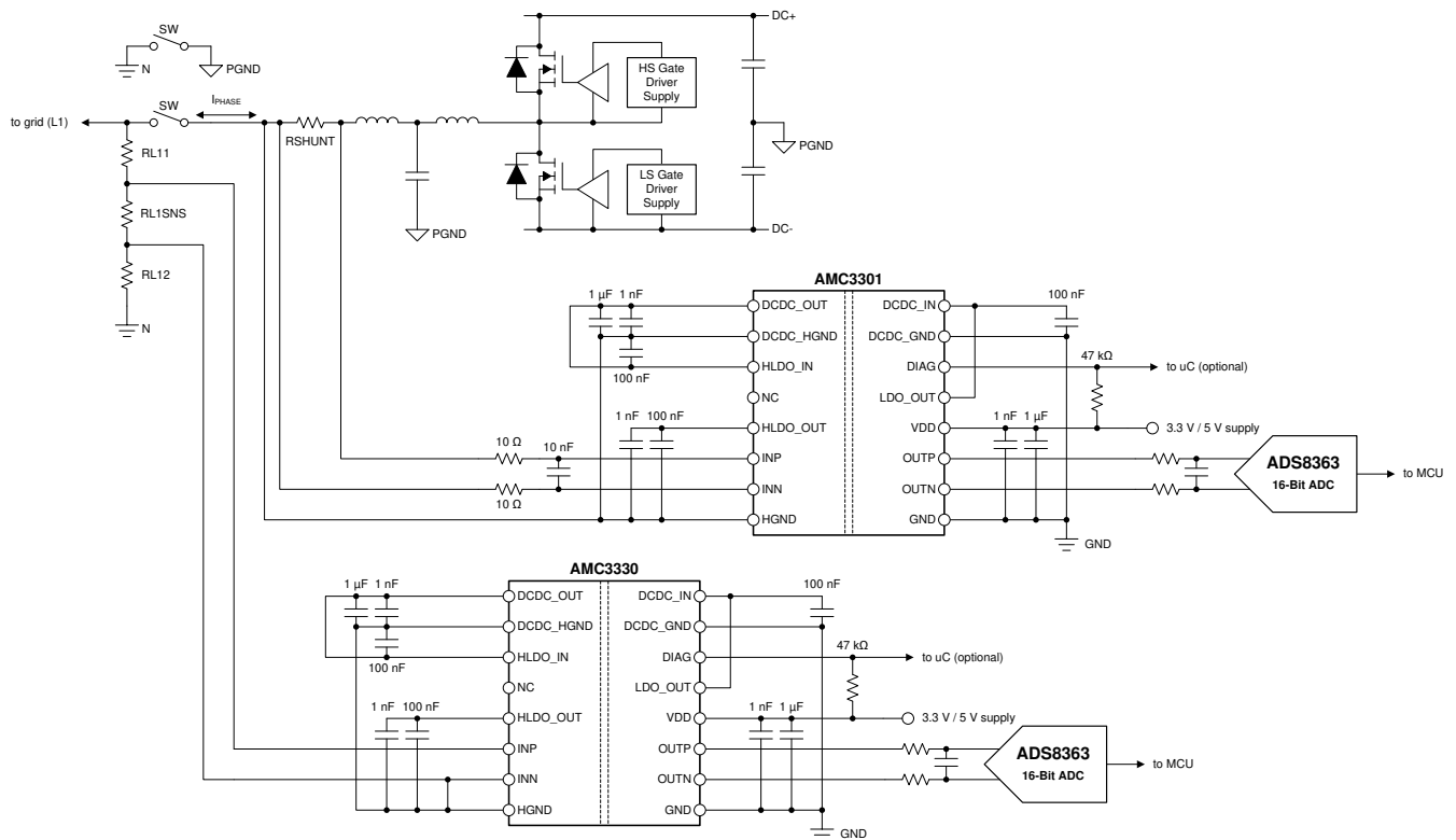
図 7-1. The AMC3301 in a Solar Inverter Application
