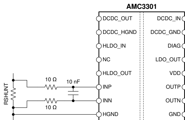
図 7-2. Differential Input Filter
