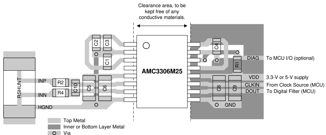
☒ 10-1. Recommended Layout of the AMC3306M25
