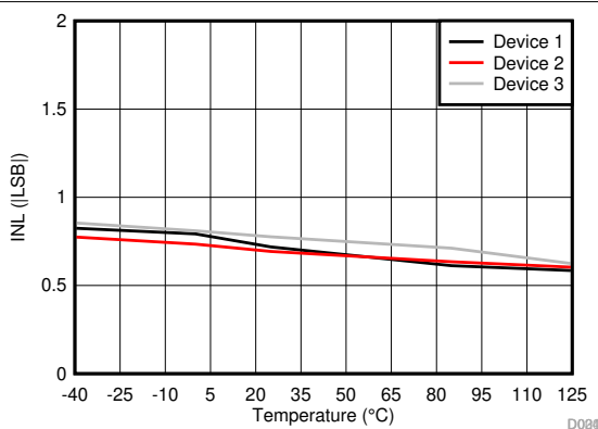
FIG 6-18. Integral Nonlinearity vs Temperature
