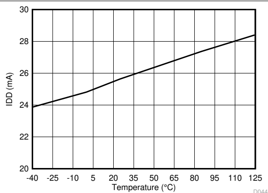
Figure 6-40. Supply Current vs Temperature
