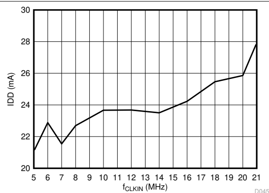
Figure 6-39. Supply Current vs Input Clock Frequency
