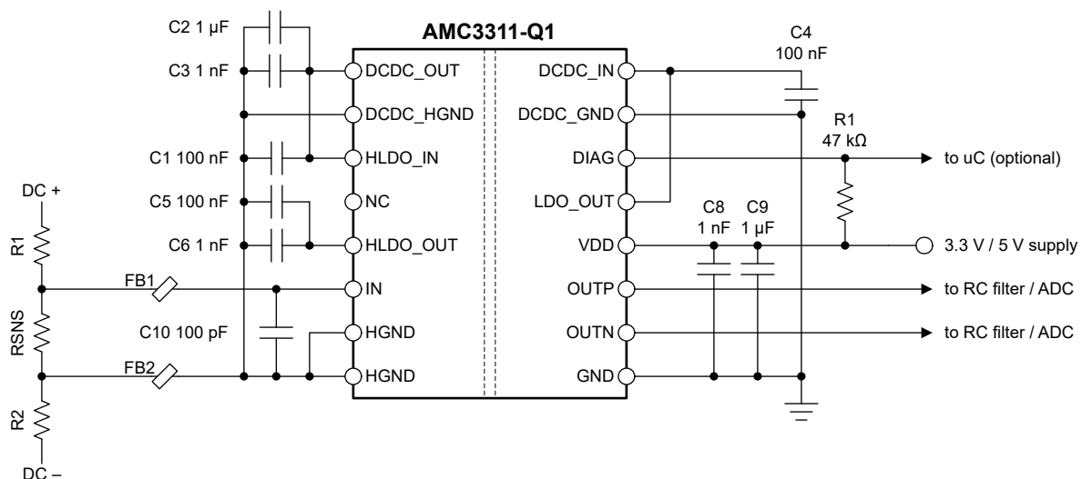
Figure 8-5. Decoupling the AMC3311-Q1
