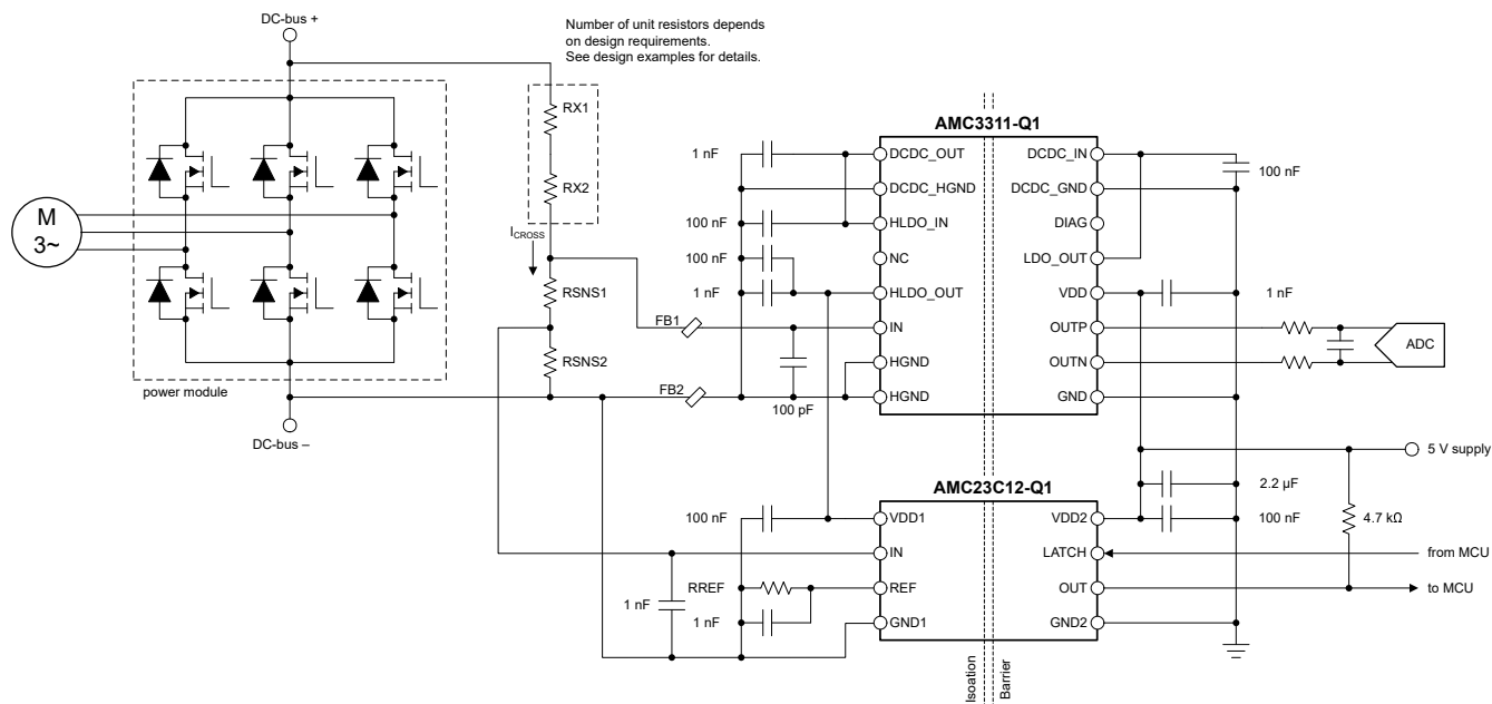
8-1. The AMC3311-Q1 in a Traction Inverter Application
