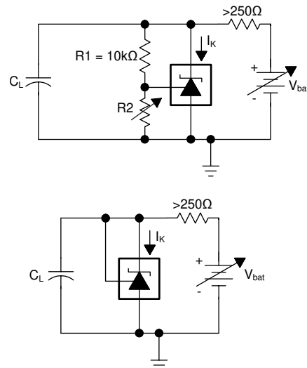
图 6-6. Test Circuit for Stability Boundary Conditions
