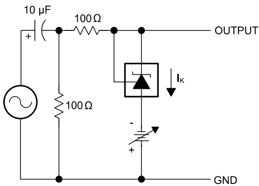
图 6-5. Test Circuit for Reference Impedance ( Z_{KA} )
