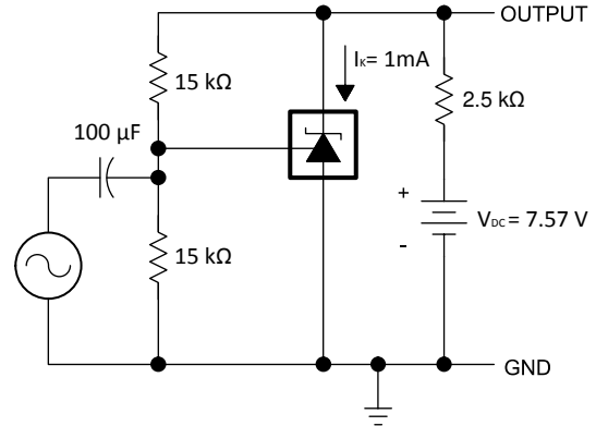
图 6-4. Test Circuit for Phase and Gain Measurement
