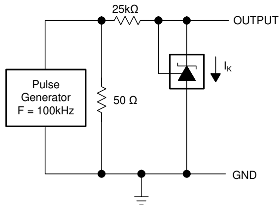
图 6-7. Test Circuit for Pulse Response
