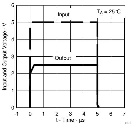
Figure 11. Pulse Response
