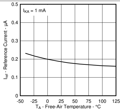
FIG 2. Reference Current versus Free-Air Temperature
