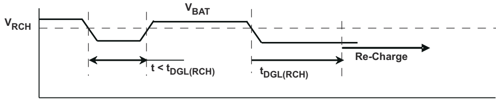
FIG 9-12. Recharge – t_{DGL(RCH)}
