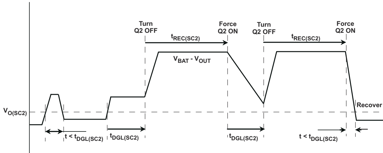
FIG 9-13. OUT Short-Circuit – Supplement Mode
