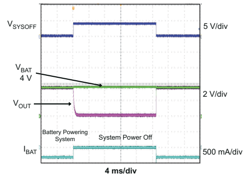
图 10-11. System ON/OFF With Input Not Connected V_{IN} = 0 V BQ24075, BQ24079
