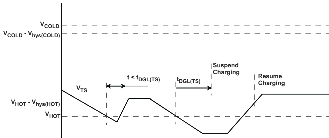
FIG 9-14. Battery Pack Temperature Sensing – TS Pin. Battery Temperature Increasing
