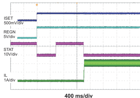
図 8-2. Charge Enable by ISET
