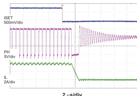
図 8-4. Charge Disable by ISET
