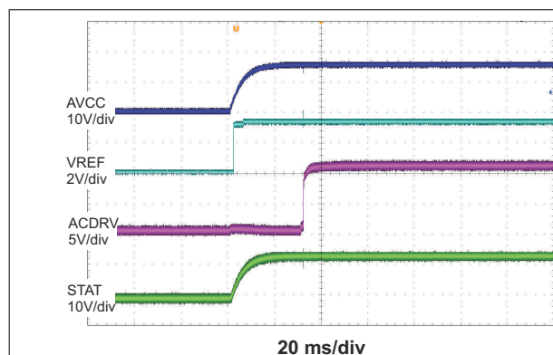
図 8-1. Power Up (ISET = 0)
