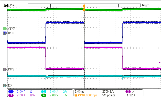
10-17. System Load Transient
