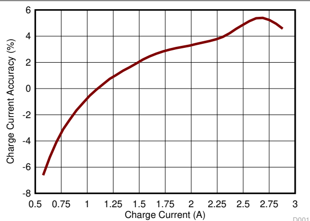
8-4. Charge Current Accuracy
