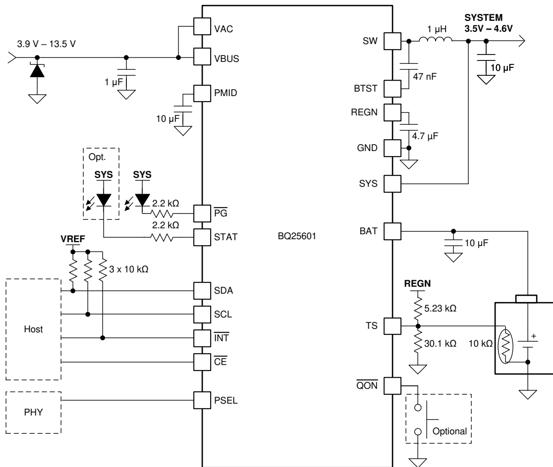
図 10-1. Power Path Management Application
