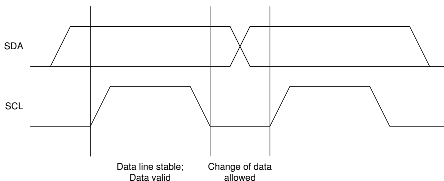
FIG 9-12. Bit Transfer on the I 2 C Bus
