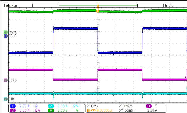
10-15. System Load Transient
