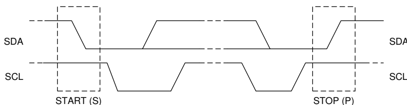
FIG 9-13. TS START and STOP conditions
