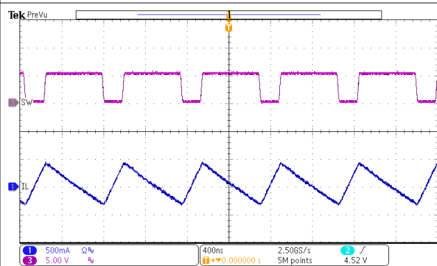
10-11. OTG Switching
