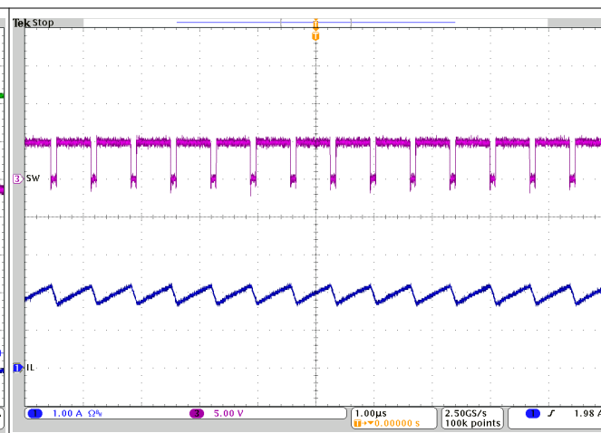
10-7. PWM Switching in Buck Mode
