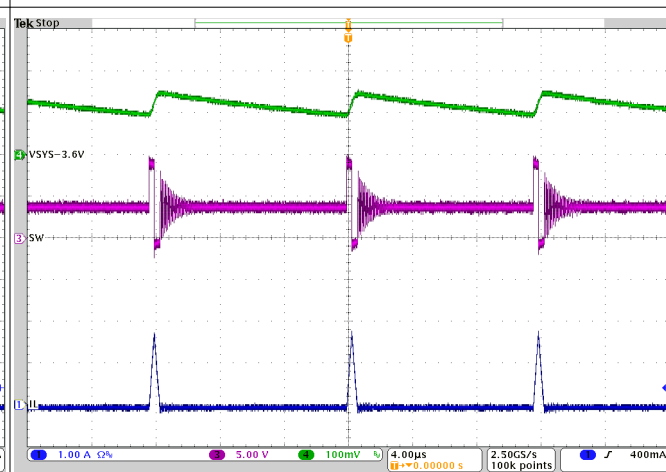
10-3. Power Up with Charge Enabled
