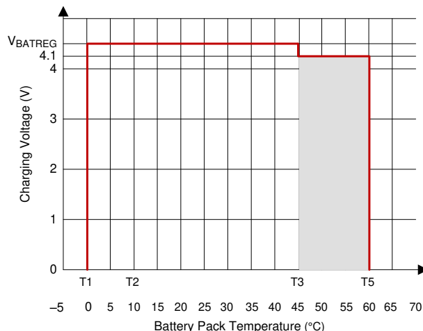
图 9-3. JEITA Profile: Charging Voltage
