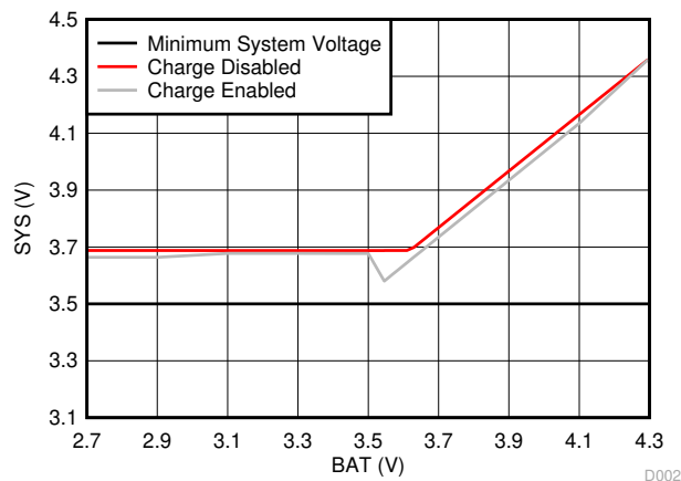
FIG 9-1. System Voltage vs Battery Voltage
