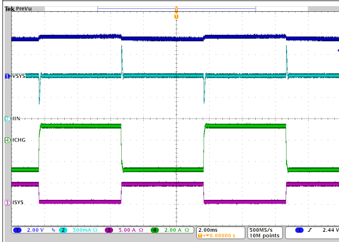
10-14. System Load Transient
