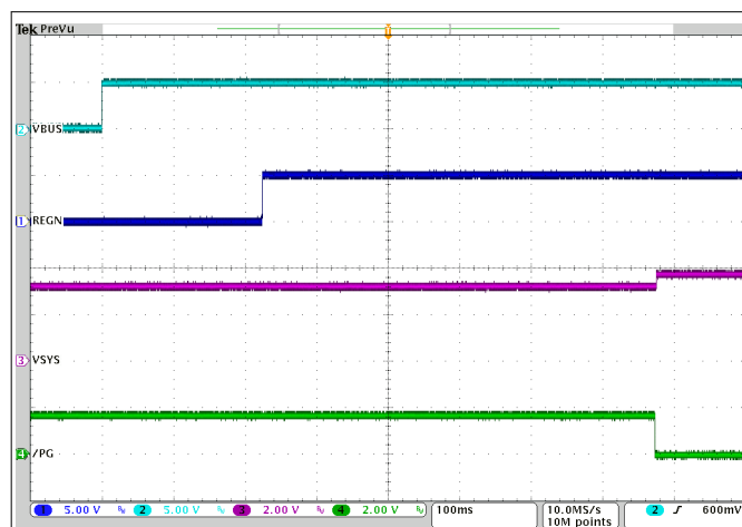
10-2. Power Up with Charge Disabled
