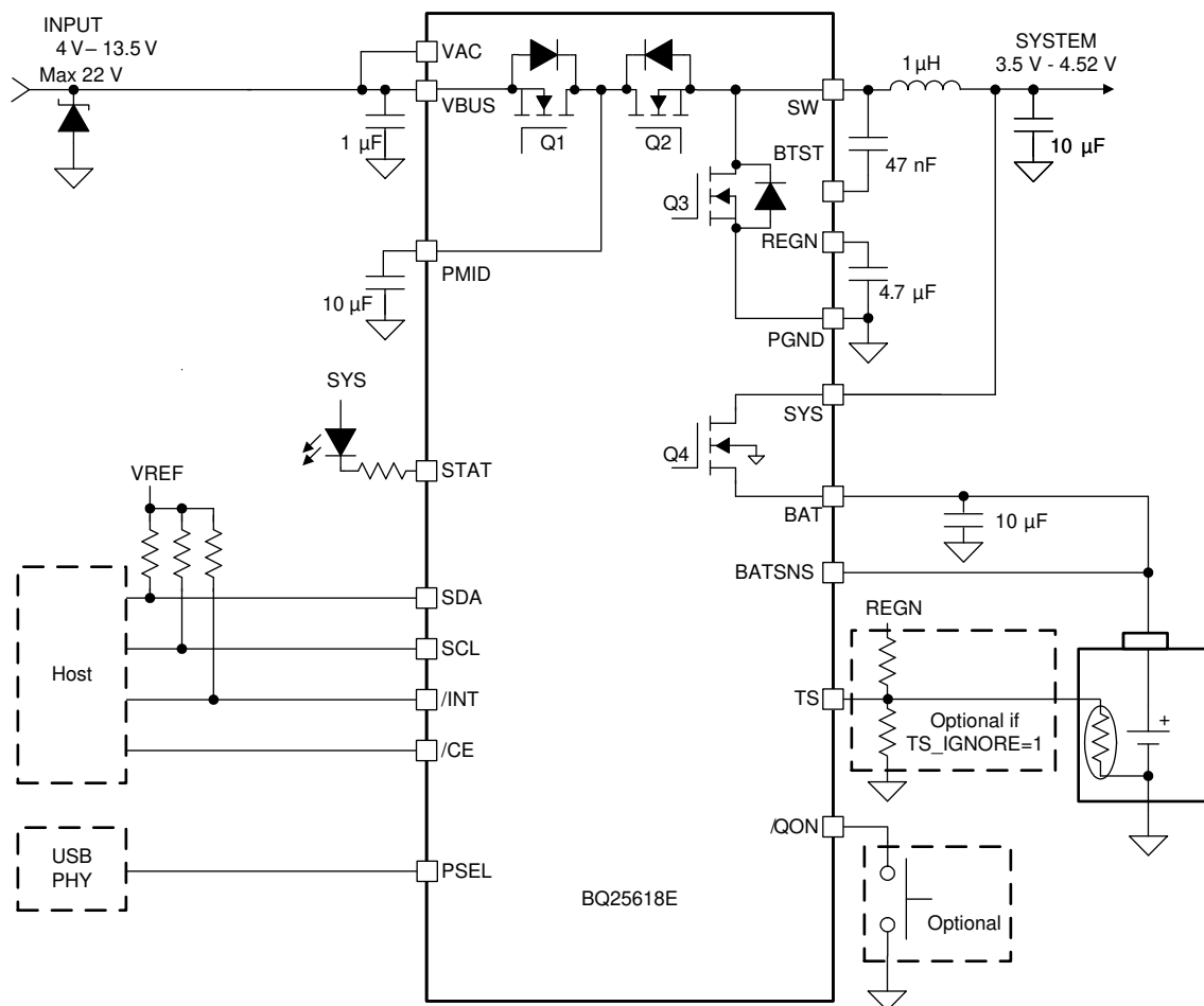
Figure 9-1. BQ25618E Application Diagram
