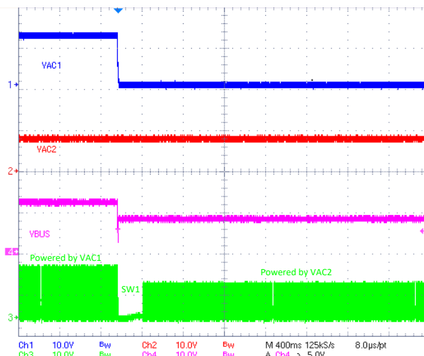
图 8-5. Input Source Auto Transition from VAC1 to VAC2 when VAC1 is Gone
