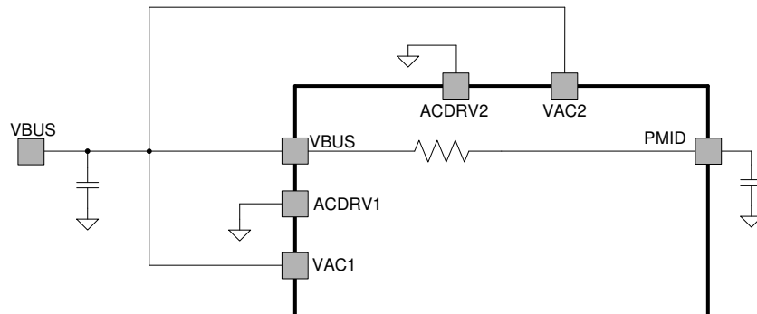
✎ 8-2. Single Input Connected to VBUS Directly Without ACFET-RBFET
