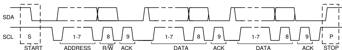
FIG 8-19. Complete Data Transfer on the I 2 C Bus
