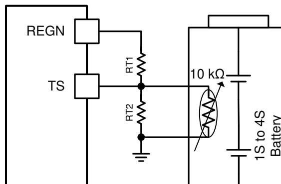
FIG 8-12. TS Resistor Network
