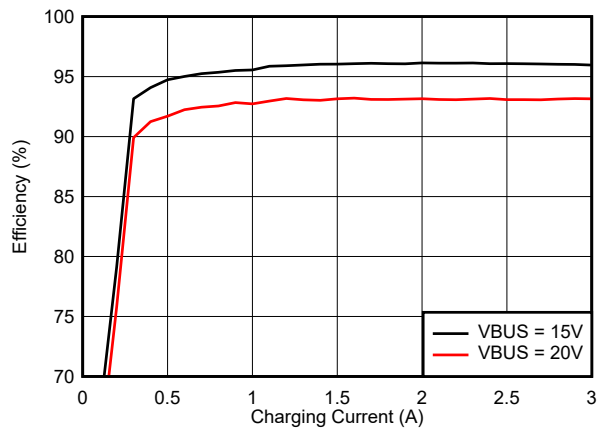
Figure 7-3. 2s Battery Charge Efficiency, 750 kHz
