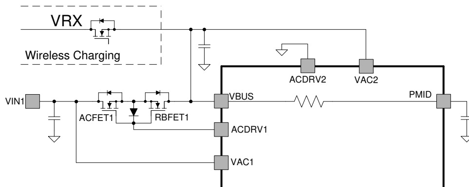
✎ 8-3. One ACFET-RBFET Structure Supporting One Input at VAC1 and/or One Input at VBUS
