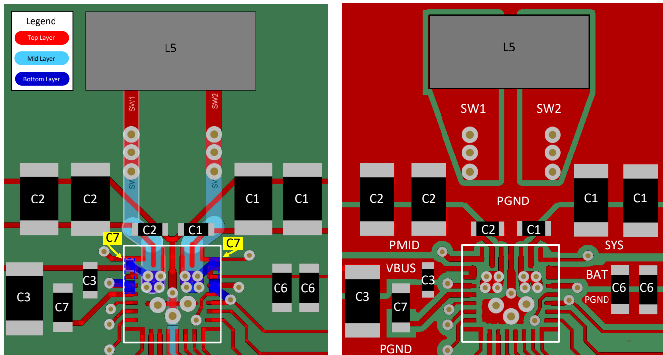
図 11-2. PCB Layout Example (Top Layer Copper Pours Removed on Left, Shown on Right)
