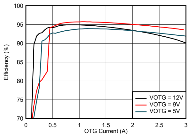
Figure 7-10. 1s Battery OTG Efficiency, 1.5 MHz
