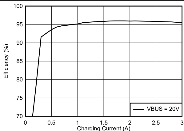
Figure 7-8. 4s Battery Charge Efficiency, 1.5 MHz
