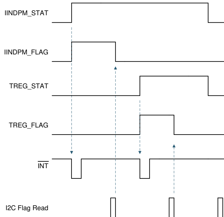
FIG 8-14. \overline{\text{INT}} Generation Behavior Example
