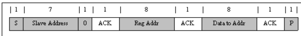
FIG 9-8. Single Write
