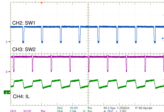
10-11. Switching During Buck Boost Mode
