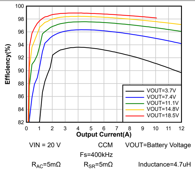
Figure 8-4. Charge Efficiency
