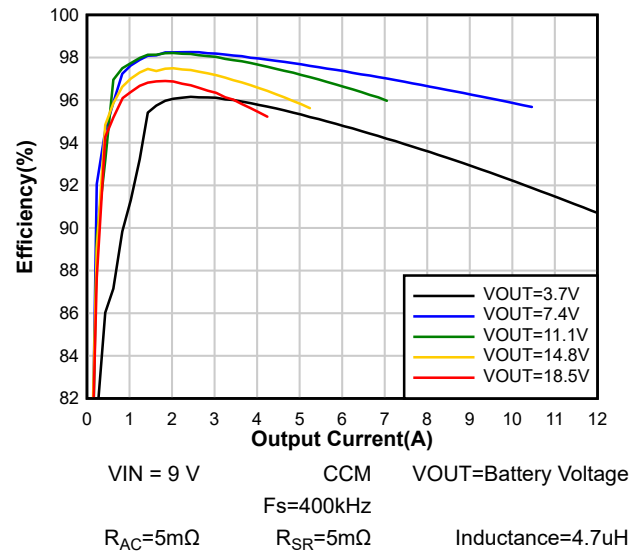
Figure 8-2. Charge Efficiency
