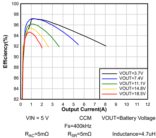
Figure 8-1. Charge Efficiency
