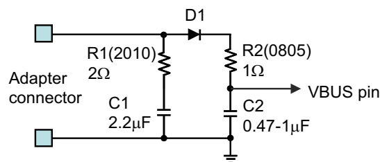
Figure 10-2. Input Filter
