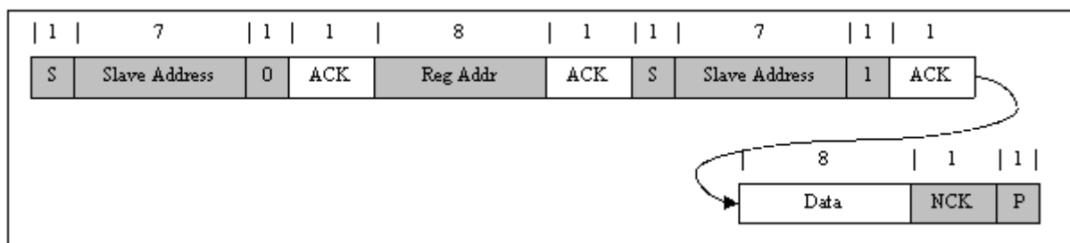
FIG 9-13. Single Read
