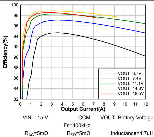
Figure 8-3. Charge Efficiency
