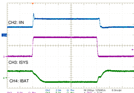
10-10. Switching During Boost Mode
