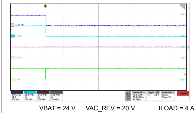
图 9-15. Reverse Mode Power Down with 4-A Load
