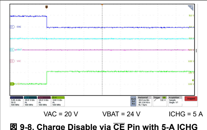
9-8. Charge Disable via \overline{\text{CE}} Pin with 5-A ICHG
