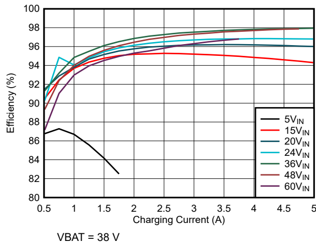
7-3. Charge Efficiency vs Charge Current (10s battery configuration)
