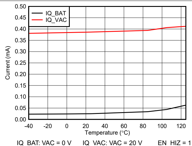
IQ_BAT: VAC = 0 V IQ_VAC: VAC = 20 V EN_HIZ = 1 Figure 7-6. Battery and Input Quiescent Current vs Temperature with VBAT = 28 V
