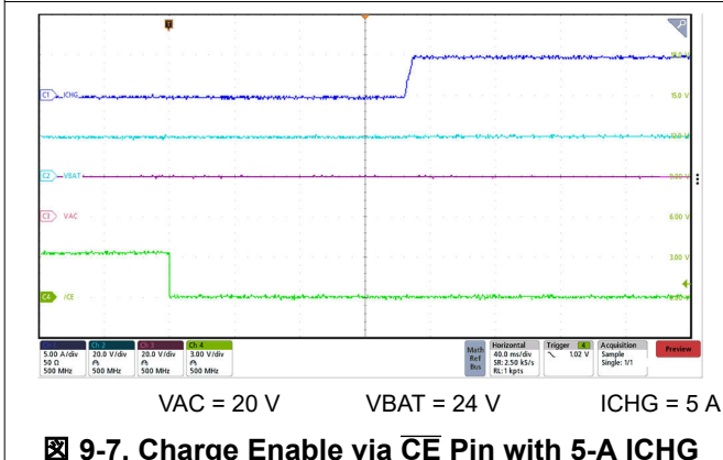
9-7. Charge Enable via \overline{\text{CE}} Pin with 5-A ICHG
