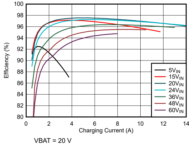
7-1. Charge Efficiency vs Charge Current (5s battery configuration)
