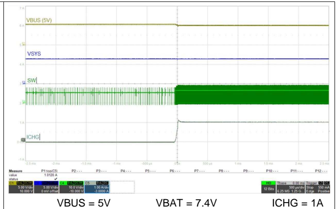
Figure 75. Charge Enable
