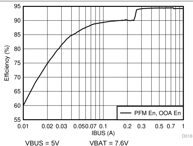
FIG 5. OTG Efficiency vs. VBUS Output Current
