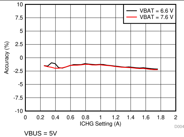
Figure 7. Charge Current Accuracy vs. ICHG Setting
