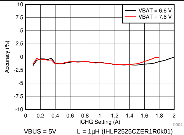
Figure 8. Charge Current Accuracy vs. ICHG Setting
