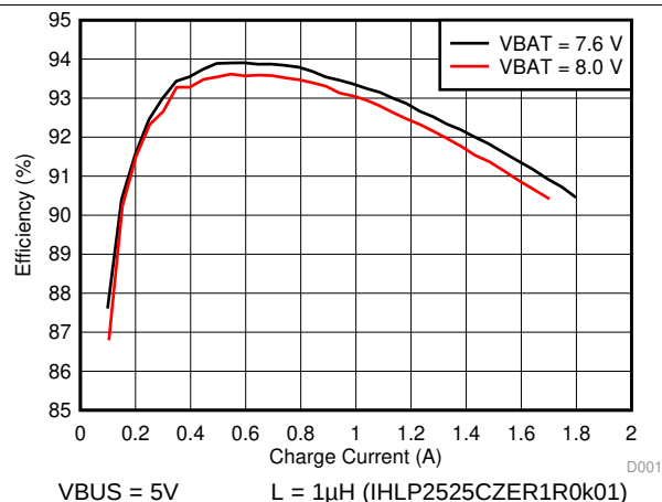
FIG 2. Charge Efficiency vs. Charge Current
