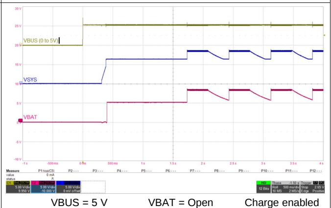
图 24. Adapter Plug-in with No Battery
