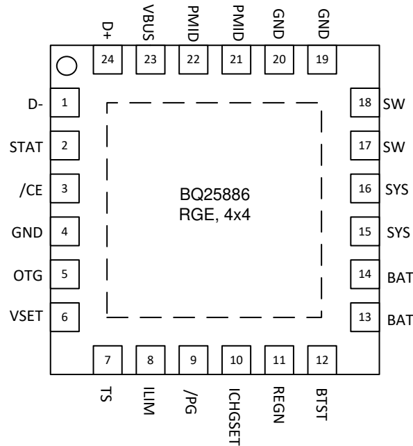
Pin Functions
