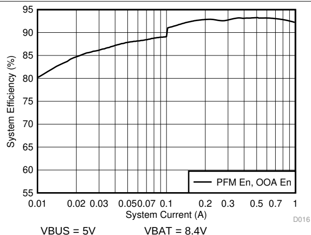
FIG 3. System Efficiency vs. System Current
