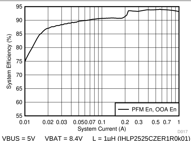
FIG 4. System Efficiency vs. System Current
