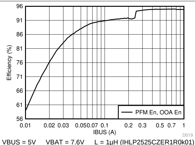
FIG 6. OTG Efficiency vs. VBUS Output Current
