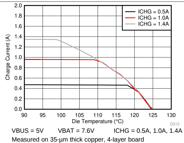
Figure 12. Max Current Temperature Profile
