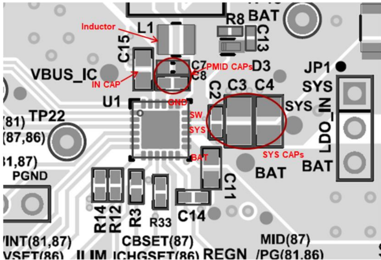
✎ 81. PCB Layout Example
