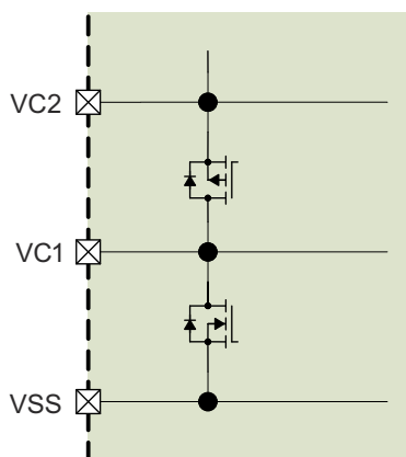
8-3. Internal Cell Balancing
