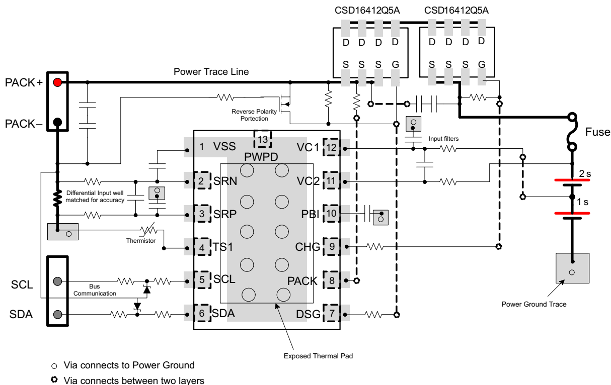
11-2. BQ28Z610-R1 Board Layout
