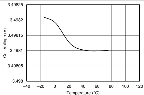
FIG 7-15. V_{CELL} Measurement at 3.5-V vs Temperature
