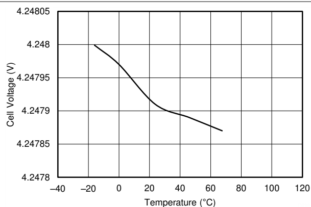
FIG 7-16. V_{CELL} Measurement at 4.25-V vs Temperature
