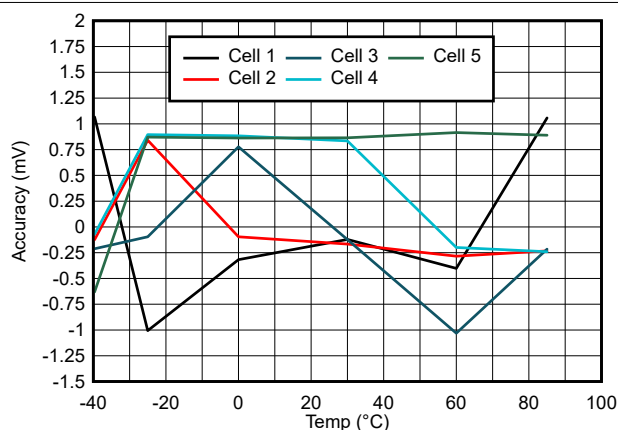
Figure 6-5. Cell Voltage Measurement Error vs Temperature with Cell Voltage = 2.5 V
