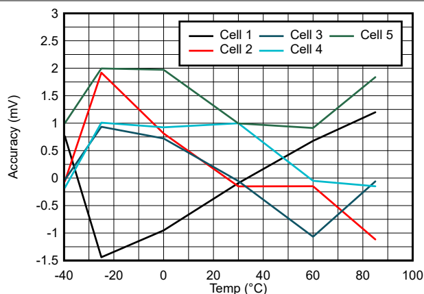
Figure 6-7. Cell Voltage Measurement Error vs Temperature with Cell Voltage = 4.5 V
