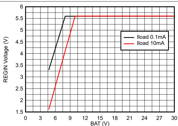
6-24. REGIN Voltage vs BAT Voltage
