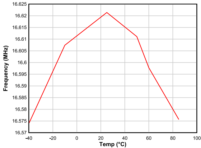
Figure 6-13. High Frequency Oscillator (HFO) Accuracy vs Temperature
