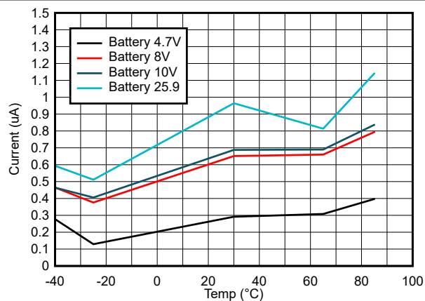
図 6-26. BAT Current in SHUTDOWN Mode vs Temperature
