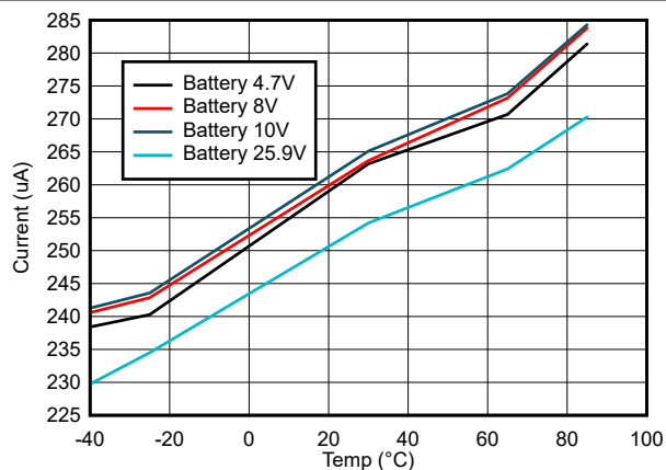
図 6-25. BAT Current in NORMAL Mode vs Temperature
