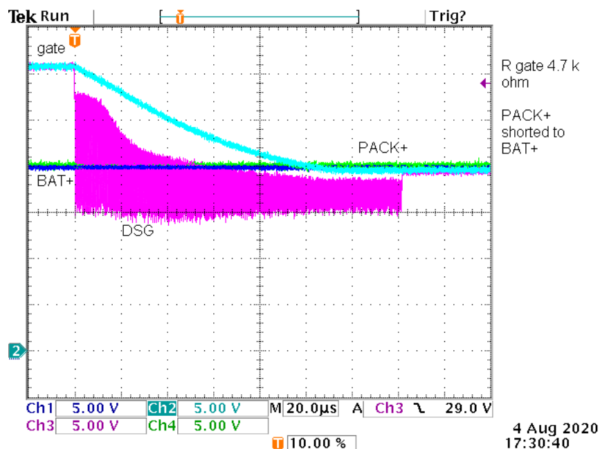
Figure 8-10. A Slower Turn-Off Case Using a 4.7-k \Omega Series Gate Resistor, and the PACK+ Connector Shorted to the Top of the Stack
