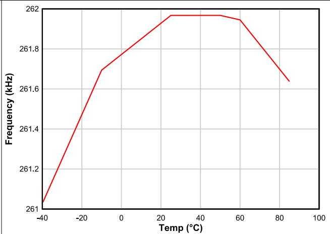
Figure 6-12. Low Frequency Oscillator (LFO) Accuracy vs Temperature
