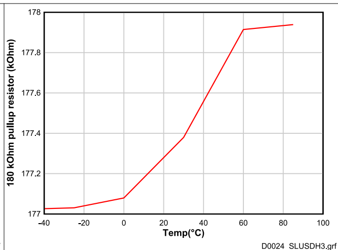
6-20. Thermistor Pullup Resistance vs Temperature (180-k \Omega Setting)
