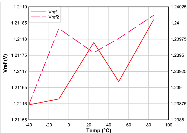
Figure 6-10. Internal Voltage References vs Temperature (VREF1 and VREF2)
