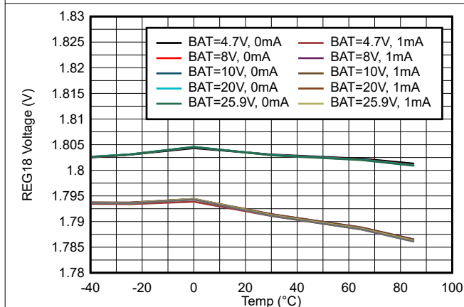
6-23. REG18 Voltage vs Temperature
