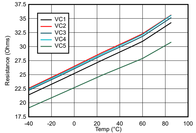
Figure 6-16. Cell Balancing Resistance vs Temperature
