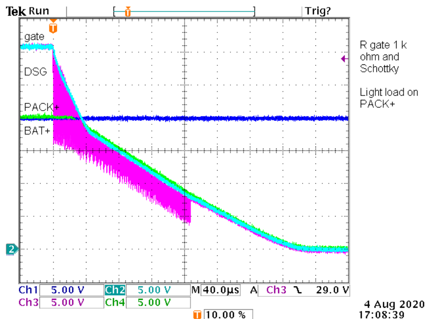
Figure 8-8. Moderate Speed DSG FET Turn-Off, Using a 1-k \Omega Series Gate Resistor, and a Light Load on PACK+.
