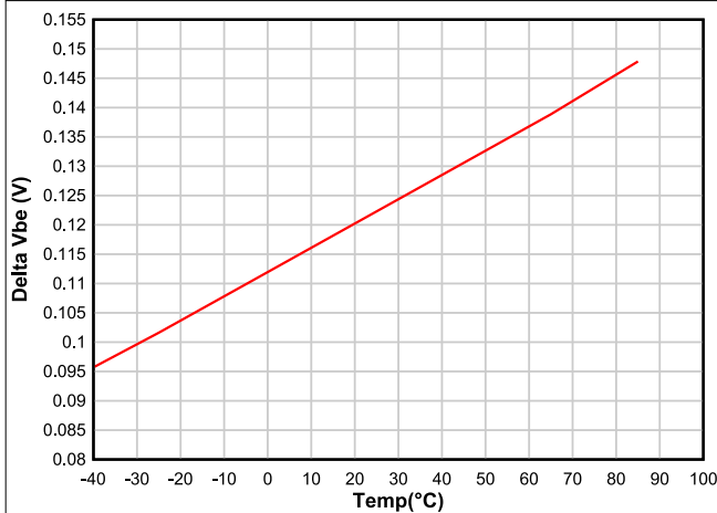
Figure 6-11. Internal Temperature Sensor (Delta V_{BE} ) Voltage vs Temperature
