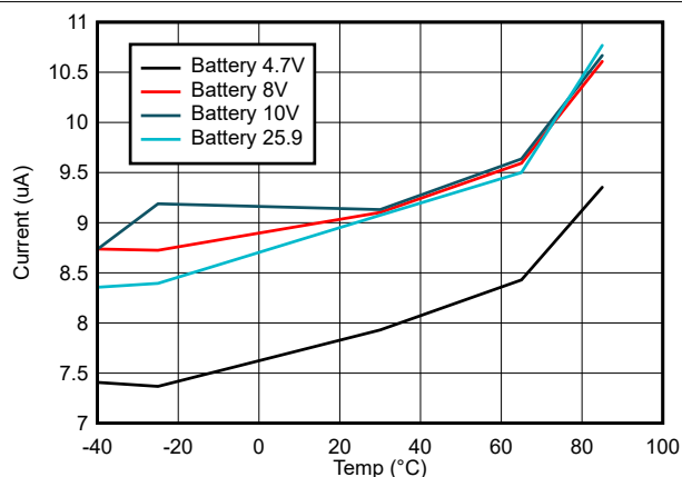
図 6-28. BAT Current in DEEPSLEEP2 (No LFO) Mode vs Temperature
