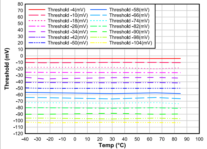
Figure 6-14. Overcurrent in Discharge Protection 1 (OCD1) Threshold vs Temperature
