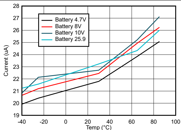
図 6-27. BAT Current in SLEEP2 (SRC Follower) Mode vs Temperature
