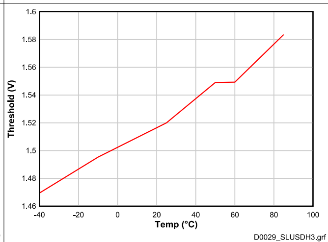
6-22. LD Wake Voltage vs Temperature
