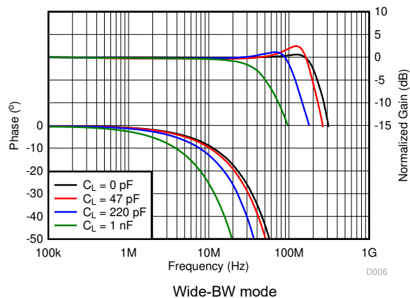
図 6-24. Gain and Phase vs Frequency and Load Capacitance
