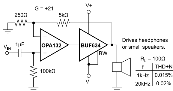
図 8-2. High Performance Headphone Driver
