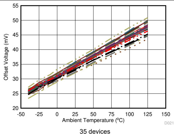
図 6-43. Offset Voltage vs Temperature
