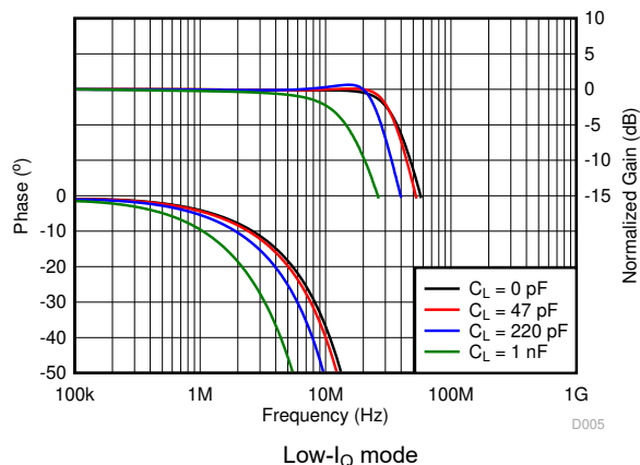
図 6-23. Gain and Phase vs Frequency and Load Capacitance
