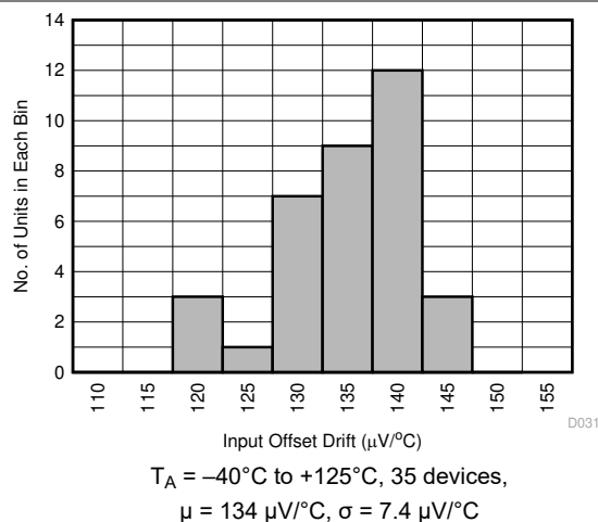
図 6-44. Offset Voltage Drift Distribution Histogram
