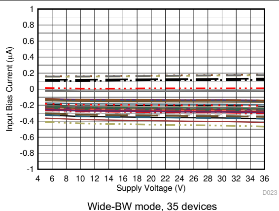
図 6-46. Input Bias Current vs Supply Voltage
