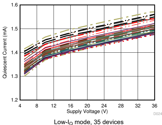
図 6-47. Quiescent Current vs Supply Voltage
