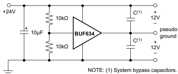
8-3. Pseudo-Ground Driver
