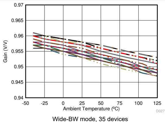
図 6-52. Buffer Gain vs Temperature
