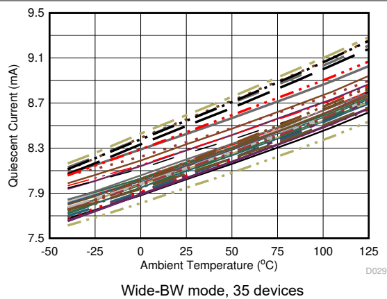
図 6-50. Quiescent Current vs Temperature
