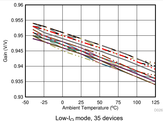
図 6-51. Buffer Gain vs Temperature
