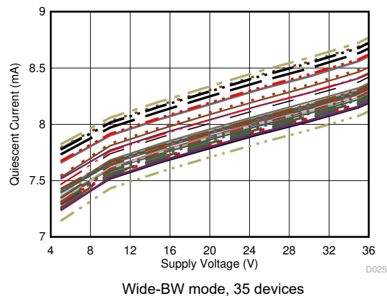
図 6-48. Quiescent Current vs Supply Voltage
