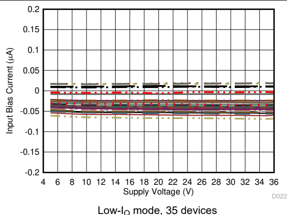
図 6-45. Input Bias Current vs Supply Voltage
