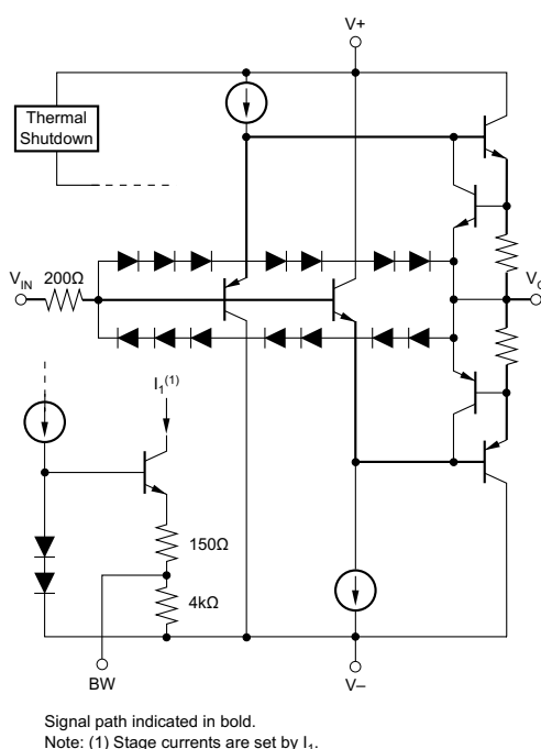
図 7-1. Internal Block Diagram: TO-220 and TO-263
