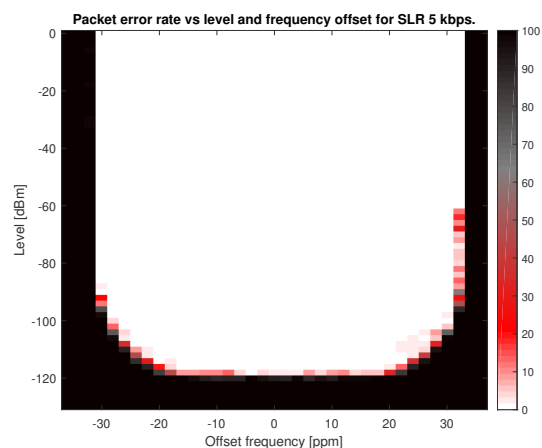
7-15. PER vs. Level vs. Frequency (SimpleLink™ Long Range 5 kbps, 868 MHz)
