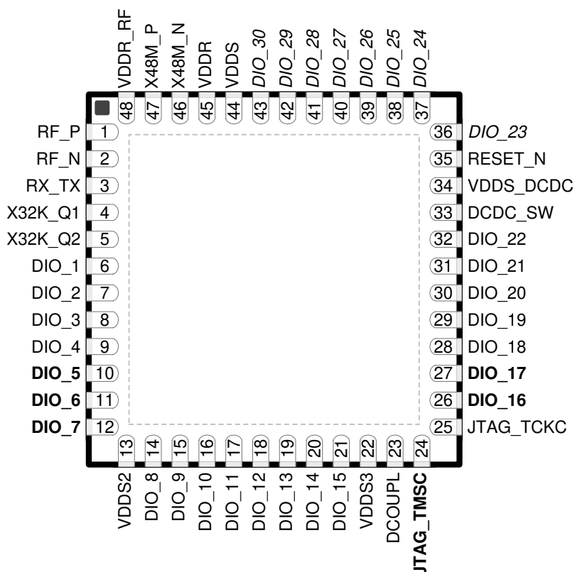
❏ 6-1. RGZ (7-mm x 7-mm) Pinout, 0.5-mm Pitch (Top View)
