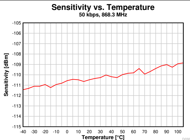
7-12. Sensitivity vs. Temperature (50 kbps, 868.3 MHz)
