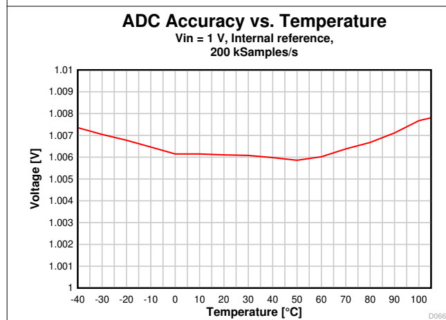
7-26. ADC Accuracy vs. Temperature
