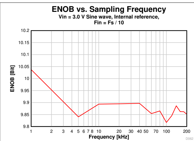
7-23. ENOB vs. Sampling Frequency
