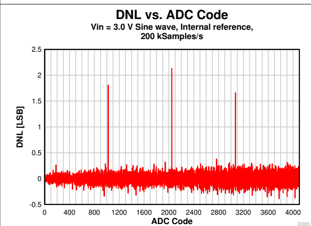
7-25. DNL vs. ADC Code
