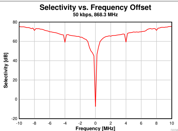
7-14. Selectivity vs. Frequency Offset (50 kbps, 868.3 MHz)
