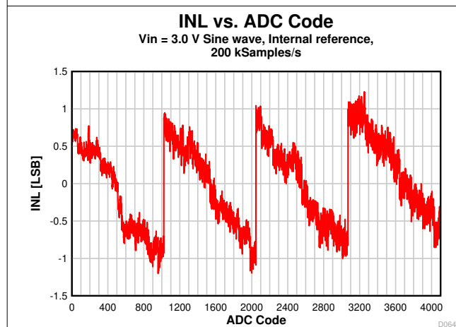
7-24. INL vs. ADC Code
