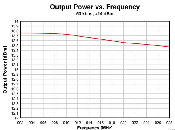
7-21. Output Power vs. Frequency (50 kbps, 915 MHz)
