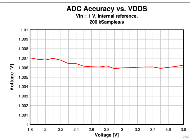
7-27. ADC Accuracy vs. Supply Voltage (VDD)
