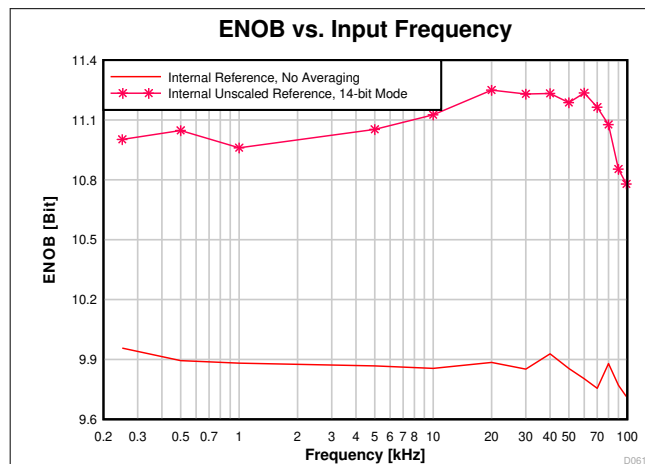
7-22. ENOB vs. Input Frequency
