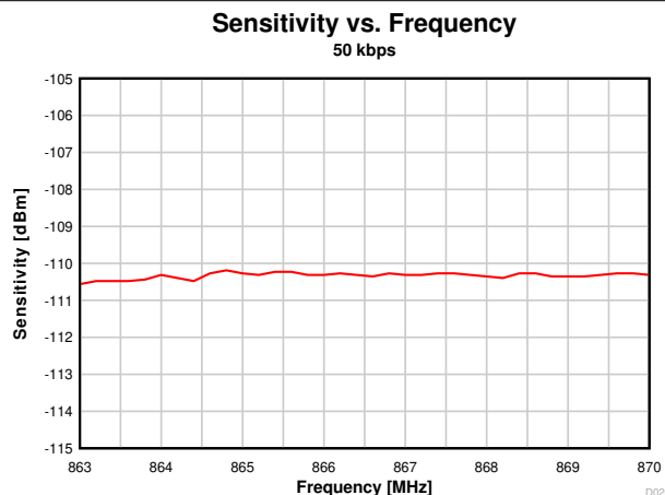
7-10. Sensitivity vs. Frequency (50 kbps, 868 MHz)
