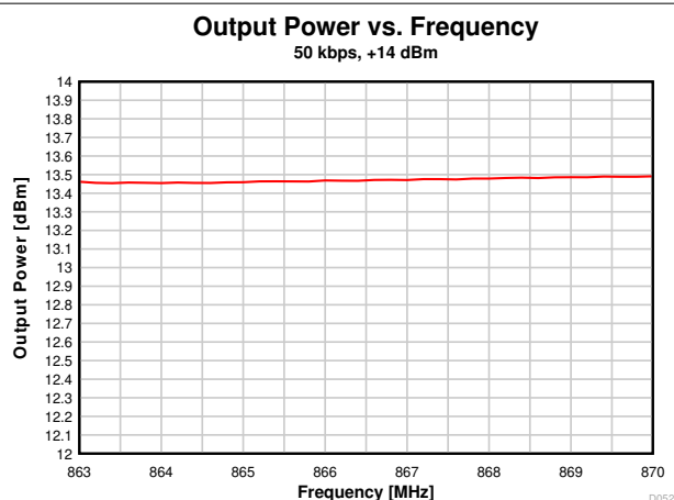
7-20. Output Power vs. Frequency (50 kbps, 868 MHz)
