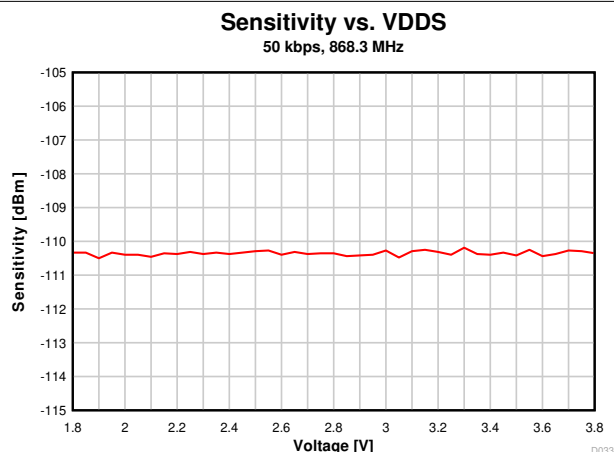
7-13. Sensitivity vs. Supply Voltage (VDD) (50 kbps, 868.3 MHz)
