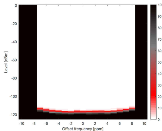
Figure 7-17. Narrowband, 9.6 kbps \pm 2.4 kHz deviation, 2-GFSK, 868 MHz, 17.1 kHz RX Bandwidth
